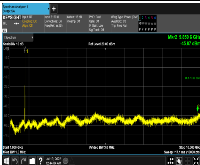
Band66-5MHz-16QAM-131997-1RB#0-Range5:1000~10000MHz
