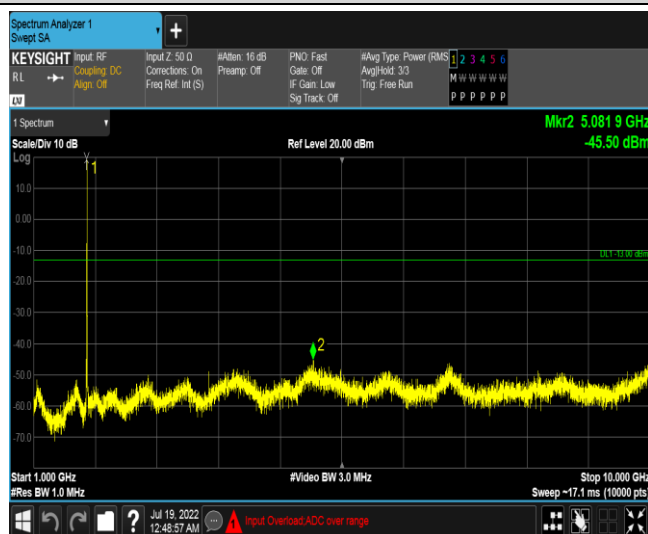
Band66-5MHz-16QAM-132647-1RB#0-Range5:1000~10000MHz
