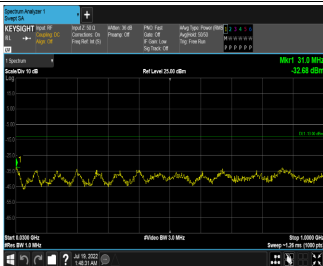
Band66-15MHz-QPSK-132322-1RB#0-Range4:30~1000MHz
