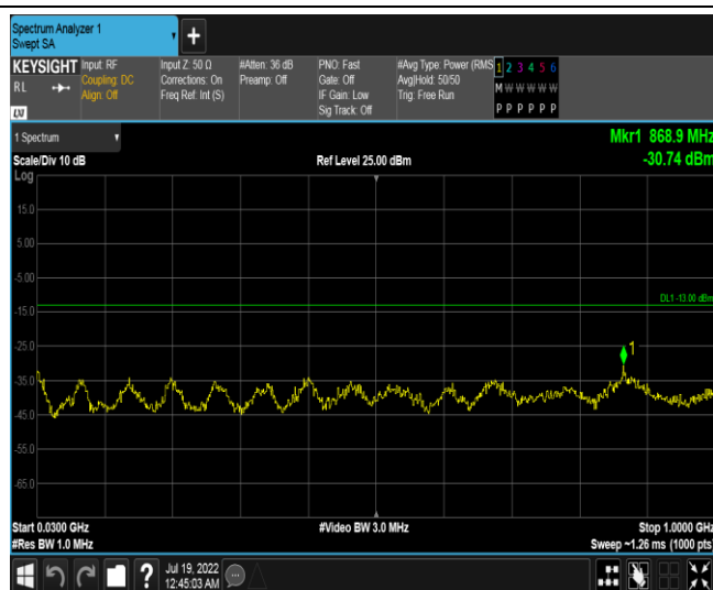
Band66-5MHz-QPSK-132322-1RB#0-Range1:30~1000MHz
