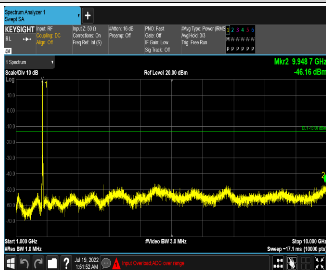
Band66-15MHz-QPSK-132597-1RB#0-Range5:1000~10000MHz
