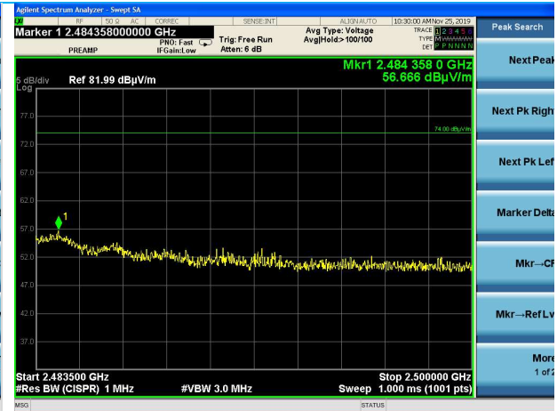
2483.5-2500 MHz, Horizontal Antenna, Flat EUT Channel 25
