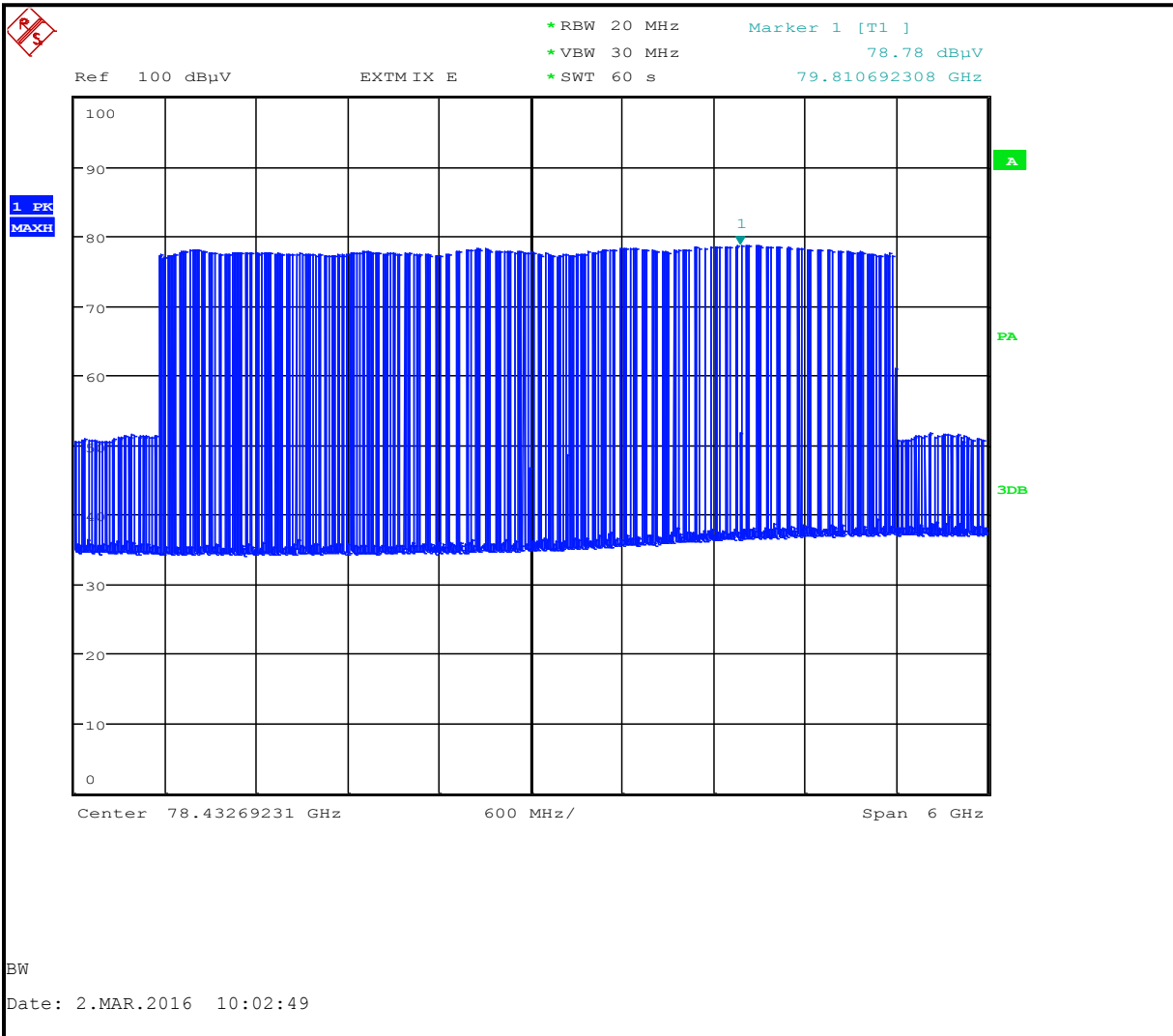
Plot 4-1: Radiated Fundamental (EIRP in 20 MHz, Peak Detector)
