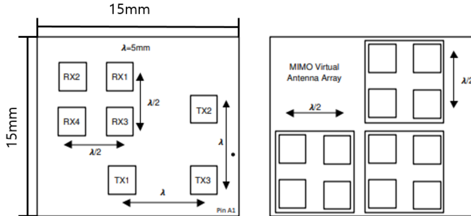
Figure 1. Antenna Positions (Placement and Relative Spacing)
