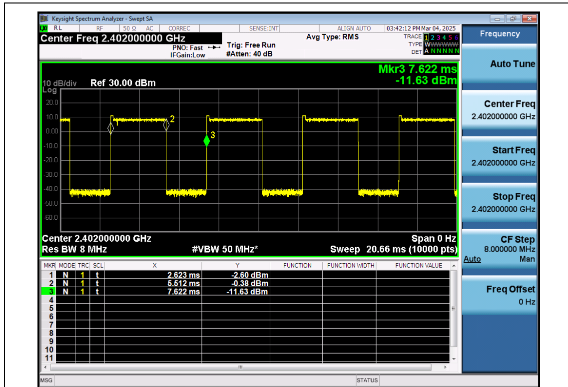
EDR--8DPSK-ANT1-2402
