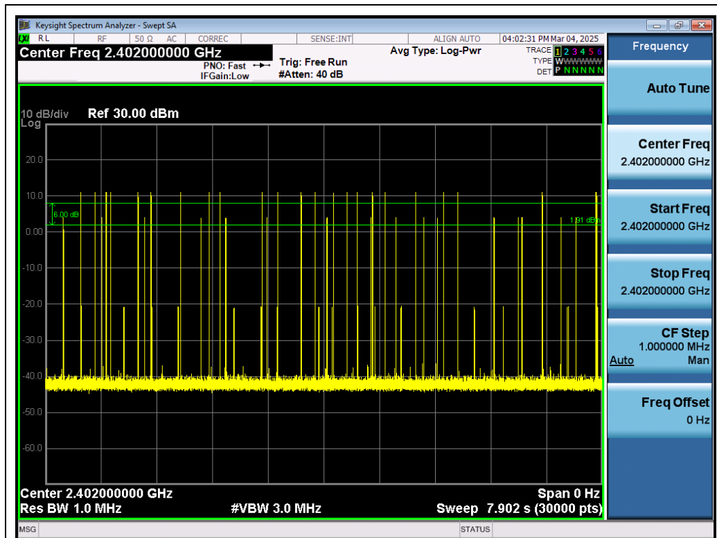
Test_Graph_EDR_HOP_ANT1_NA_2Mbps_2402_Number of Busrt
