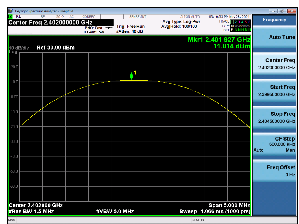
Test_Graph_BR_ANT1_2402_1Mbps_Peak Power
