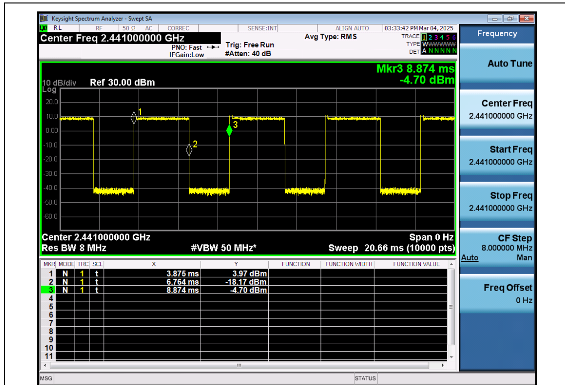
EDR- \pi /4-DQPSK-ANT1-2441
