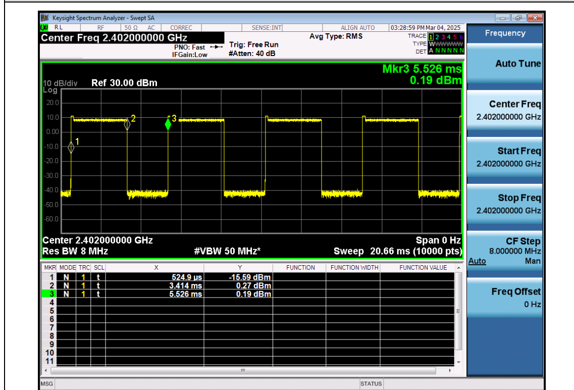
EDR-π /4-DQPSK-ANT1-2402
