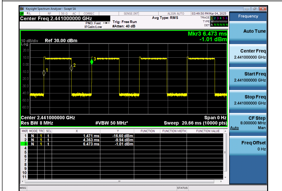
EDR-8DPSK-ANT1-2441
