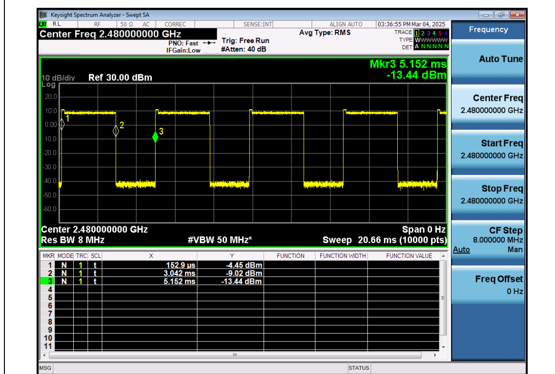
EDR- \pi /4-DQPSK-ANT1-2480
