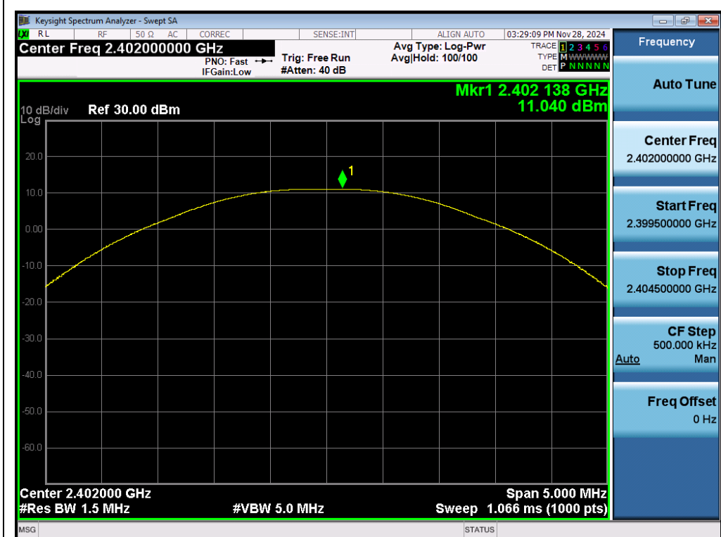
Test_Graph_EDR_ANT1_2402_2Mbps_Peak Power
