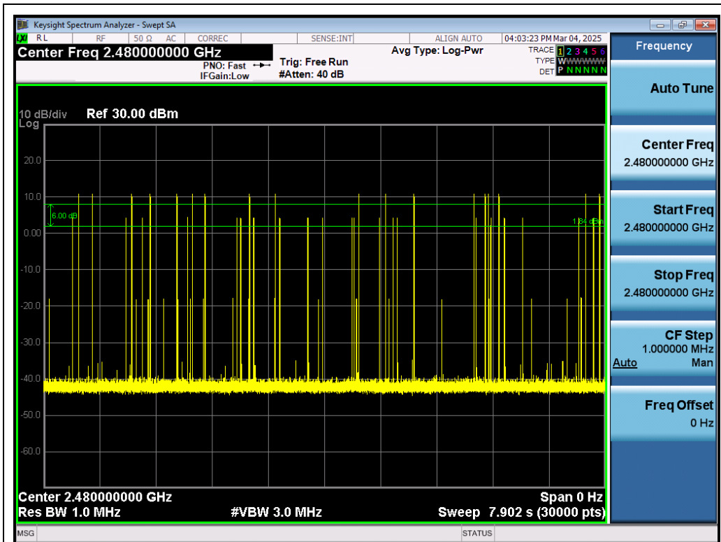
Test_Graph_EDR_HOP_ANT1_NA_2Mbps_2480_Number of Burst
