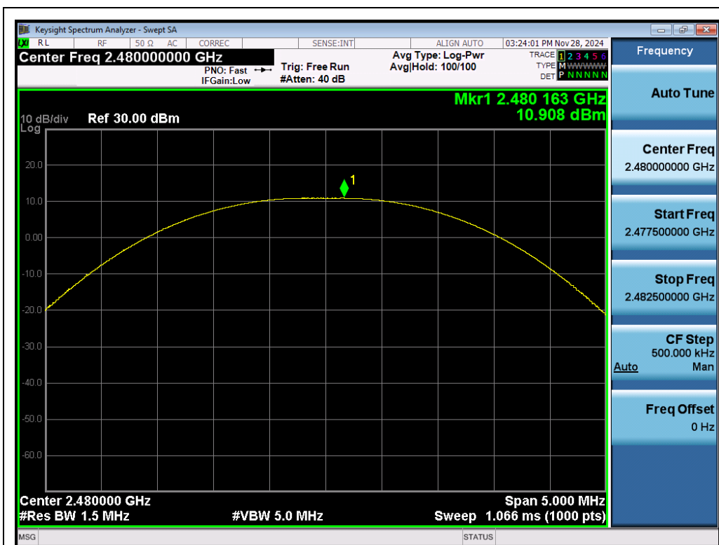
Test_Graph_BR_ANT1_2480_1Mbps_Peak Power
