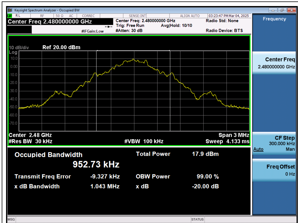
Test_Graph_BR_ANT1_2480_1Mbps_OBW
