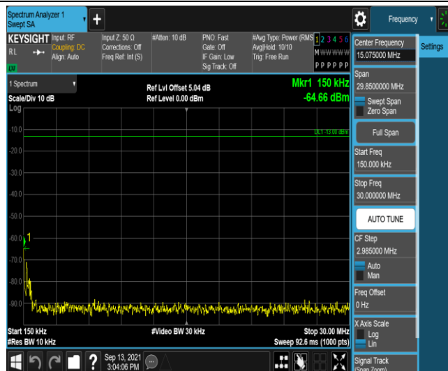
Band26-10MHz-16QAM-26990-1RB#0-Range2:0.15~30MHz
