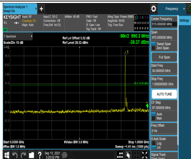
Band26-15MHz-QPSK-26965-1RB#0-Range3:30~1000MHz
