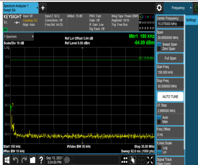
Band26-15MHz-QPSK-26965-1RB#0-Range2:0.15~30MHz
