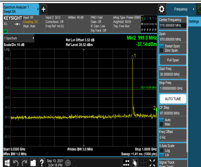
Band26-10MHz-16QAM-26990-1RB#0-Range3:30~1000MHz
