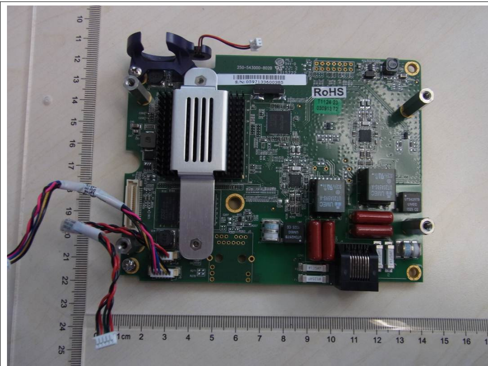
Figure 30: PCB with DSL connector CSC-TPSVW-CU, CSC-TPSVW
