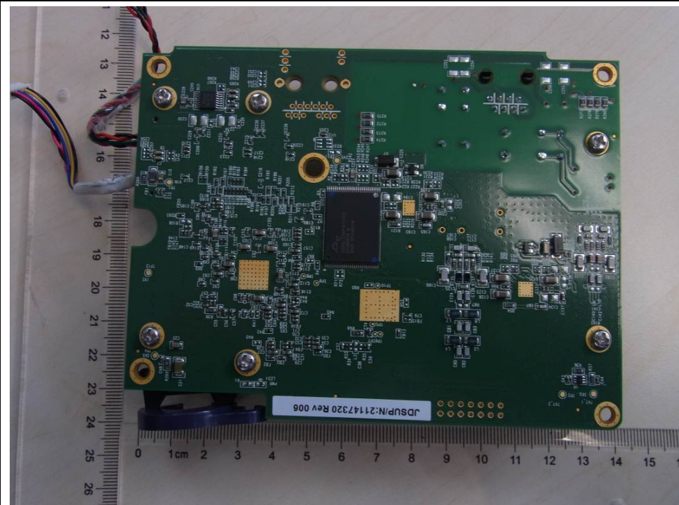
Figure 31: PCB with DSL connector CSC-TPSVW-CU, CSC-TPSVW
