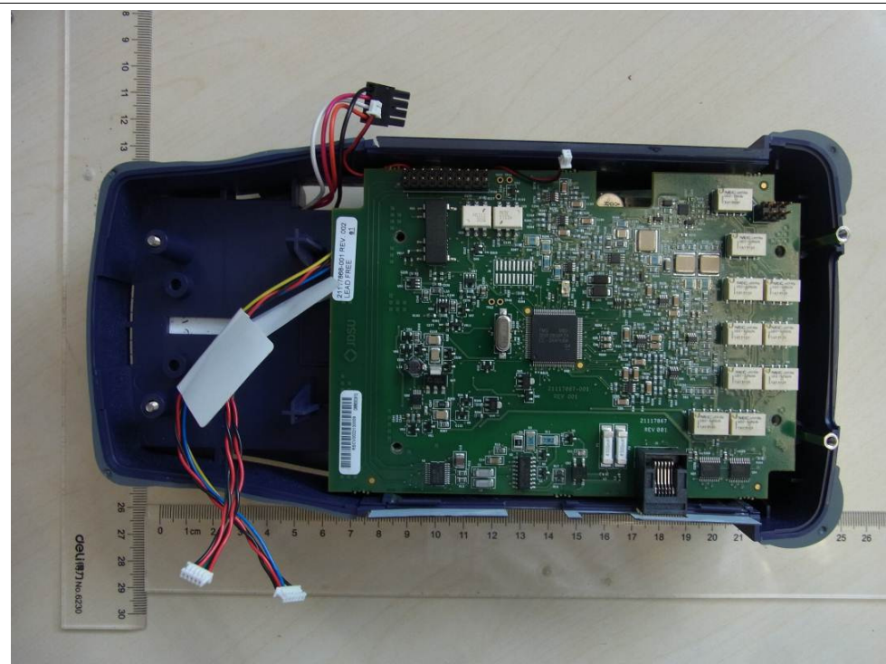
Figure 18: Internal view bottom enclosure CSC-TPSVW-CU, SCTPS-AB-CU
