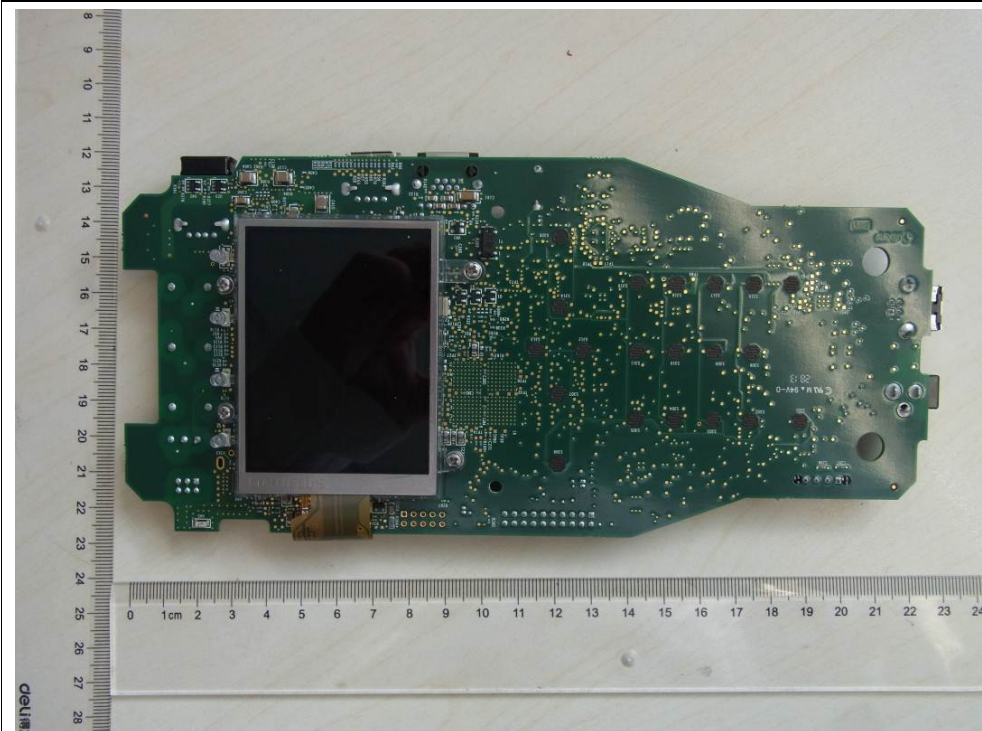
Figure 21: Main PCB
