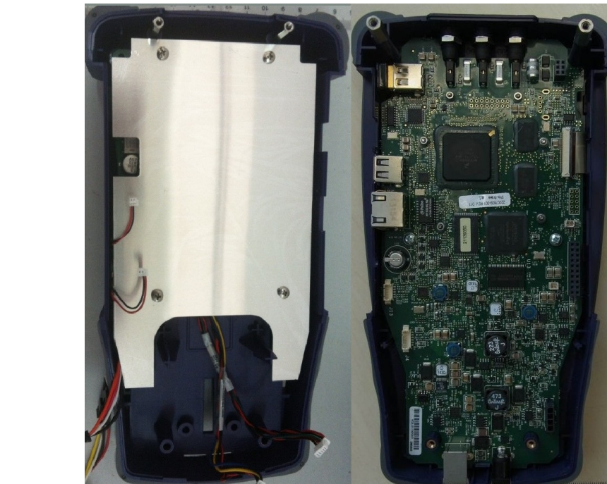
Figure 15: Internal view CSC-TPSVW, SCTPS-AB
