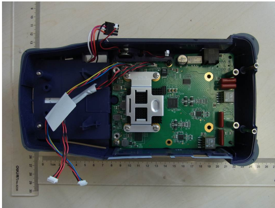
Figure 25: Internal view of bottom enclosure SCTPS-AB-CU, SCTPS-AB
