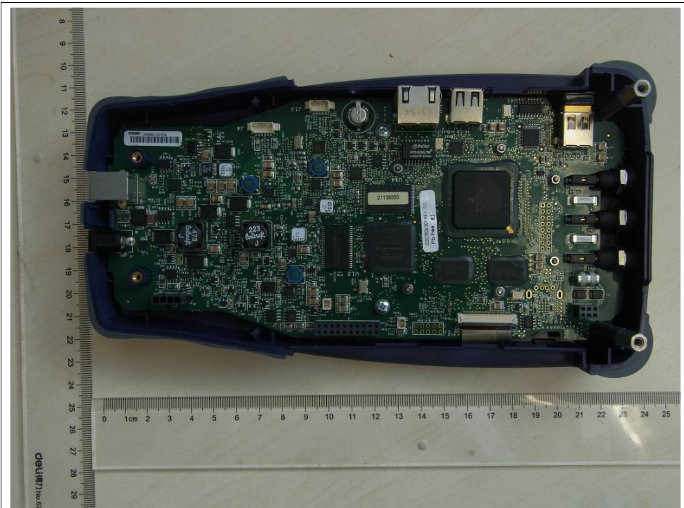
Figure 16: Internal view
