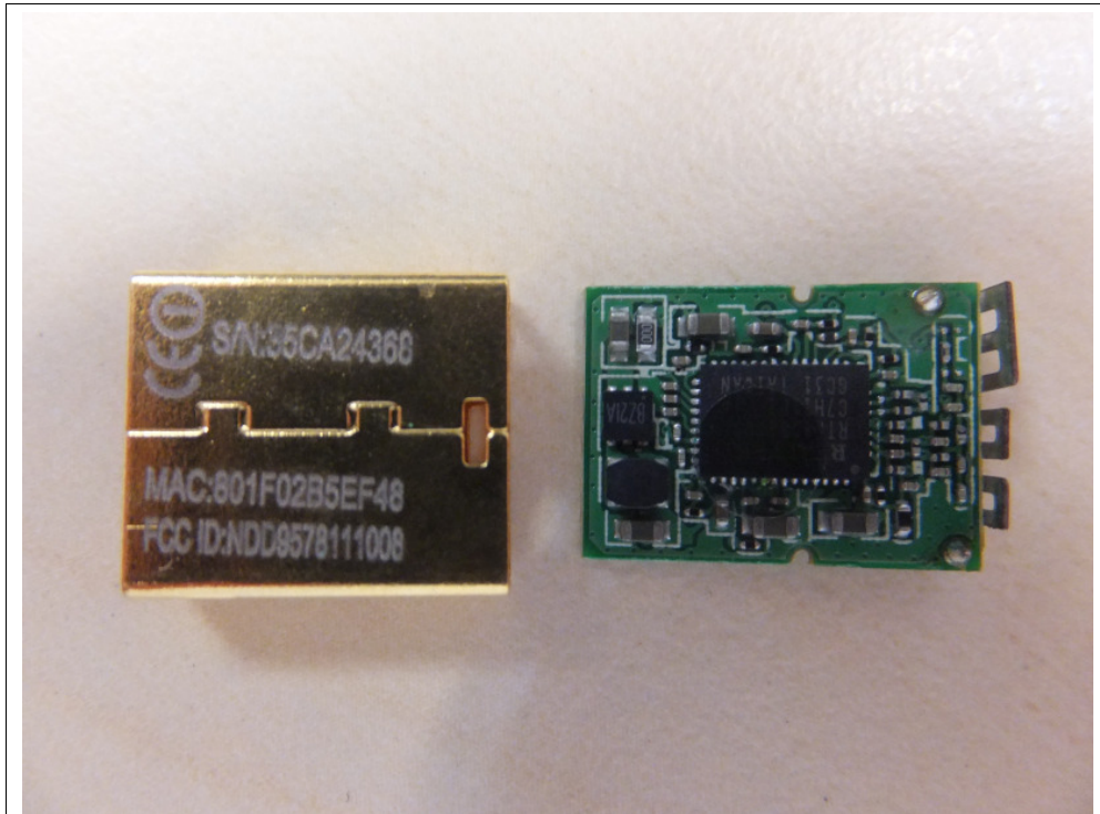
Figure 36: Wi-Fi USB dongle internal view 2
