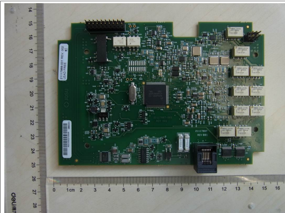
Figure 22: PCB with POTS connector CSC-TPSVW-CU, SCTPS-AB-CU
