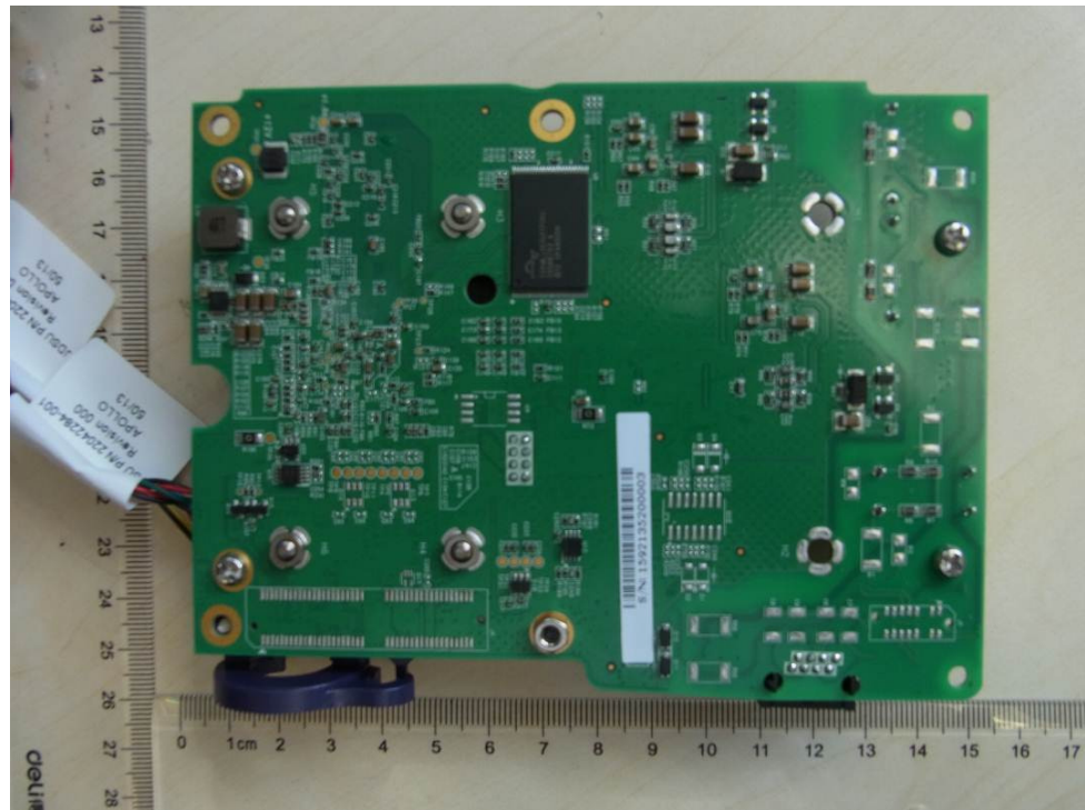
Figure 29: PCB with DSL connector SCTPS-AB-CU, SCTPS-AB
