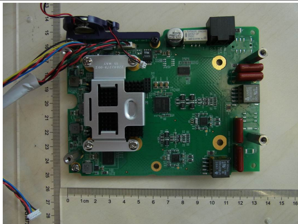
Figure 28: PCB with DSL connector SCTPS-AB-CU, SCTPS-AB
