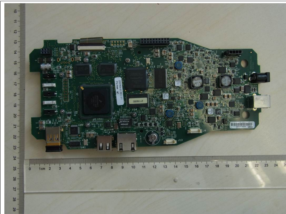
Figure 20: Main PCB
