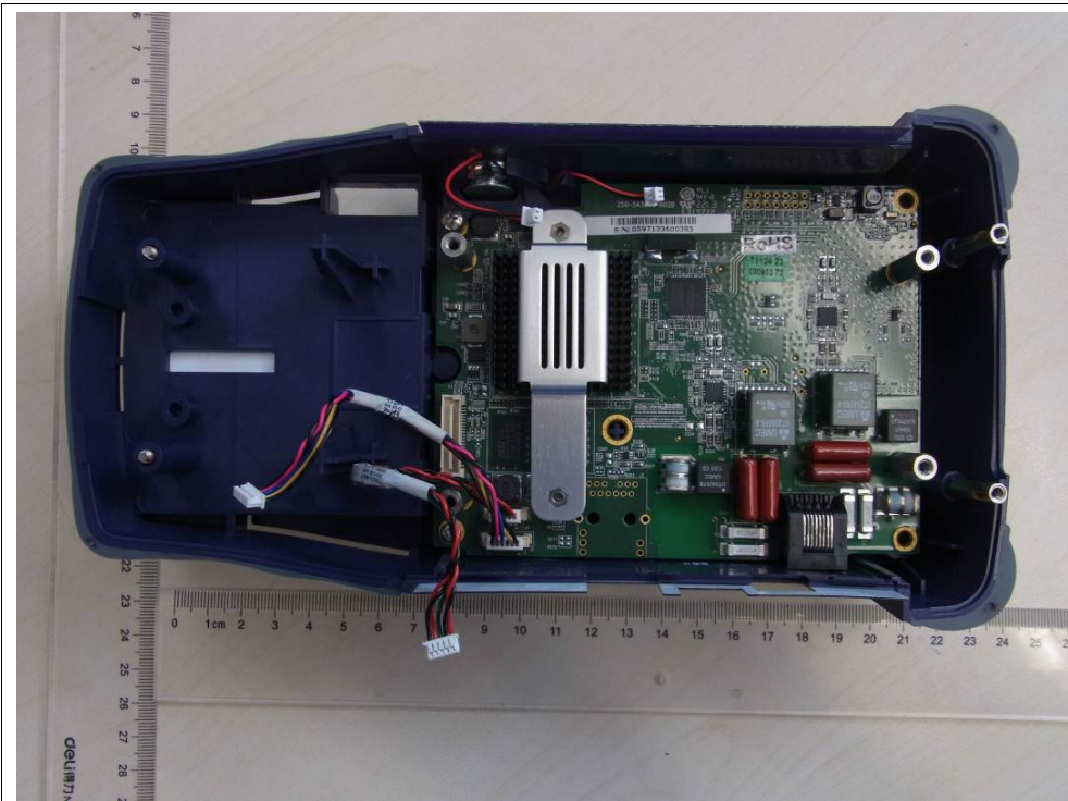
Figure 26: Internal view of bottom enclosure CSC-TPSVW-CU, CSC-TPSVW
