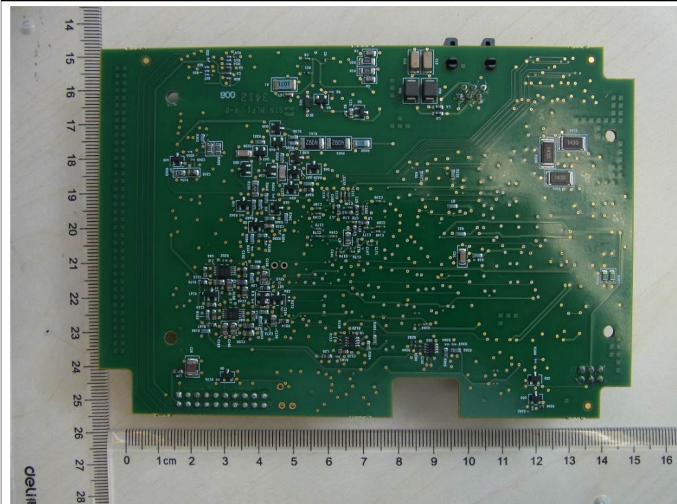
Figure 23 PCB with POTS connector CSC-TPSVW-CU, SCTPS-AB-CU
