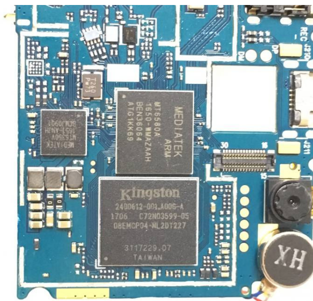
EUT – Main IC View
