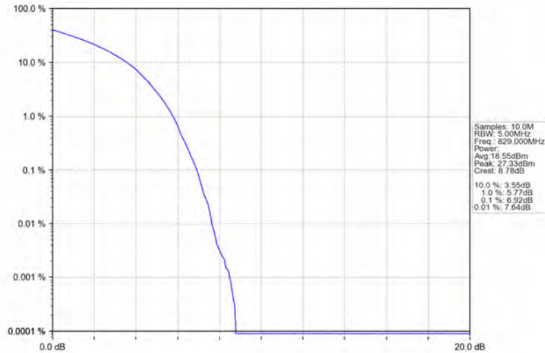
Band26b_10MHz_64QAM_LCH_829MHz_RB_50_0_NTNV
