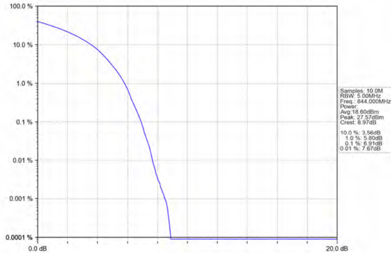
Band26b_10MHz_64QAM_HCH_844MHz_RB_50_0_NTNV
