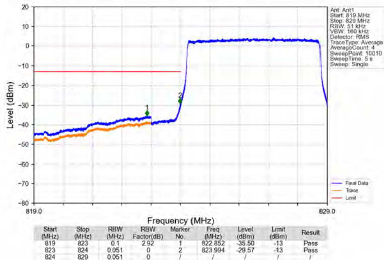
Band26b_5MHz_16QAM_LCH_826.5MHz_RB_25_0_NTNV
