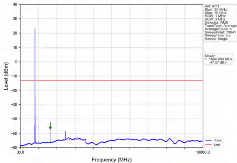
Band26b_10MHz_16QAM_HCH_844MHz_RB_1_0_NTNV
