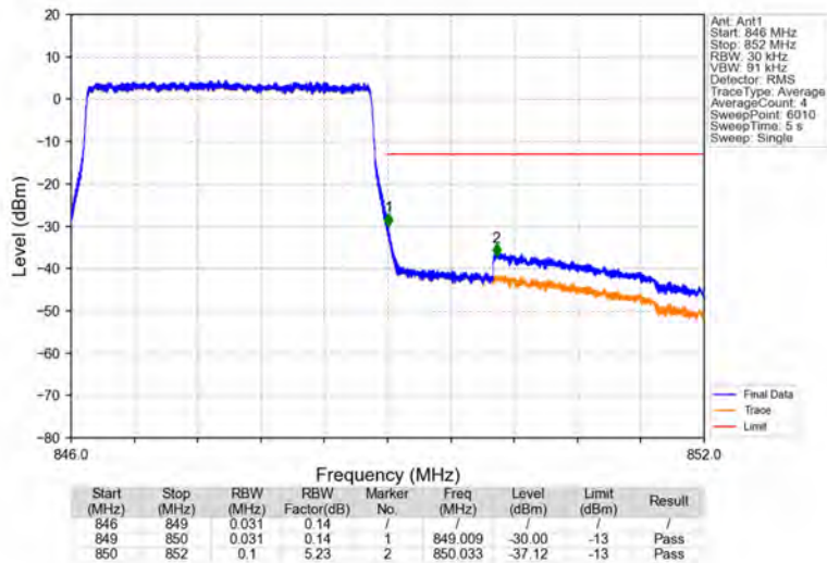
Band26b_3MHz_16QAM_HCH_847.5MHz_RB_15_0_NTNV
