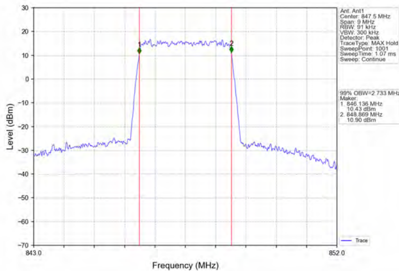
Band26b_3MHz_64QAM_HCH_847.5MHz_RB_15_0_NTNV
