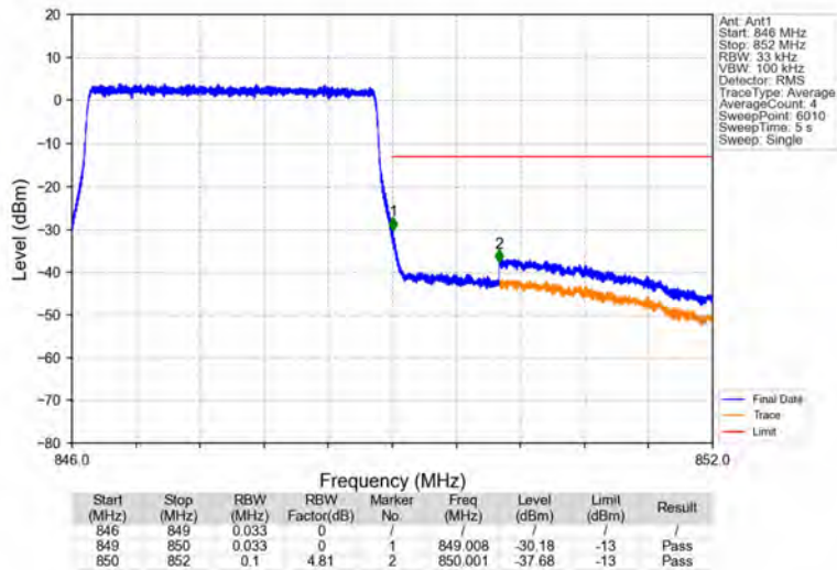
Band26b_3MHz_64QAM_HCH_847.5MHz_RB_15_0_NTNV
