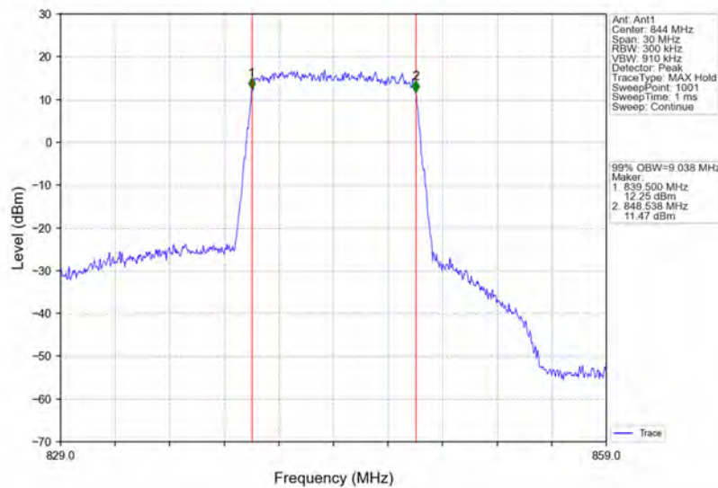
Band26b_10MHz_64QAM_HCH_844MHz_RB_50_0_NTNV
