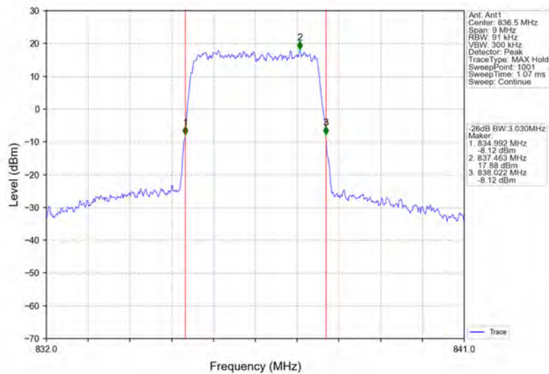
Band26b_3MHz_16QAM_MCH_836.5MHz_RB_15_0_NTNV
