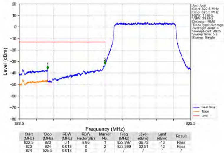
Band26b_1.4MHz_16QAM_LCH_824.7MHz_RB_6_0_NTNV
