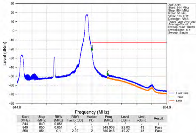
Band26b_5MHz_16QAM_HCH_846.5MHz_RB_1_24_NTNV
