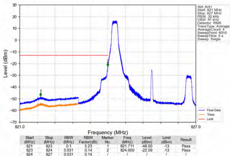
Band26b_3MHz_16QAM_LCH_825.5MHz_RB_1_0_NTNV
