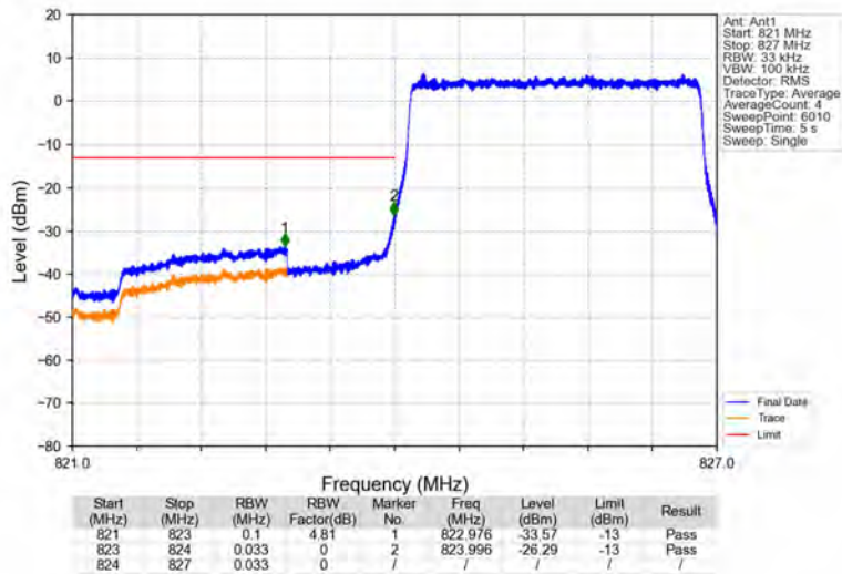
Band26b_3MHz_QPSK_LCH_825.5MHz_RB_15_0_NTNV
