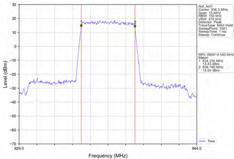
Band26b_5MHz_QPSK_MCH_836.5MHz_RB_25_0_NTNV
