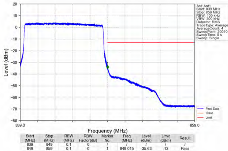
Band26b_10MHz_16QAM_HCH_844MHz_RB_50_0_NTNV
