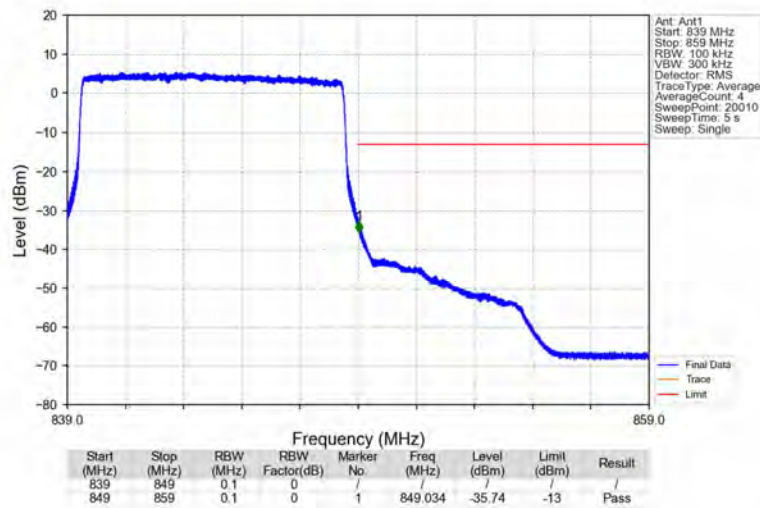
Band26b_10MHz_QPSK_HCH_844MHz_RB_50_0_NTNV
