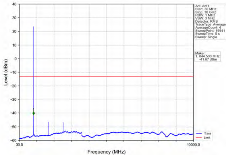
Band26b_1.4MHz_QPSK_HCH_848.3MHz_RB_1_5_NTNV
