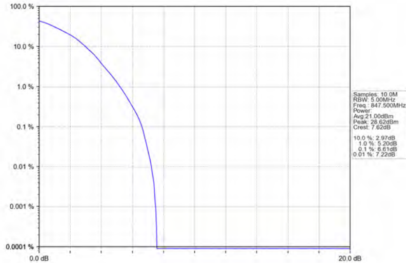
Band26b_3MHz_64QAM_HCH_847.5MHz_RB_15_0_NTNV
