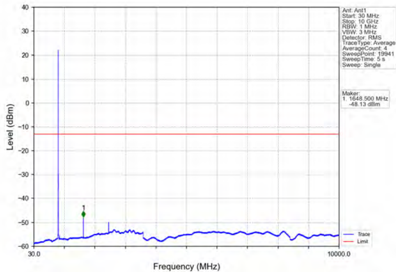
Band26b_3MHz_16QAM_LCH_825.5MHz_RB_15_0_NTNV
