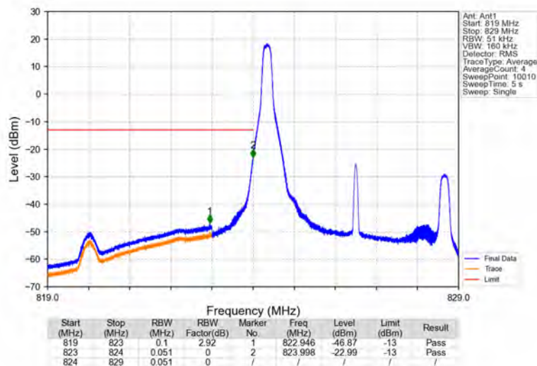
Band26b_5MHz_16QAM_LCH_826.5MHz_RB_1_0_NTNV
