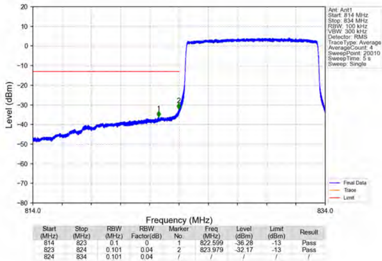
Band26b_10MHz_16QAM_LCH_829MHz_RB_50_0_NTNV
