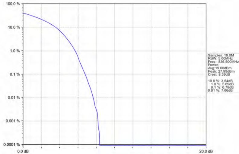
Band26b_10MHz_16QAM_MCH_836.5MHz_RB_50_0_NTNV
