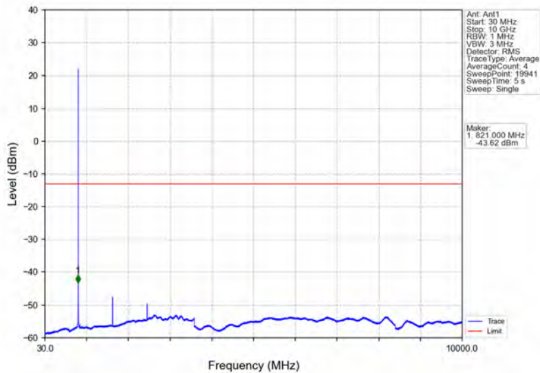
Band26b_1.4MHz_16QAM_LCH_824.7MHz_RB_6_0_NTNV
