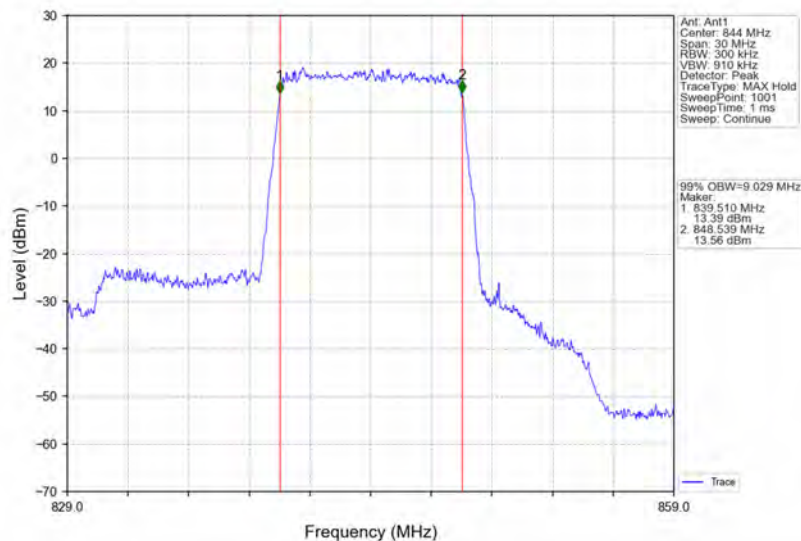
Band26b_10MHz_QPSK_HCH_844MHz_RB_50_0_NTNV
