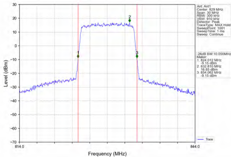
Band26b_10MHz_64QAM_LCH_829MHz_RB_50_0_NTNV
