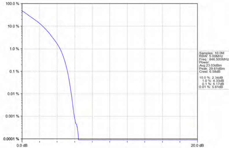
Band26b_5MHz_QPSK_HCH_846.5MHz_RB_25_0_NTNV
