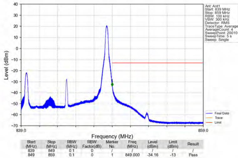
Band26b_10MHz_16QAM_HCH_844MHz_RB_1_49_NTNV
