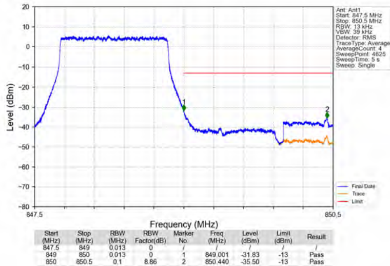
Band26b_1.4MHz_QPSK_HCH_848.3MHz_RB_6_0_NTNV
