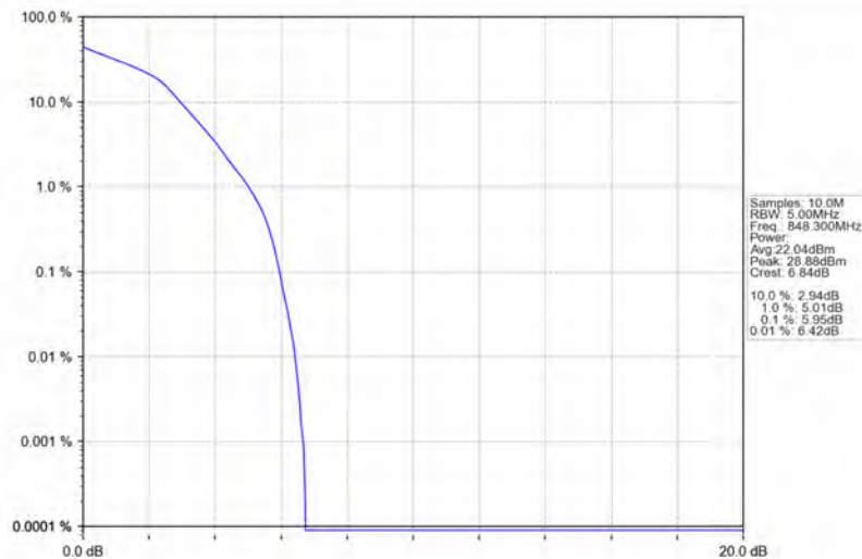
Band26b_1.4MHz_16QAM_HCH_848.3MHz_RB_6_0_NTNV
