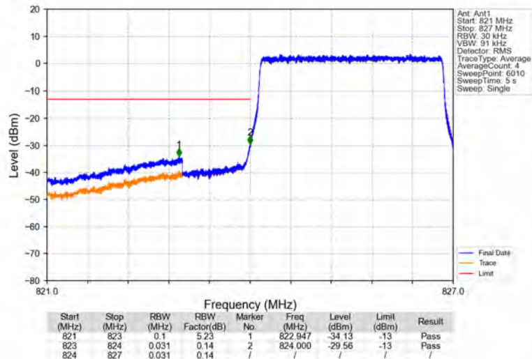
Band26b_3MHz_64QAM_LCH_825.5MHz_RB_15_0_NTNV
