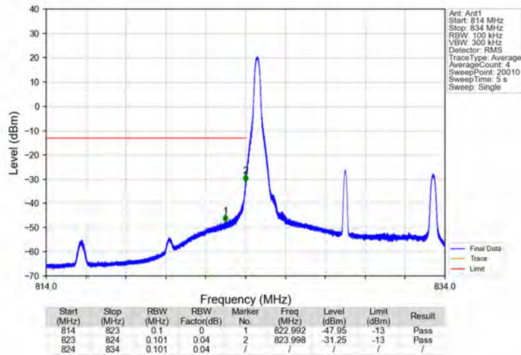
Band26b_10MHz_64QAM_LCH_829MHz_RB_1_0_NTNV
