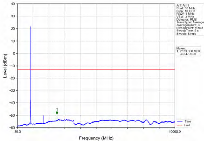
Band26b_5MHz_64QAM_HCH_846.5MHz_RB_1_24_NTNV
