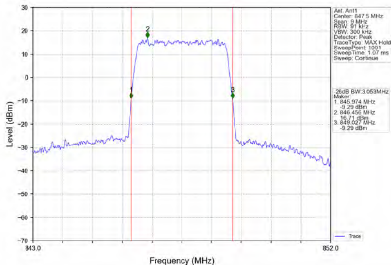
Band26b_3MHz_64QAM_HCH_847.5MHz_RB_15_0_NTNV
