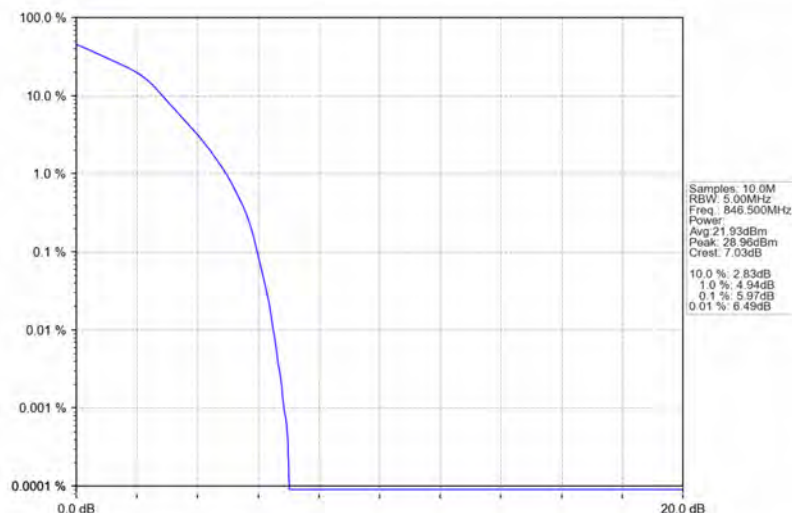
Band26b_5MHz_16QAM_HCH_846.5MHz_RB_25_0_NTNV
