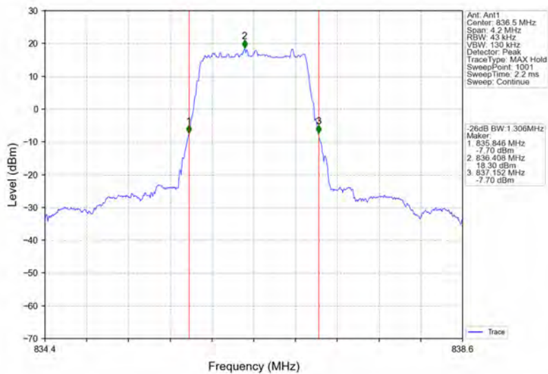
Band26b_1.4MHz_64QAM_MCH_836.5MHz_RB_6_0_NTNV
