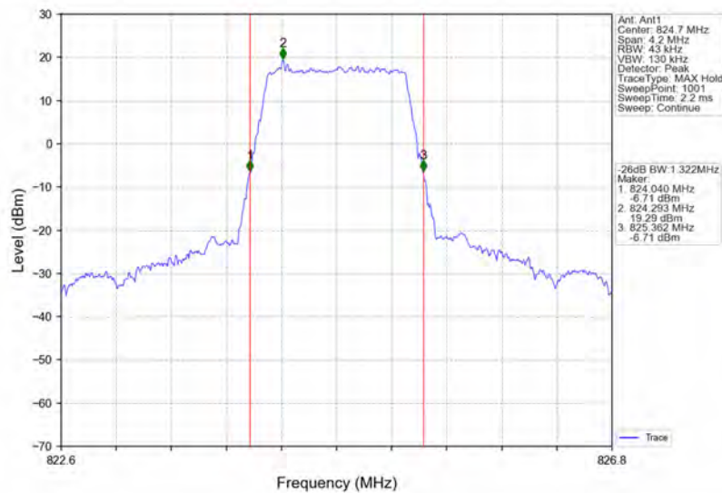
Band26b_1.4MHz_16QAM_LCH_824.7MHz_RB_6_0_NTNV
