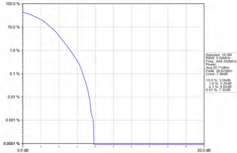
Band26b_1.4MHz_64QAM_HCH_848.3MHz_RB_6_0_NTNV
