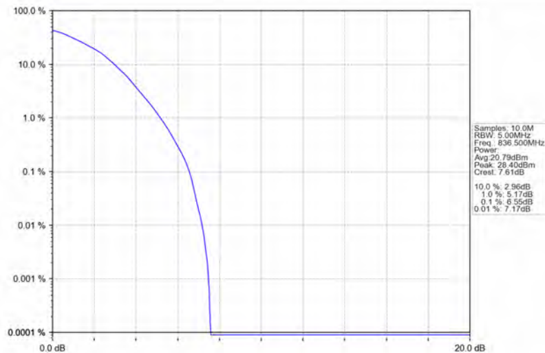
Band26b_3MHz_64QAM_MCH_836.5MHz_RB_15_0_NTNV
