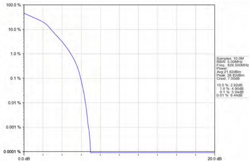
Band26b_5MHz_16QAM_LCH_826.5MHz_RB_25_0_NTNV
