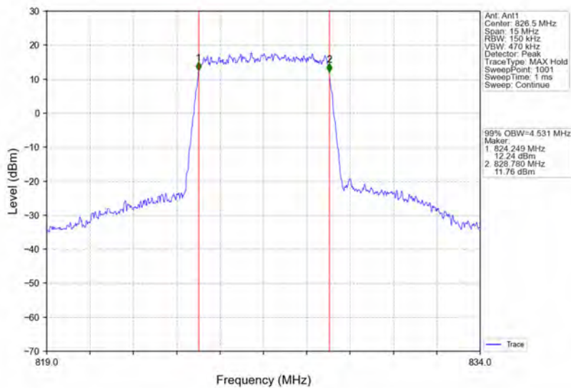
Band26b_5MHz_16QAM_LCH_826.5MHz_RB_25_0_NTNV
