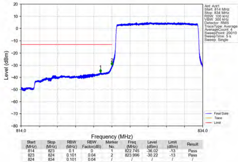
Band26b_10MHz_QPSK_LCH_829MHz_RB_50_0_NTNV
