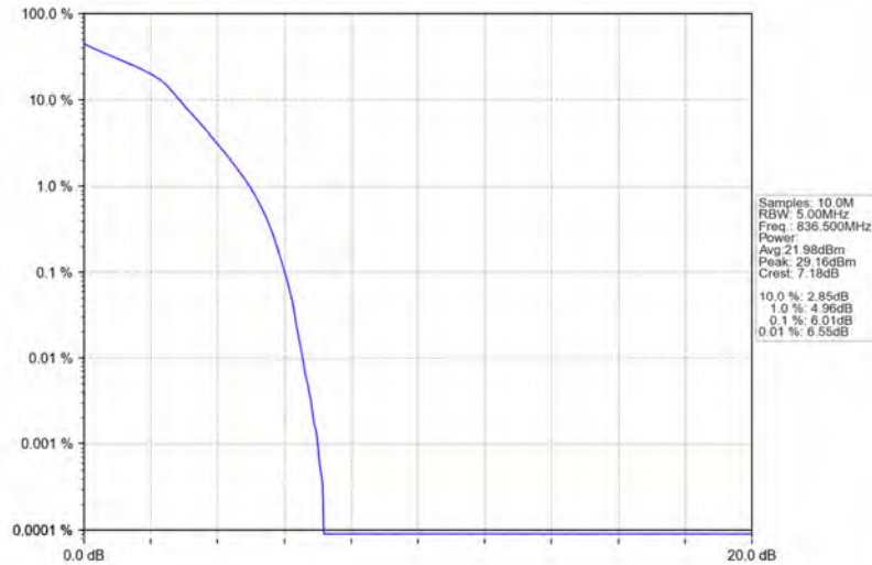
Band26b_3MHz_16QAM_MCH_836.5MHz_RB_15_0_NTNV
