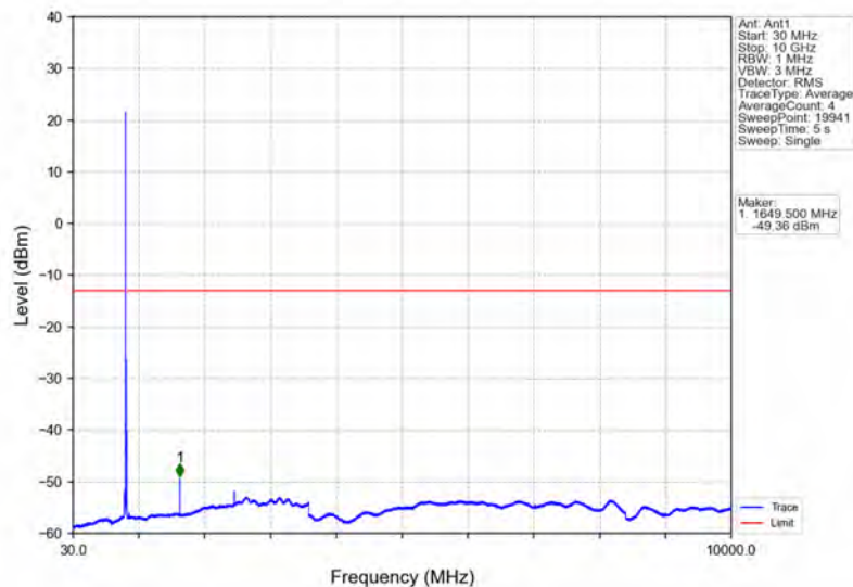
Band26b_10MHz_64QAM_LCH_829MHz_RB_1_0_NTNV
