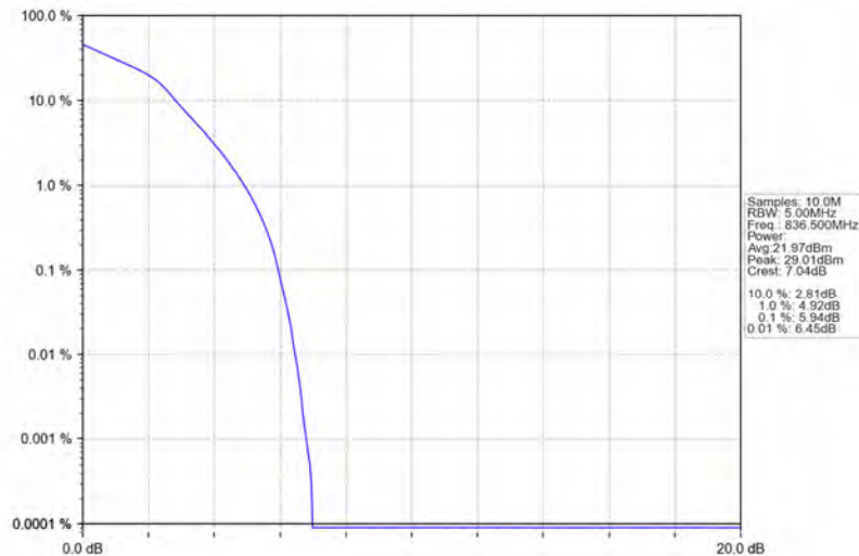
Band26b_5MHz_16QAM_MCH_836.5MHz_RB_25_0_NTNV
