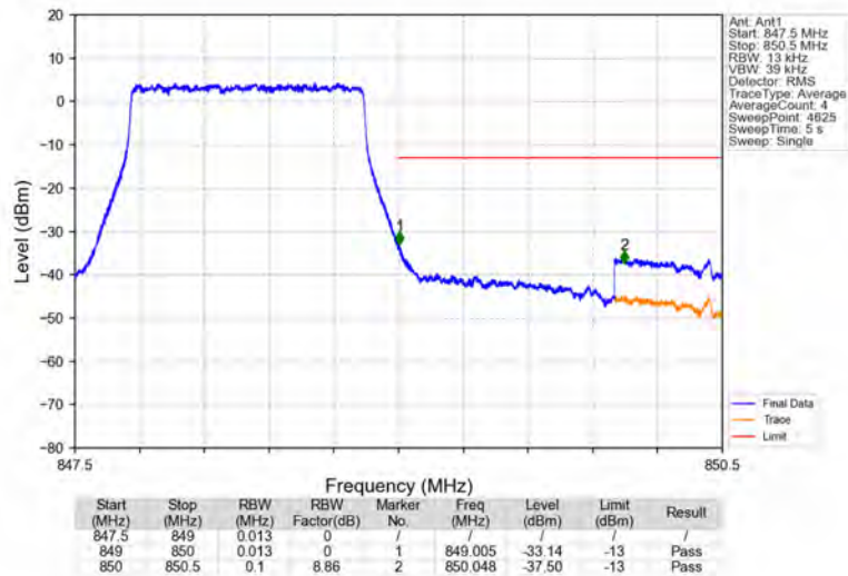
Band26b_1.4MHz_16QAM_HCH_848.3MHz_RB_6_0_NTNV
