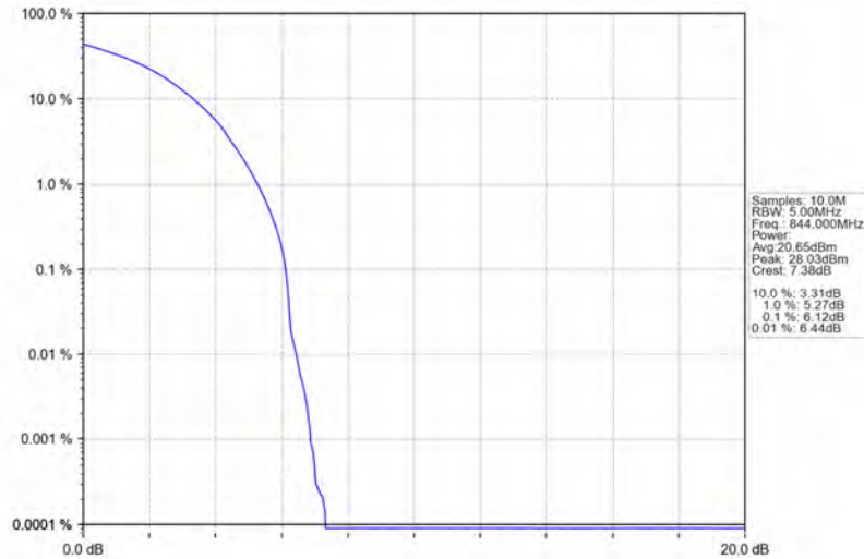
Band26b_10MHz_QPSK_HCH_844MHz_RB_50_0_NTNV
