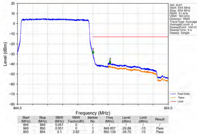
Band26b_5MHz_QPSK_HCH_846.5MHz_RB_25_0_NTNV
