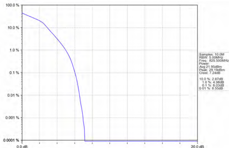
Band26b_3MHz_16QAM_LCH_825.5MHz_RB_15_0_NTNV
