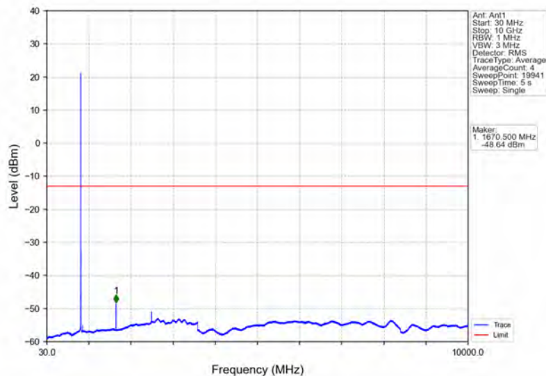
Band26b_3MHz_64QAM_MCH_836.5MHz_RB_1_0_NTNV
