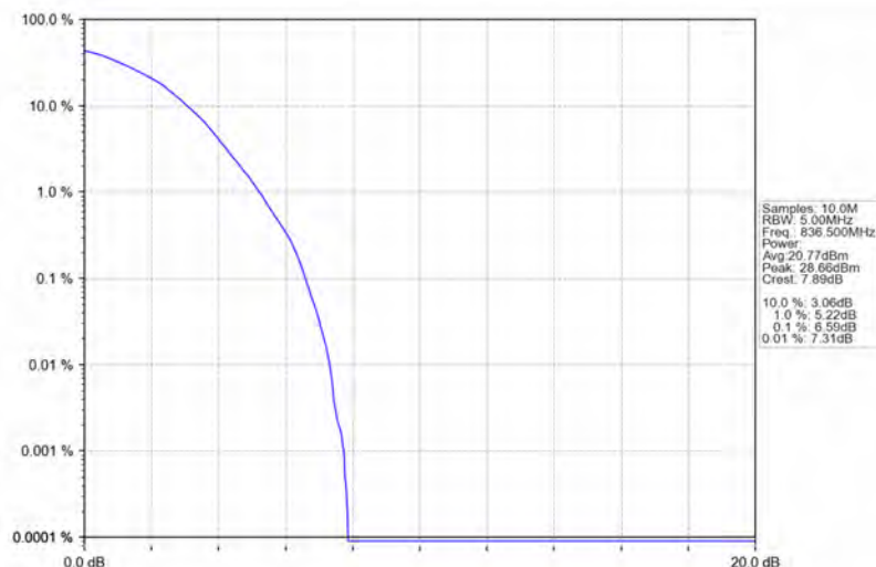
Band26b_1.4MHz_64QAM_MCH_836.5MHz_RB_6_0_NTNV
