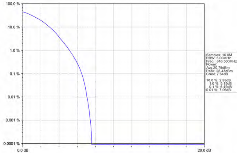
Band26b_5MHz_64QAM_HCH_846.5MHz_RB_25_0_NTNV
