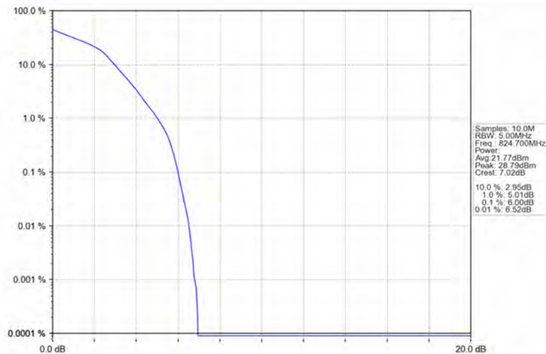
Band26b_1.4MHz_16QAM_LCH_824.7MHz_RB_6_0_NTNV
