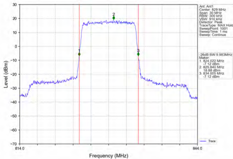
Band26b_10MHz_QPSK_LCH_829MHz_RB_50_0_NTNV
