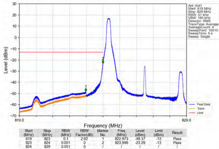
Band26b_5MHz_64QAM_LCH_826.5MHz_RB_1_0_NTNV
