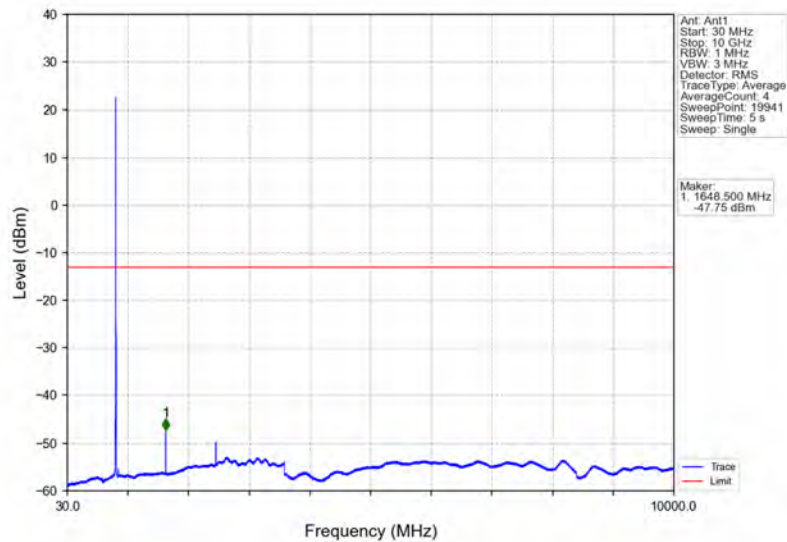
Band26b_5MHz_16QAM_LCH_826.5MHz_RB_25_0_NTNV
