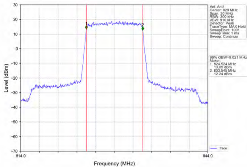
Band26b_10MHz_QPSK_LCH_829MHz_RB_50_0_NTNV
