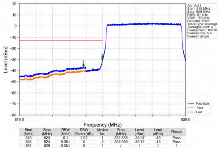
Band26b_5MHz_64QAM_LCH_826.5MHz_RB_25_0_NTNV
