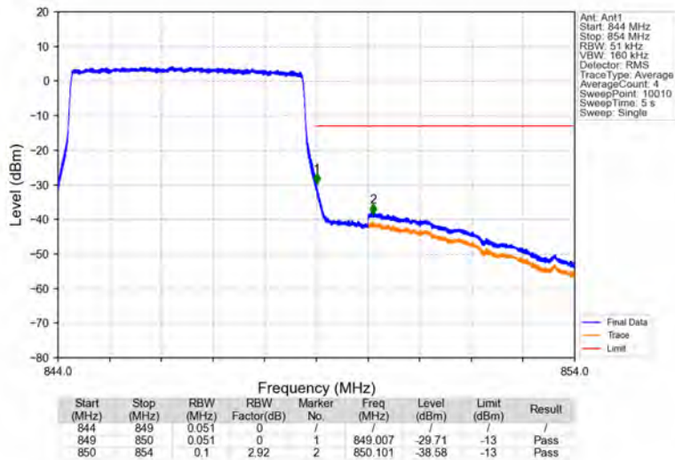
Band26b_5MHz_16QAM_HCH_846.5MHz_RB_25_0_NTNV
