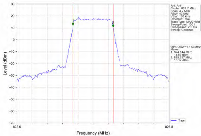
Band26b_1.4MHz_16QAM_LCH_824.7MHz_RB_6_0_NTNV
