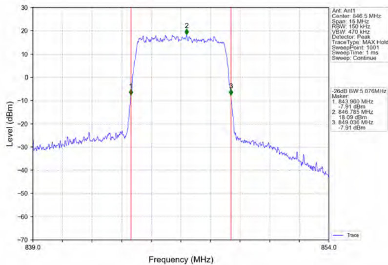
Band26b_5MHz_16QAM_HCH_846.5MHz_RB_25_0_NTNV
