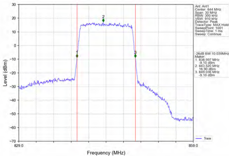
Band26b_10MHz_64QAM_HCH_844MHz_RB_50_0_NTNV
