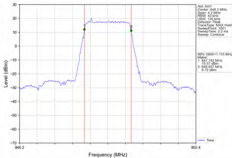
Band26b_1.4MHz_16QAM_HCH_848.3MHz_RB_6_0_NTNV
