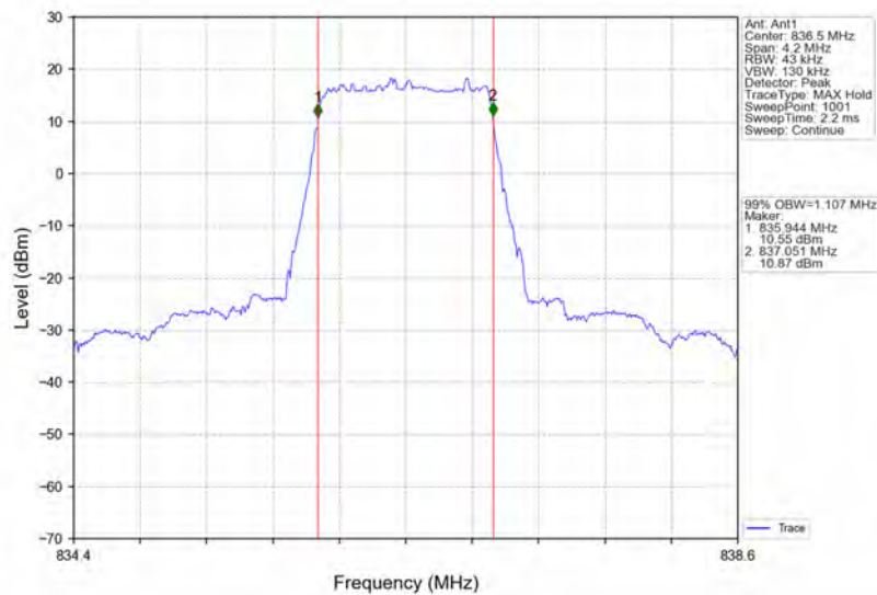
Band26b_1.4MHz_64QAM_MCH_836.5MHz_RB_6_0_NTNV
