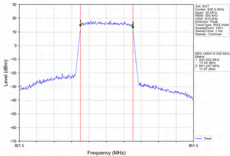
Band26b_10MHz_16QAM_MCH_836.5MHz_RB_50_0_NTNV
