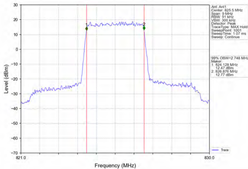
Band26b_3MHz_QPSK_LCH_825.5MHz_RB_15_0_NTNV
