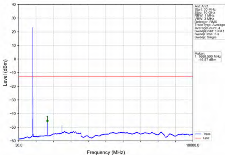
Band26b_5MHz_QPSK_MCH_836.5MHz_RB_1_0_NTNV
