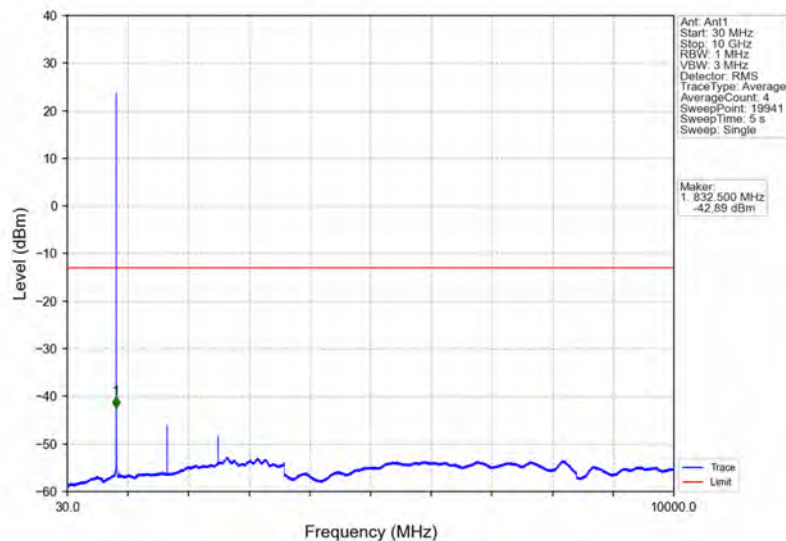
Band26b_1.4MHz_QPSK_MCH_836.5MHz_RB_1_0_NTNV
