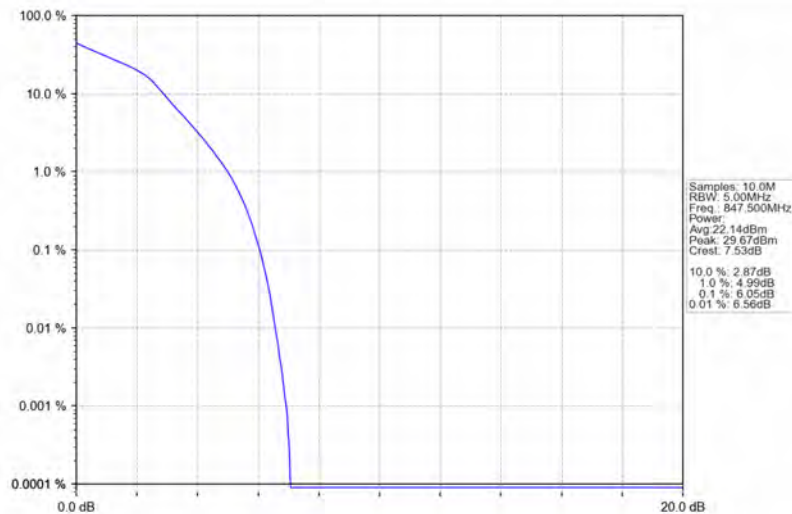
Band26b_3MHz_16QAM_HCH_847.5MHz_RB_15_0_NTNV
