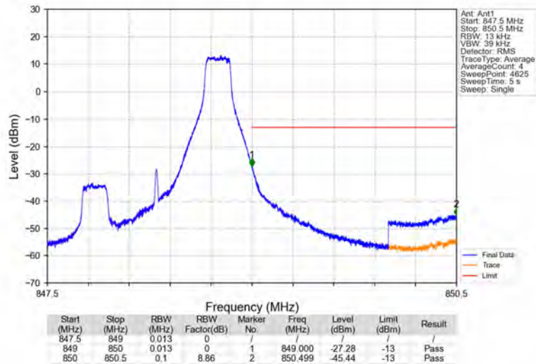
Band26b_1.4MHz_16QAM_HCH_848.3MHz_RB_1_5_NTNV
