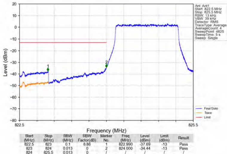
Band26b_1.4MHz_64QAM_LCH_824.7MHz_RB_6_0_NTNV
