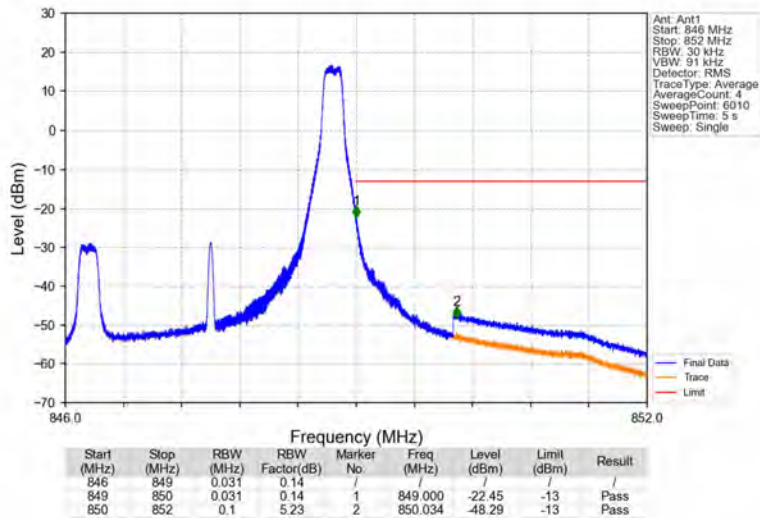
Band26b_3MHz_16QAM_HCH_847.5MHz_RB_1_14_NTNV
