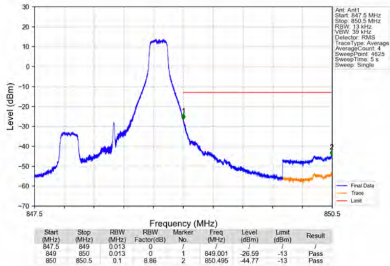
Band26b_1.4MHz_QPSK_HCH_848.3MHz_RB_1_5_NTNV
