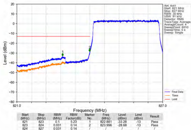
Band26b_3MHz_16QAM_LCH_825.5MHz_RB_15_0_NTNV
