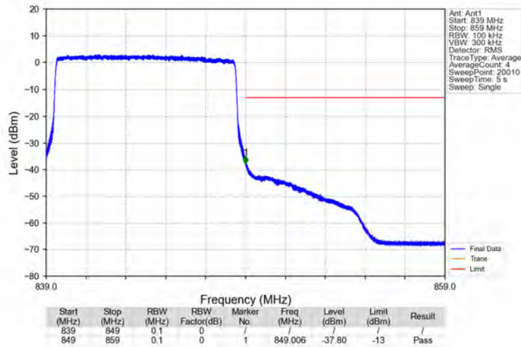
Band26b_10MHz_64QAM_HCH_844MHz_RB_50_0_NTNV
