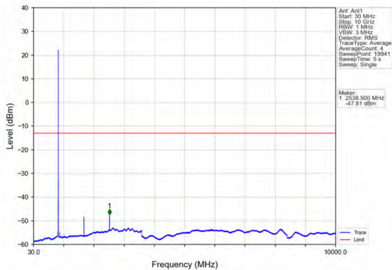
Band26b_3MHz_16QAM_HCH_847.5MHz_RB_1_0_NTNV
