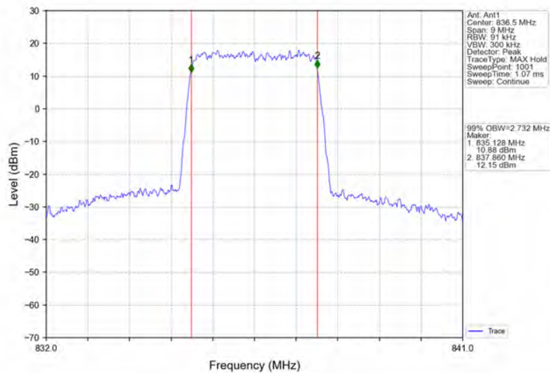
Band26b_3MHz_16QAM_MCH_836.5MHz_RB_15_0_NTNV
