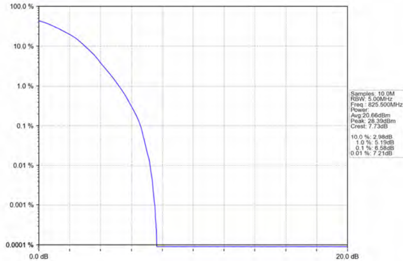
Band26b_3MHz_64QAM_LCH_825.5MHz_RB_15_0_NTNV
