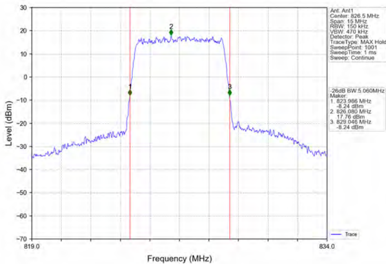
Band26b_5MHz_16QAM_LCH_826.5MHz_RB_25_0_NTNV
