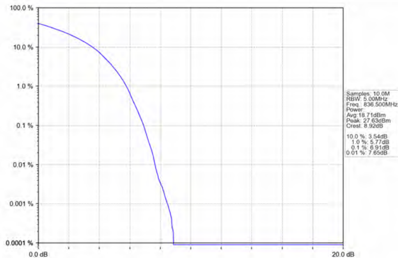
Band26b_10MHz_64QAM_MCH_836.5MHz_RB_50_0_NTNV
