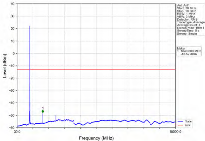
Band26b_10MHz_16QAM_LCH_829MHz_RB_50_0_NTNV
