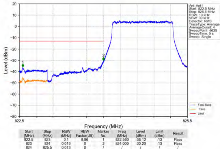
Band26b_1.4MHz_QPSK_LCH_824.7MHz_RB_6_0_NTNV
