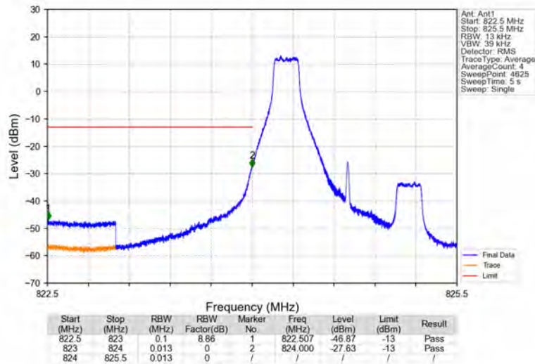
Band26b_1.4MHz_16QAM_LCH_824.7MHz_RB_1_0_NTNV
