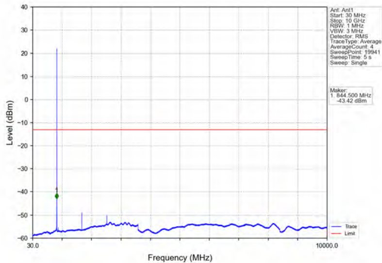
Band26b_1.4MHz_64QAM_HCH_848.3MHz_RB_1_5_NTNV
