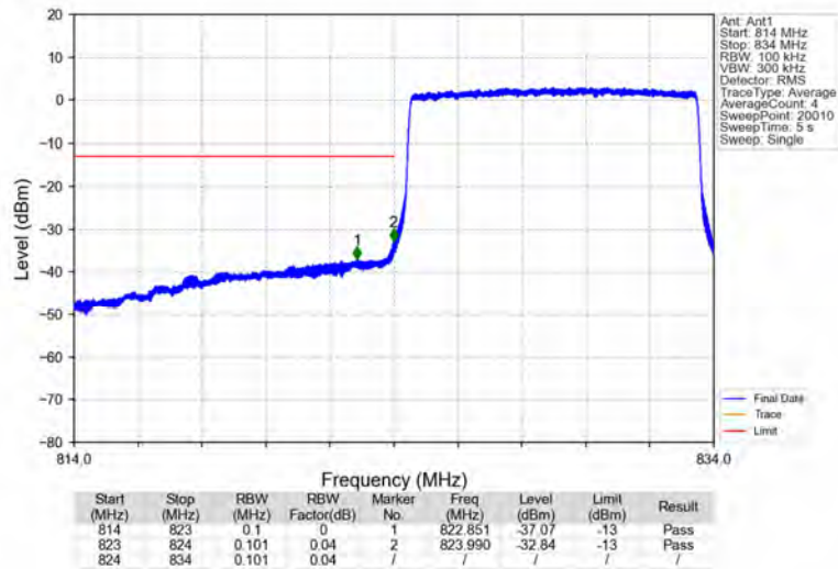
Band26b_10MHz_64QAM_LCH_829MHz_RB_50_0_NTNV
