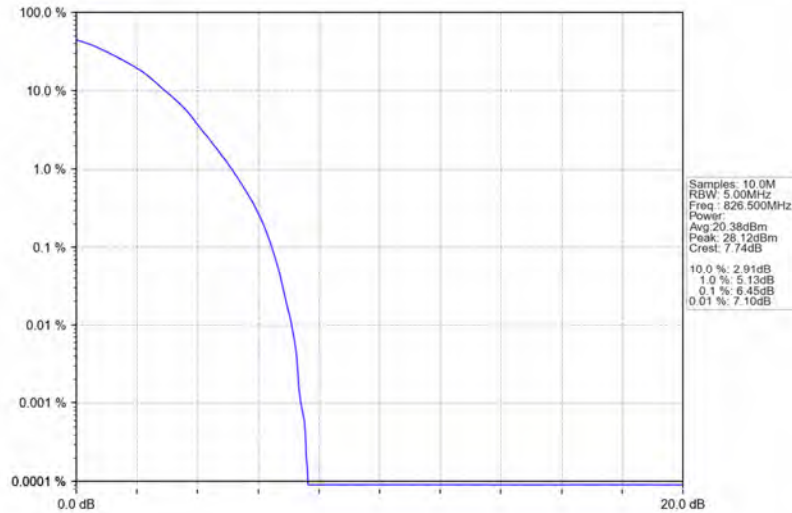
Band26b_5MHz_64QAM_LCH_826.5MHz_RB_25_0_NTNV
