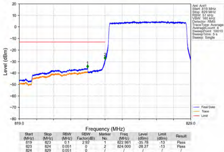
Band26b_5MHz_QPSK_LCH_826.5MHz_RB_25_0_NTNV
