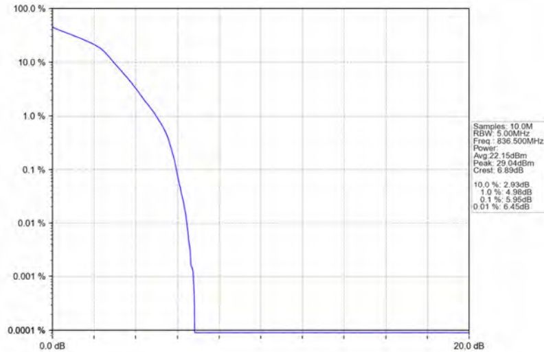
Band26b_1.4MHz_16QAM_MCH_836.5MHz_RB_6_0_NTNV
