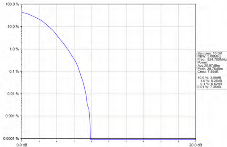
Band26b_1.4MHz_64QAM_LCH_824.7MHz_RB_6_0_NTNV
