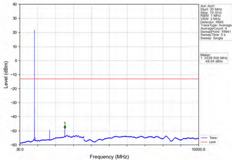
Band26b_3MHz_64QAM_HCH_847.5MHz_RB_1_14_NTNV
