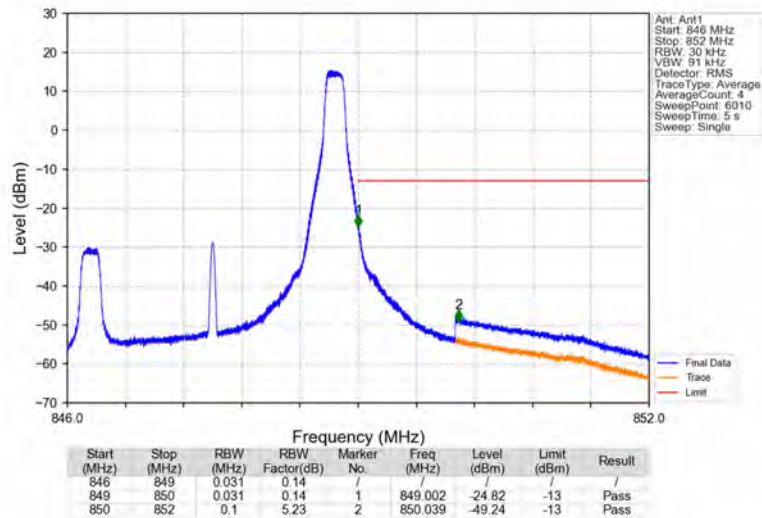
Band26b_3MHz_64QAM_HCH_847.5MHz_RB_1_14_NTNV
