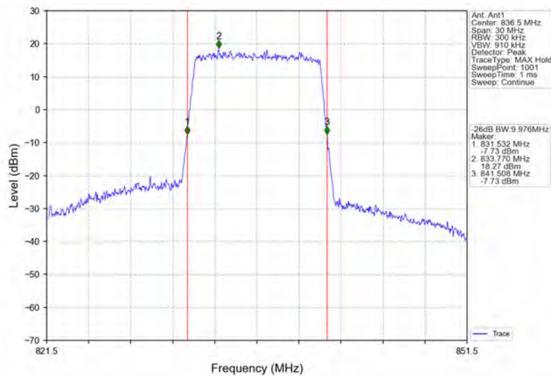
Band26b_10MHz_16QAM_MCH_836.5MHz_RB_50_0_NTNV
