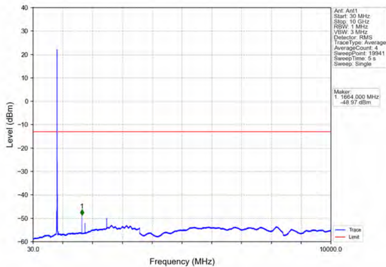
Band26b_10MHz_64QAM_MCH_836.5MHz_RB_1_0_NTNV
