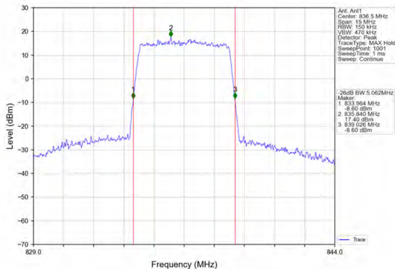
Band26b_5MHz_64QAM_MCH_836.5MHz_RB_25_0_NTNV
