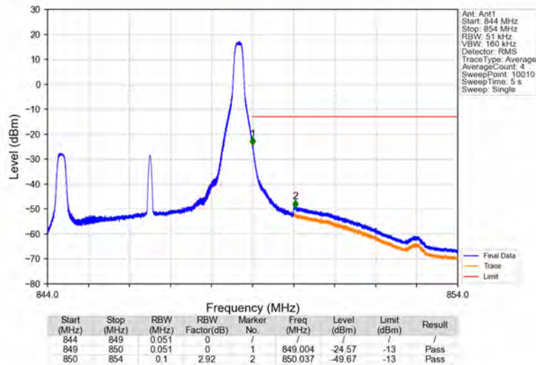
Band26b_5MHz_64QAM_HCH_846.5MHz_RB_1_24_NTNV
