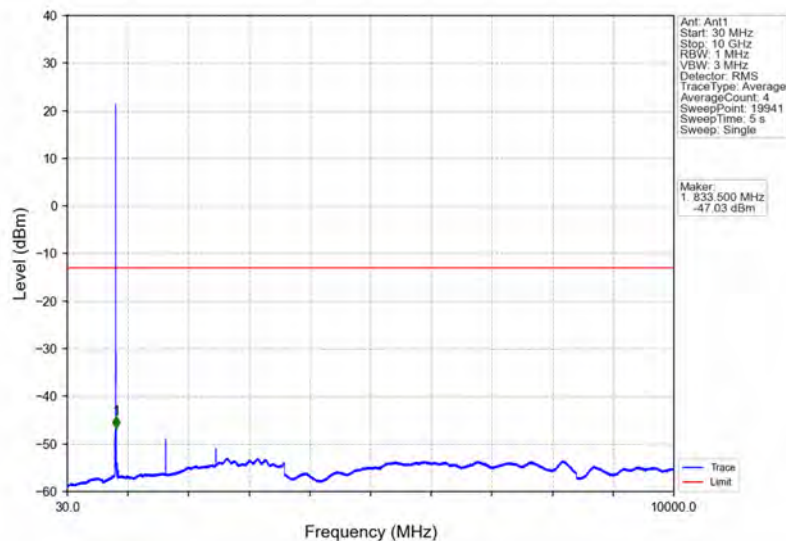
Band26b_3MHz_64QAM_LCH_825.5MHz_RB_1_0_NTNV
