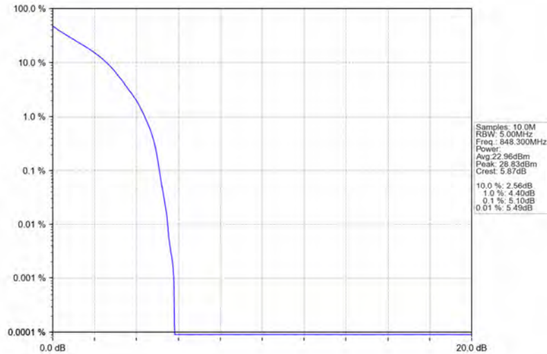
Band26b_1.4MHz_QPSK_HCH_848.3MHz_RB_6_0_NTNV
