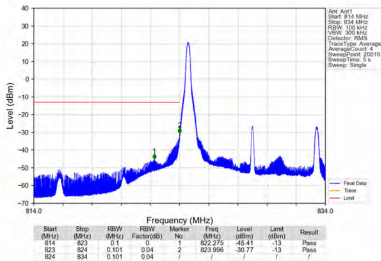
Band26b_10MHz_16QAM_LCH_829MHz_RB_1_0_NTNV
