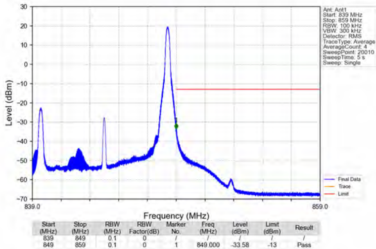
Band26b_10MHz_64QAM_HCH_844MHz_RB_1_49_NTNV
