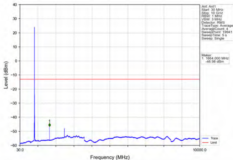
Band26b_10MHz_QPSK_MCH_836.5MHz_RB_1_0_NTNV
