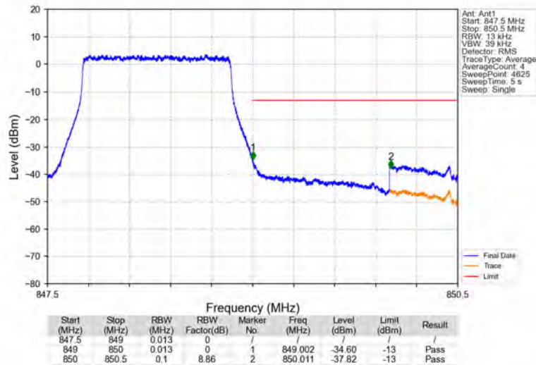
Band26b_1.4MHz_64QAM_HCH_848.3MHz_RB_6_0_NTNV
