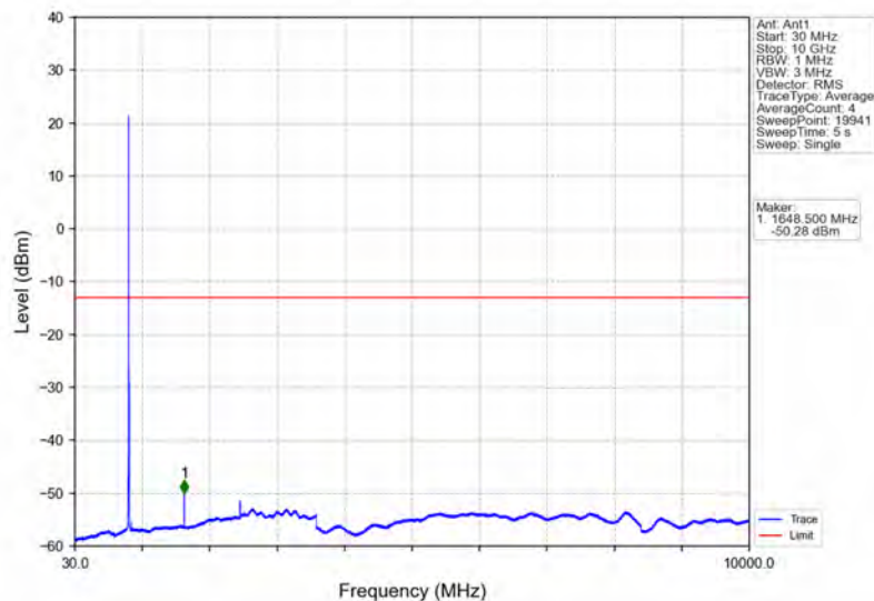
Band26b_5MHz_64QAM_LCH_826.5MHz_RB_1_0_NTNV
