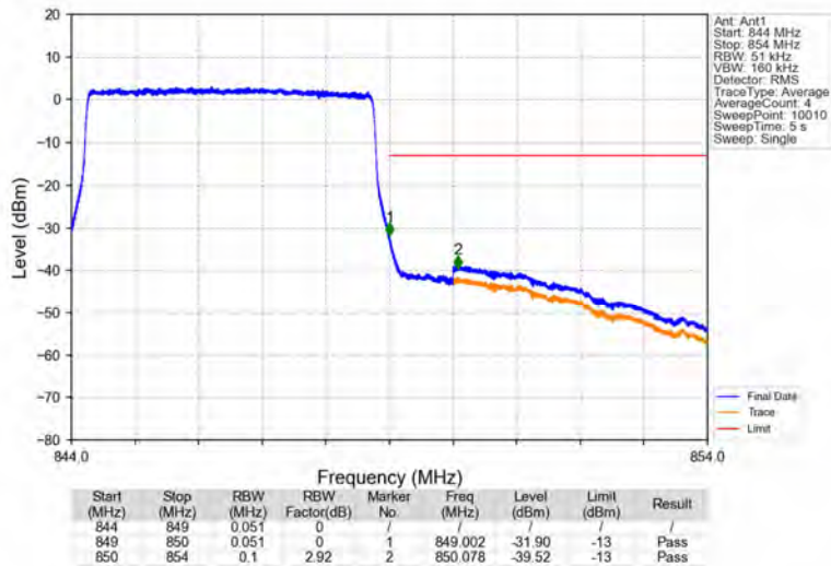
Band26b_5MHz_64QAM_HCH_846.5MHz_RB_25_0_NTNV
