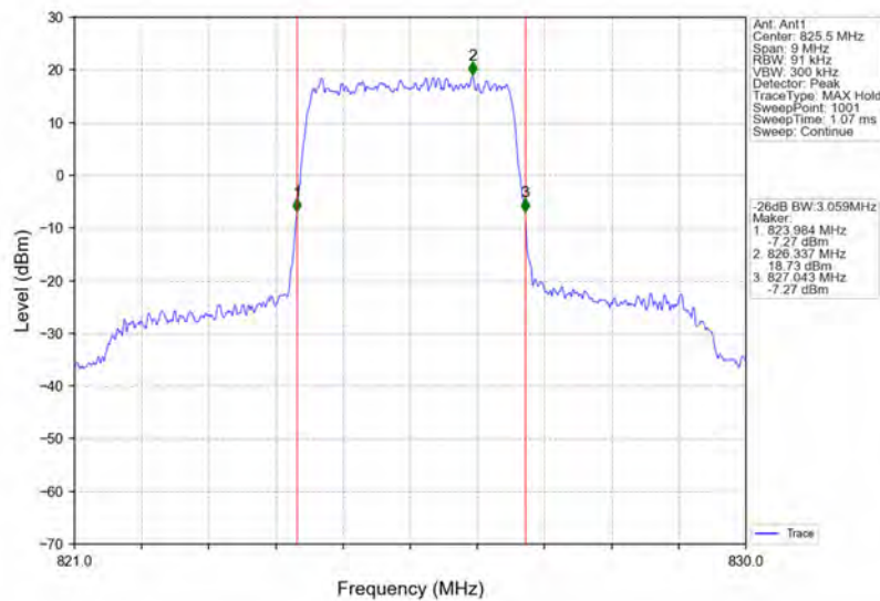
Band26b_3MHz_QPSK_LCH_825.5MHz_RB_15_0_NTNV
