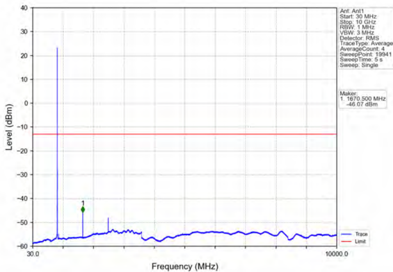
Band26b_3MHz_QPSK_MCH_836.5MHz_RB_1_0_NTNV
