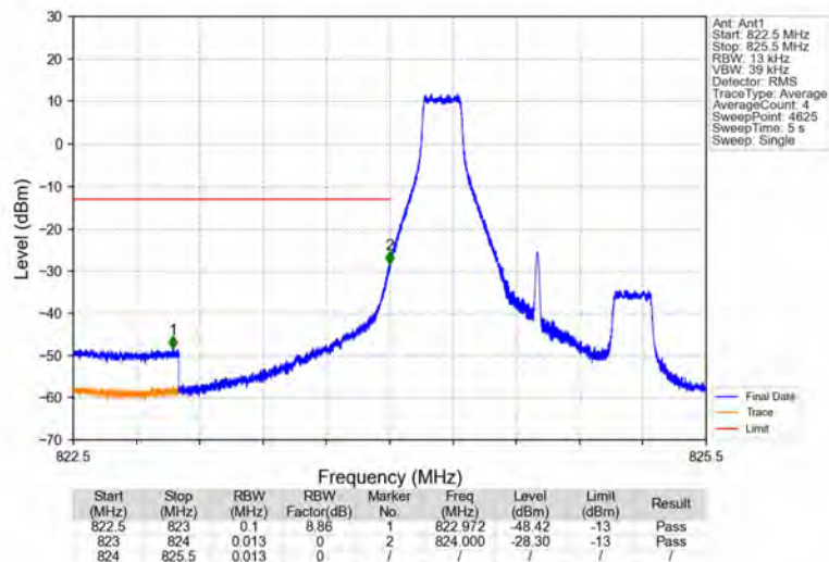
Band26b_1.4MHz_64QAM_LCH_824.7MHz_RB_1_0_NTNV
