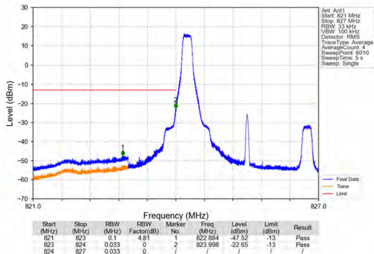
Band26b_3MHz_64QAM_LCH_825.5MHz_RB_1_0_NTNV
