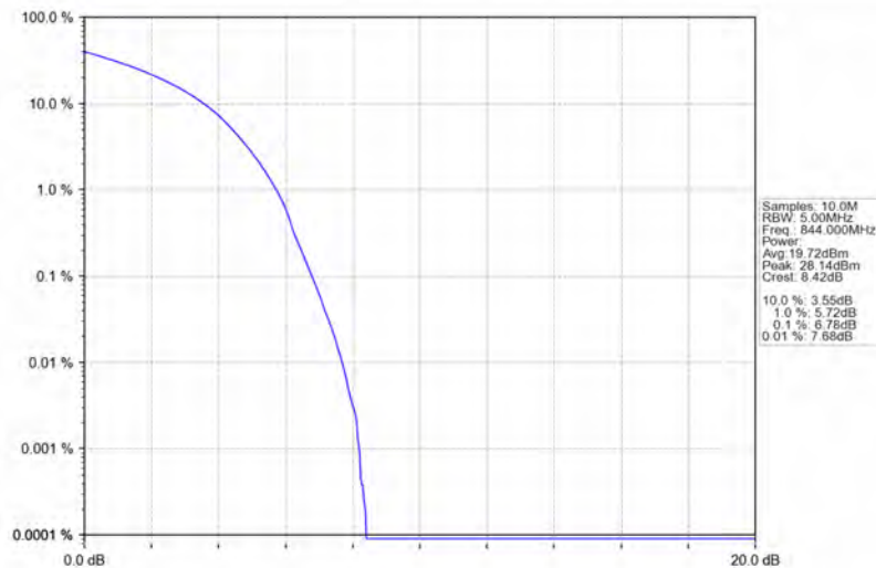
Band26b_10MHz_16QAM_HCH_844MHz_RB_50_0_NTNV
