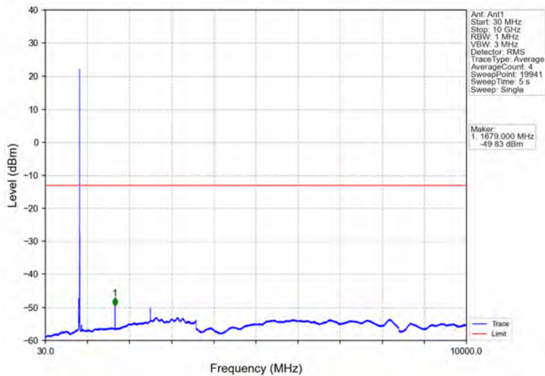
Band26b_10MHz_64QAM_HCH_844MHz_RB_1_49_NTNV
