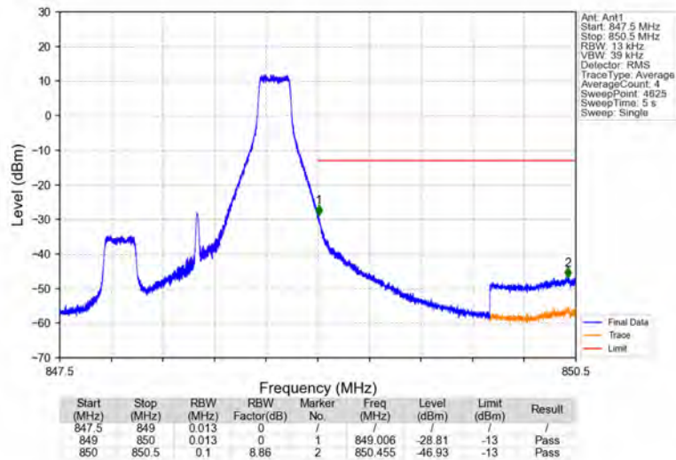
Band26b_1.4MHz_64QAM_HCH_848.3MHz_RB_1_5_NTNV
