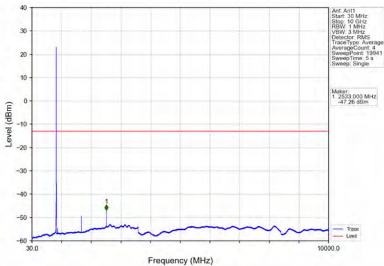
Band26b_5MHz_16QAM_HCH_846.5MHz_RB_1_0_NTNV
