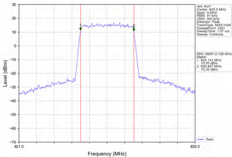
Band26b_3MHz_64QAM_LCH_825.5MHz_RB_15_0_NTNV
