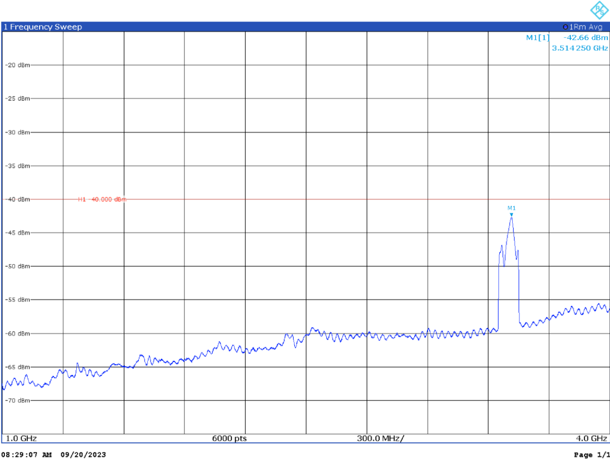
100 MHz signal, Bottom=Middle=Top Channel, 1GHz - 4GHz, V Pol
