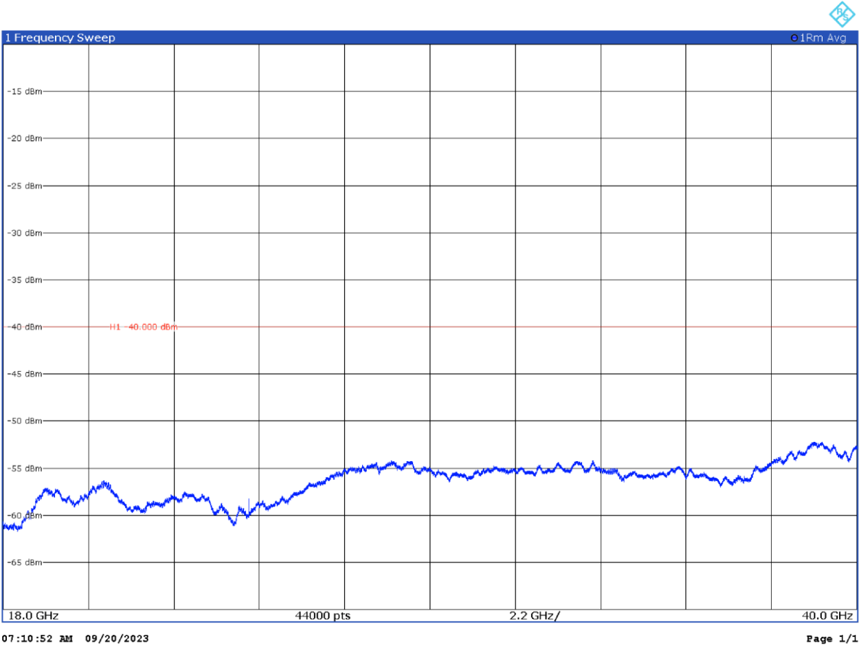
100 MHz signal, Bottom=Middle=Top Channel, 18GHz - 40GHz, V Pol
