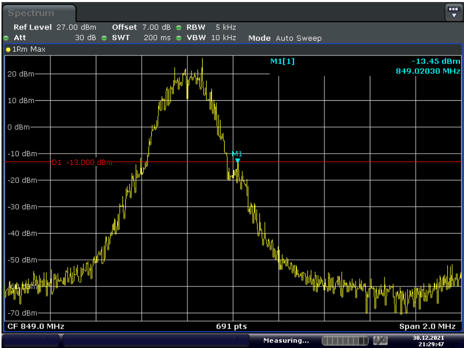
Cellular Band, Right Band Edge for GSM (GMSK) Mode
