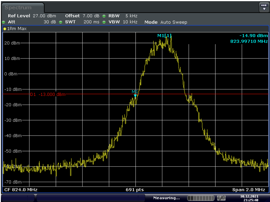
Cellular Band, Left Band Edge for GSM (GMSK) Mode
