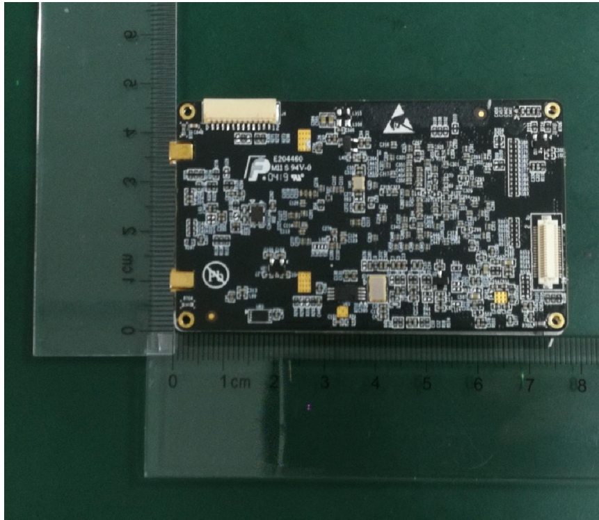
(10) EUT Photo (Model: WLN210-BM-b)
