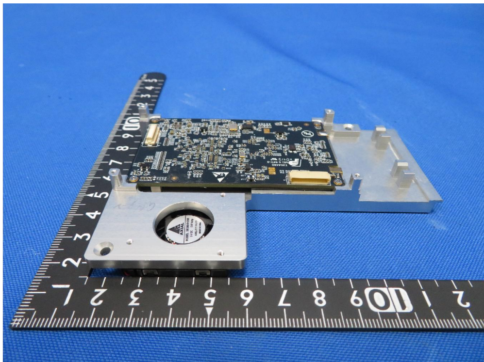
(14) EUT Photo (Model: WLN210-BM-c)
