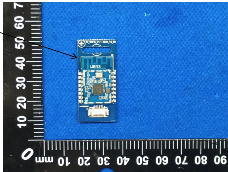
WIFI 2.4G ANT
