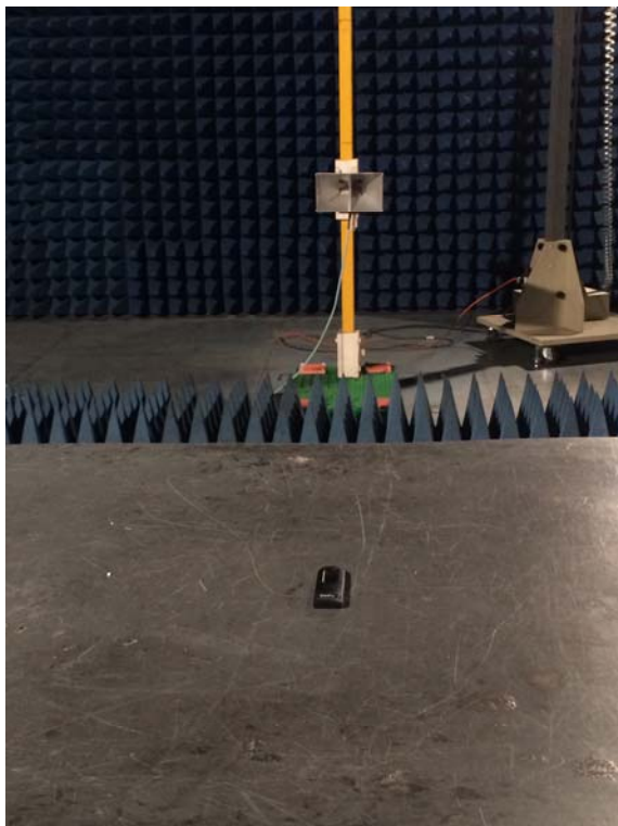
Radiated emissions test > 1GHz
