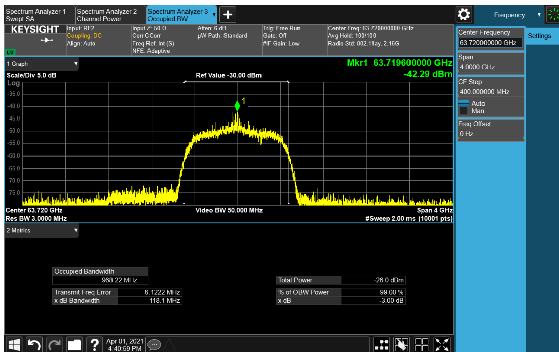
Wave-AP_1GHz_63.72GHz_Peak
