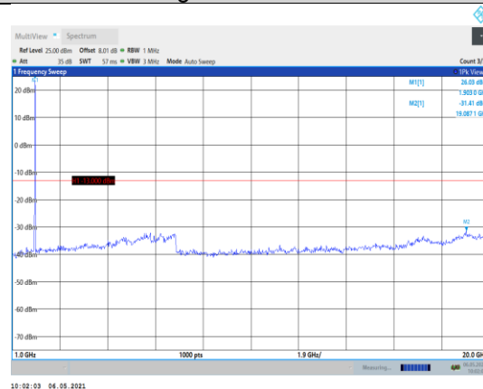
Band2-15MHz-16QAM-19125-1RB#0- Range2:1000~20000MHz
