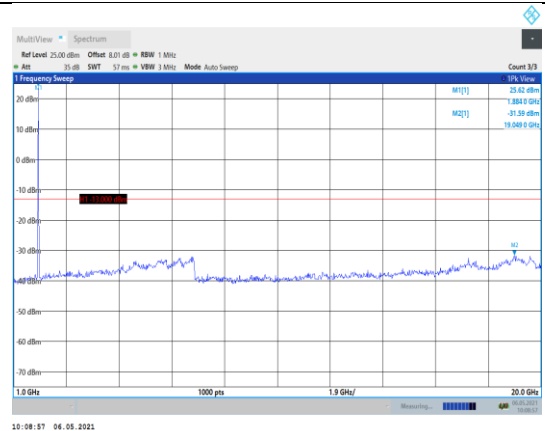
Band2-10MHz-QPSK-18900-1RB#0- Range2:1000~20000MHz
