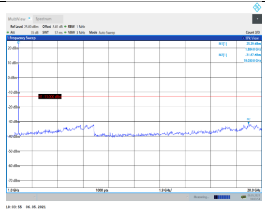
Band2-5MHz-16QAM-18900-1RB#0- Range2:1000~20000MHz
