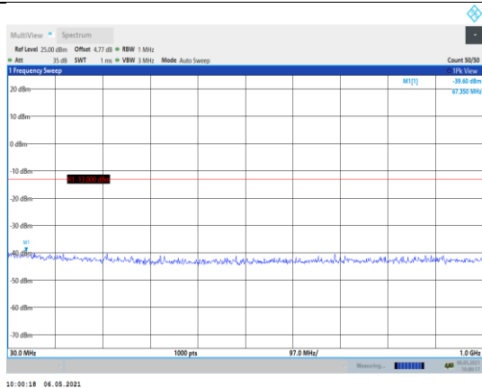
Band2-15MHz-16QAM-18675-1RB#0- Range1:30~1000MHz
