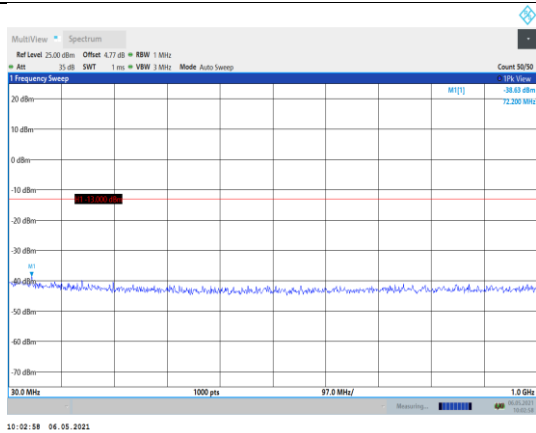
Band2-5MHz-16QAM-18625-1RB#0- Range1:30~1000MHz
