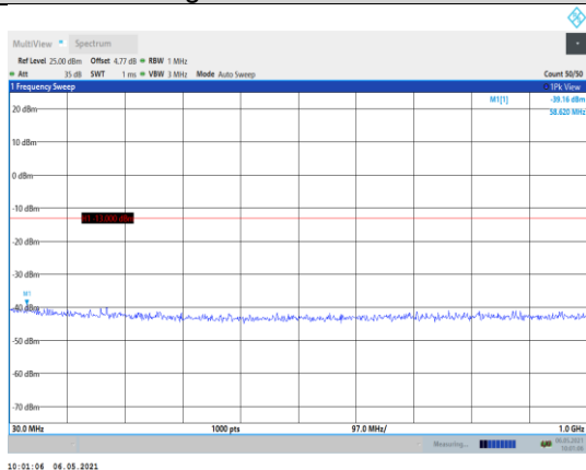
Band2-15MHz-16QAM-18900-1RB#0- Range1:30~1000MHz
