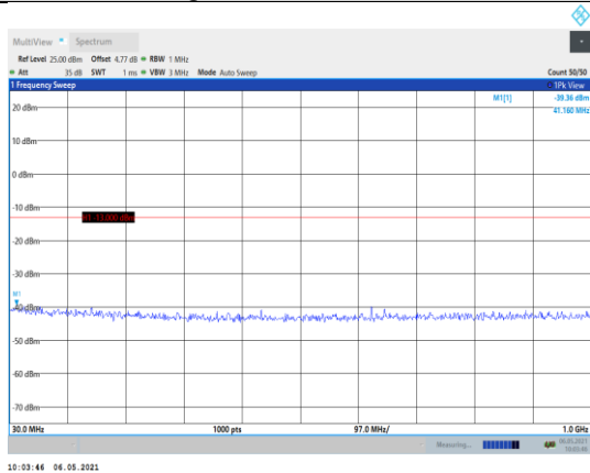
Band2-5MHz-16QAM-18900-1RB#0- Range1:30~1000MHz
