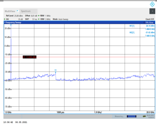
Band2-3MHz-16QAM-18900-1RB#0- Range2:1000~20000MHz
