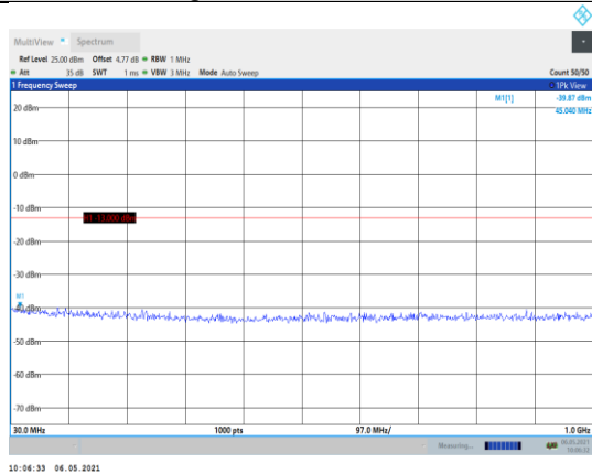
Band2-3MHz-16QAM-18900-1RB#0- Range1:30~1000MHz
