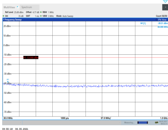
Band2-1.4MHz-QPSK-18900-1RB#0- Range1:30~1000MHz
