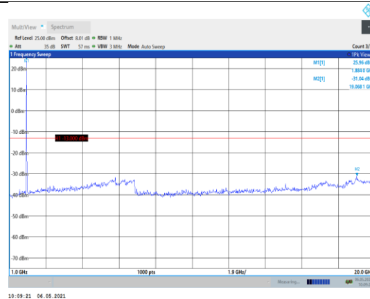
Band2-10MHz-16QAM-18900-1RB#0- Range2:1000~20000MHz
