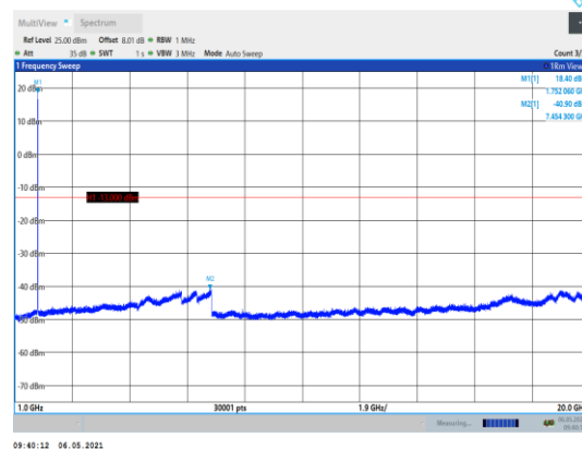
Band4-1513-1000~20000MHz
