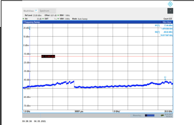
Band2-9400-1000~20000MHz
