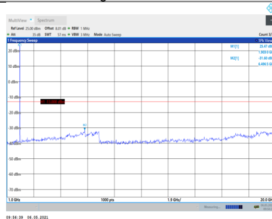
Band2-1.4MHz-16QAM-19193-1RB#0- Range2:1000~20000MHz
