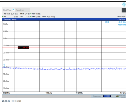
Band2-5MHz-QPSK-18625-1RB#0- Range1:30~1000MHz
