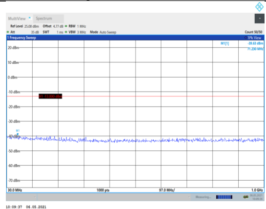
Band2-10MHz-QPSK-19150-1RB#0- Range1:30~1000MHz
