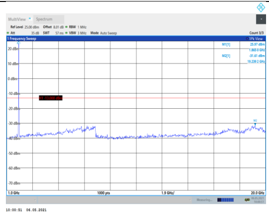
Band2-15MHz-QPSK-18900-1RB#0- Range2:1000~20000MHz
