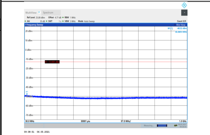
Band2-9538-30~1000MHz
