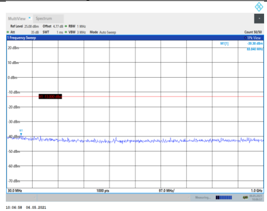
Band2-3MHz-QPSK-19185-1RB#0- Range1:30~1000MHz
