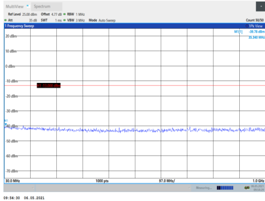
Band2-1.4MHz-QPSK-18607-1RB#0- Range1:30~1000MHz
