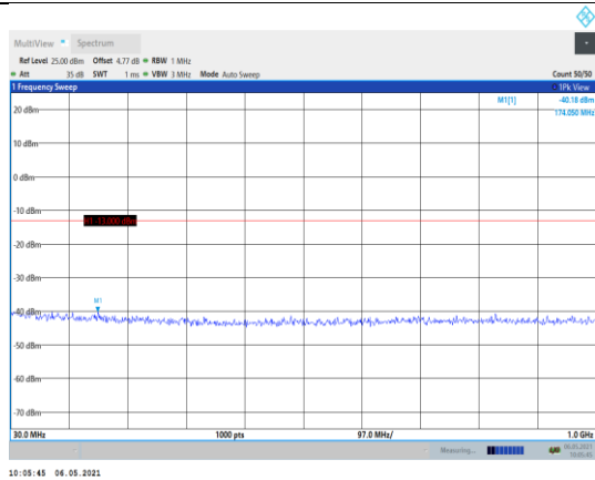
Band2-3MHz-16QAM-18615-1RB#0- Range1:30~1000MHz
