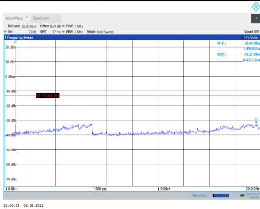
Band2-15MHz-QPSK-18675-1RB#0- Range2:1000~20000MHz
