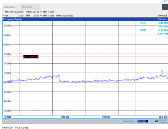
Band2-1.4MHz-QPSK-18607-1RB#0- Range2:1000~20000MHz
