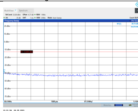
Band2-15MHz-16QAM-19125-1RB#0- Range1:30~1000MHz
