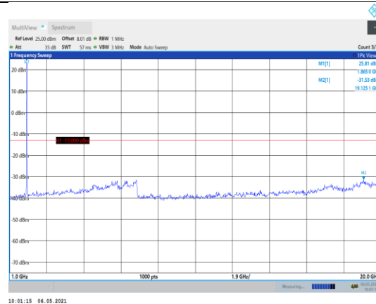
Band2-15MHz-16QAM-18900-1RB#0- Range2:1000~20000MHz
