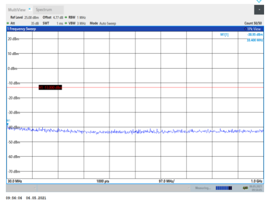
Band2-1.4MHz-QPSK-19193-1RB#0- Range1:30~1000MHz
