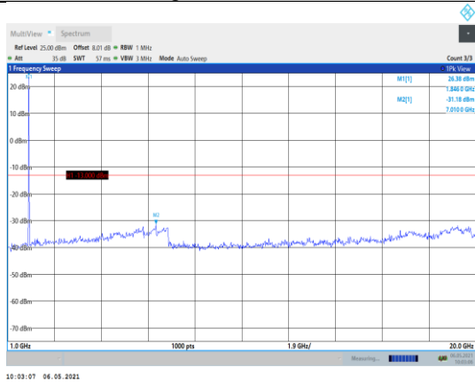
Band2-5MHz-16QAM-18625-1RB#0- Range2:1000~20000MHz
