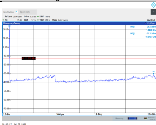
Band2-15MHz-16QAM-18675-1RB#0- Range2:1000~20000MHz
