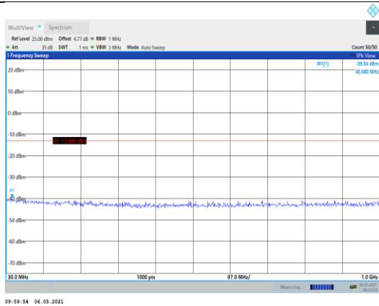
Band2-15MHz-QPSK-18675-1RB#0- Range1:30~1000MHz
