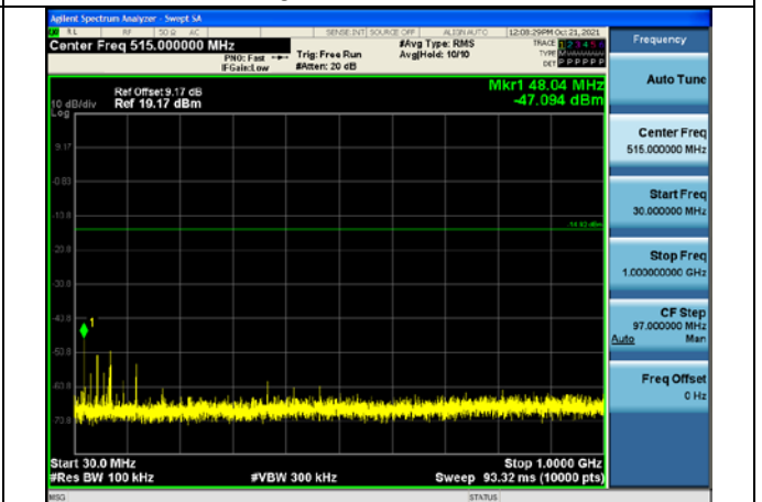
\pi/4 -DQPSK on Channel 78
