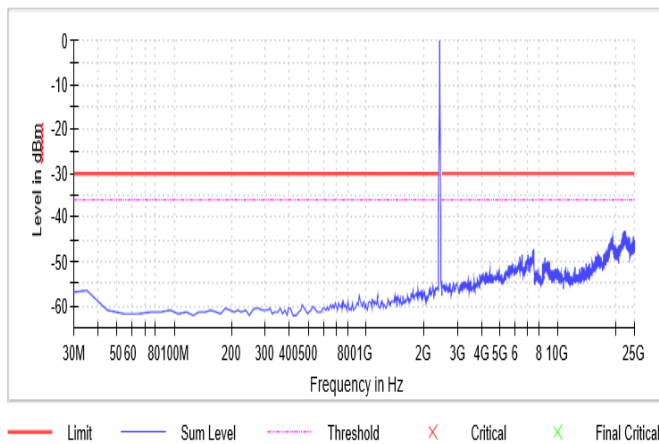
Spurious
