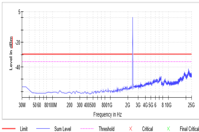
Spurious
