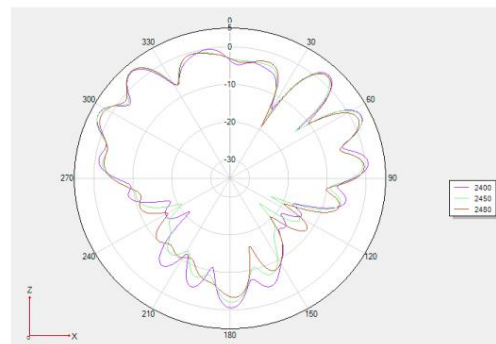
Phi 0 2D
