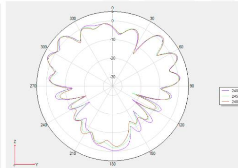
Phi 90 2D
