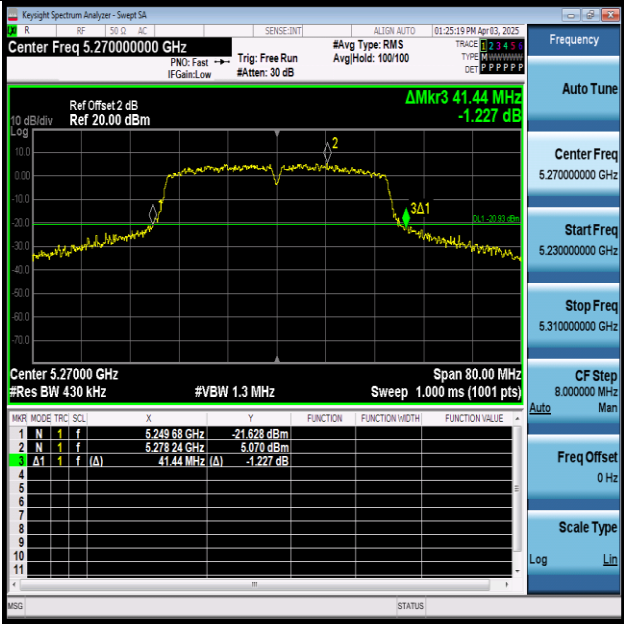
11AC40SISO-Ant1-5270
