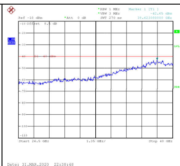
15MHz - Middle CH 26.5GHz~40GHz
