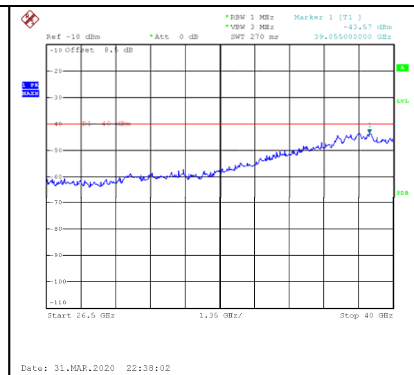
5MHz - Middle CH 26.5GHz~40GHz
