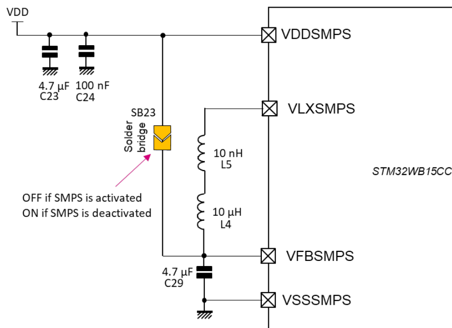
Figure 15. SMPS part
