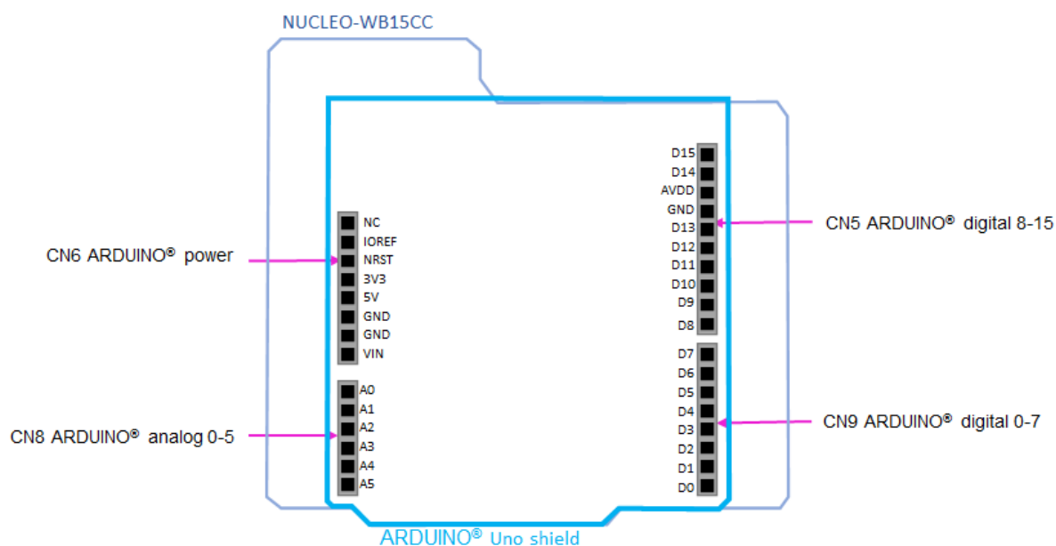
Figure 17. ARDUINO® connector location and pinout
