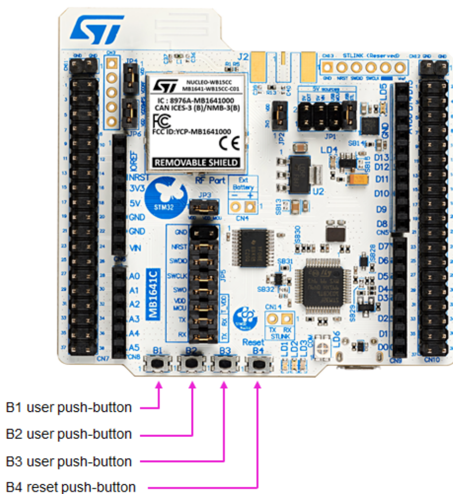
Figure 13. Push-buttons location
