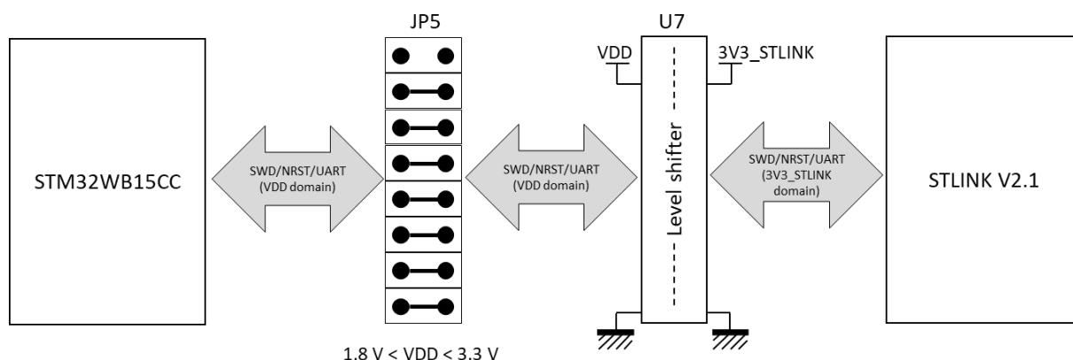
Figure 11. Interconnection bloc diagram between STM32WB15CC and ST-LINK/V2-1
