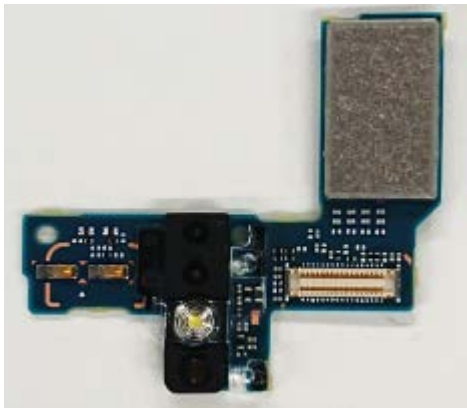
Internal Sub-PWB with Shield cases (Front-side)
