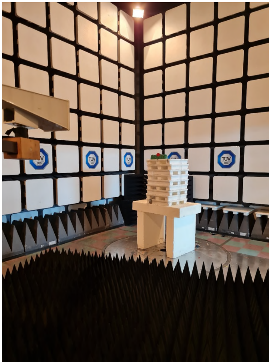
Figure 5 – Radiated Emissions Setup
