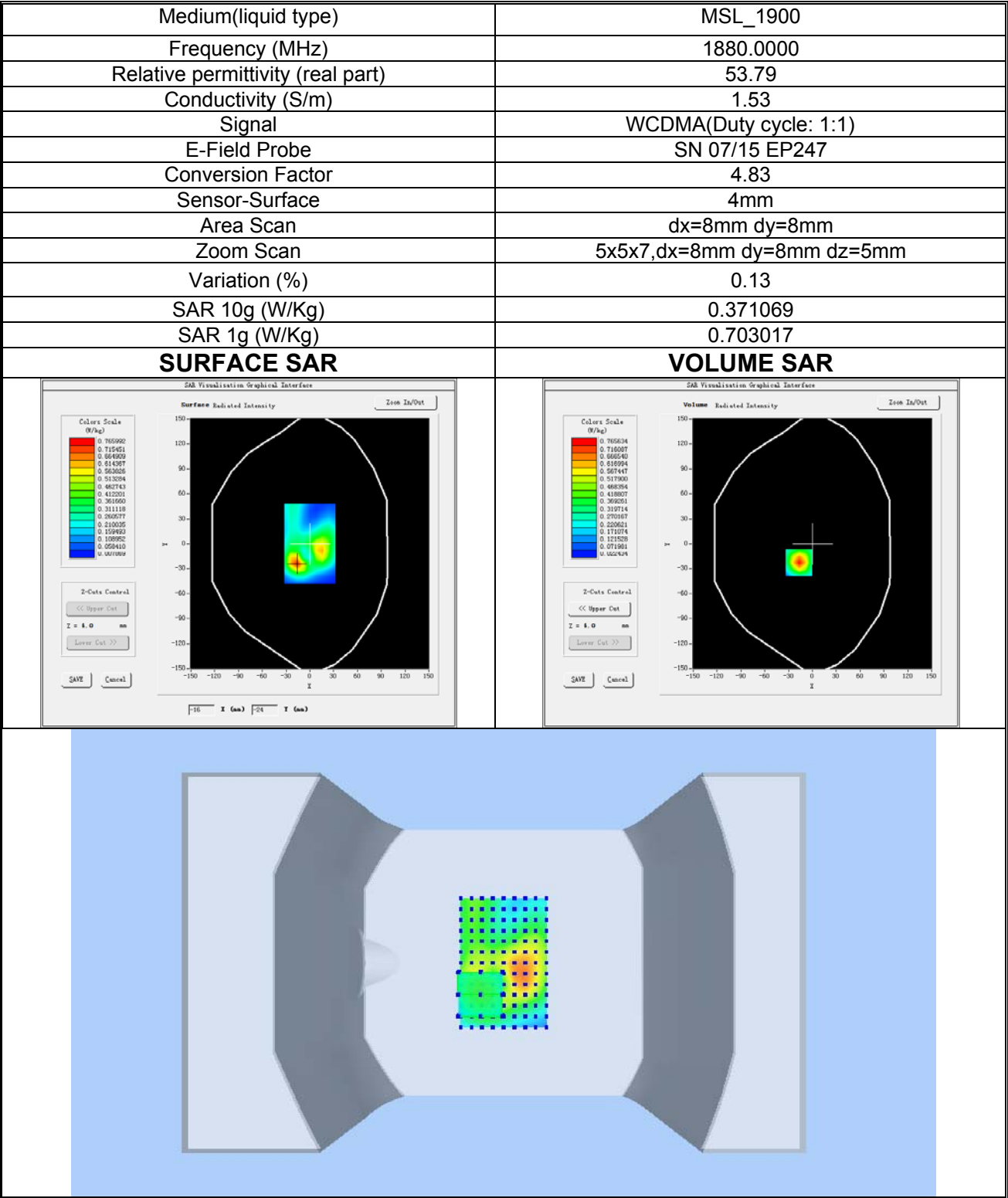
Plot 9: WCDMA BAND II , Middle channel (Body-worn/Hotspot, Back Surface) Product Description: SMARTPHONE Test Date: 2019-11-04
