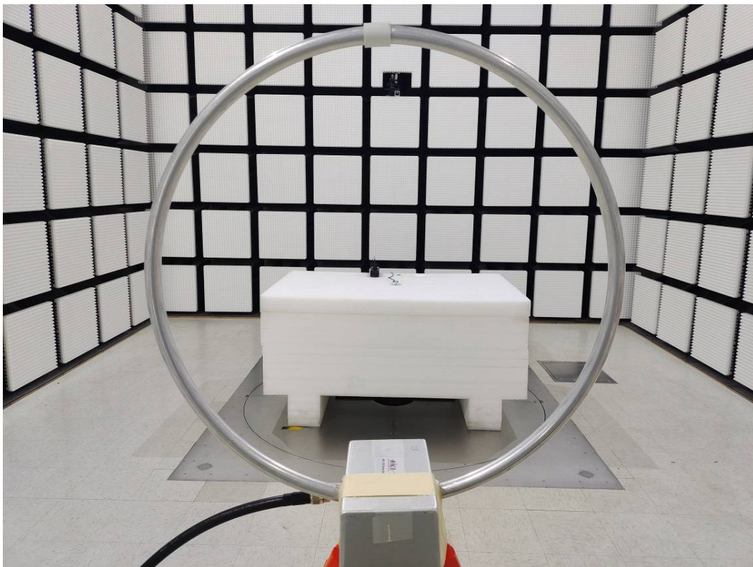
Radiated Emission Below 30MHz View Perpendicular
