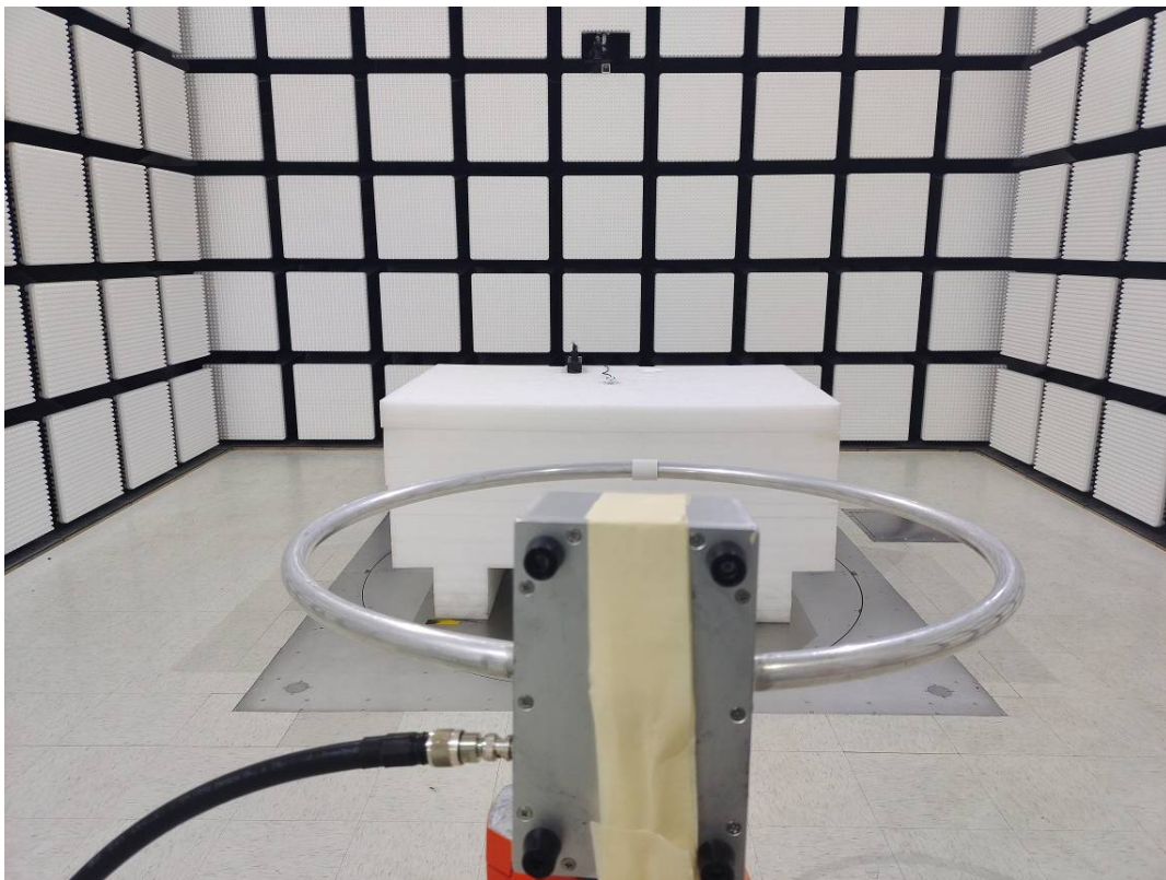
Radiated Emission Below 30MHz View Ground-parallel
