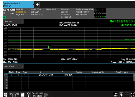
B41_N77(50M)_DFT-s-OFDM_BPSK_Edge_1RB_Left_Low_CH
