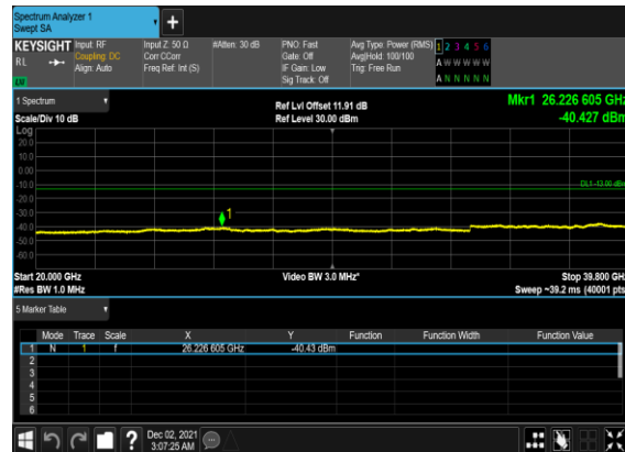
B41_N77(20M)_DFT-s-OFDM_QPSK_Edge_1RB_Left_Low_CH
