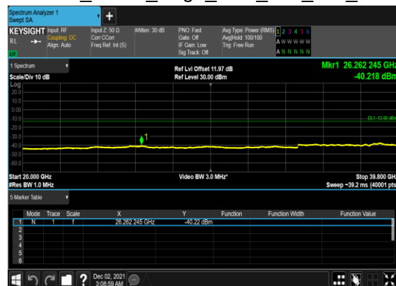
B41_N77(20M)_DFT-s-OFDM_BPSK_Edge_1RB_Left_Mid_CH
