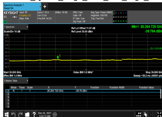
B41_N77(50M)_DFT-s- OFDM_QPSK_Edge_1RB_Left_High_CH
