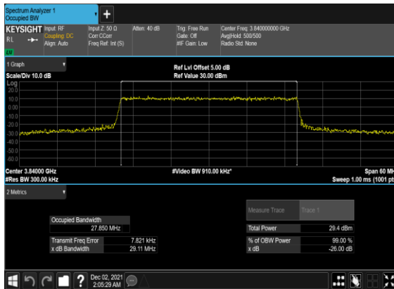
B41_N77(30M)_CP- OFDM_QPSK_Outer_Full_Mid_CH
