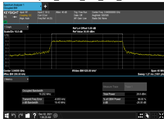
B41_N77(20M)_CP-OFDM_16 QAM_Outer_Full_Mid_CH
