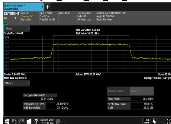
B41_N77(30M)_CP-OFDM_256 QAM_Outer_Full_Mid_CH
