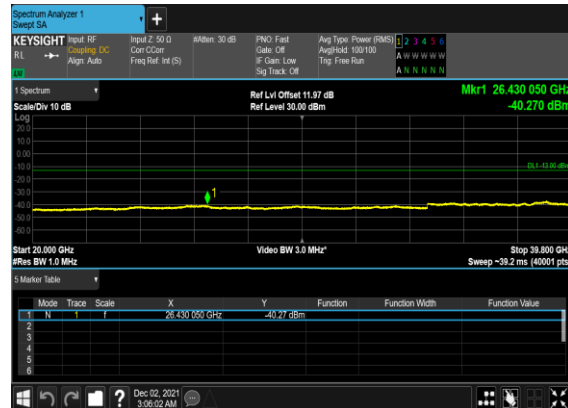
B41_N77(20M)_DFT-s-OFDM_BPSK_Edge_1RB_Left_Low_CH
