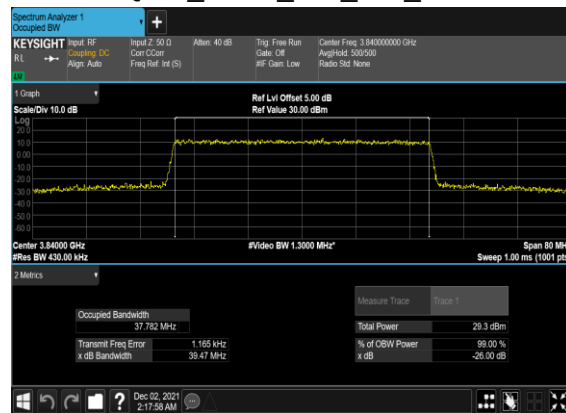
B41_N77(40M)_CP-OFDM_16 QAM_Outer_Full_Mid_CH
