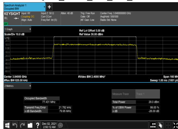
B41_N77(80M)_CP-OFDM_16 QAM_Outer_Full_Mid_CH
