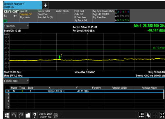
B41_N77(100M)_DFT-s-OFDM_BPSK_Edge_1RB_Left_High_CH
