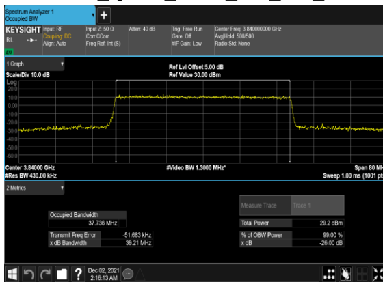
B41_N77(40M)_CP- OFDM_QPSK_Outer_Full_Mid_CH
