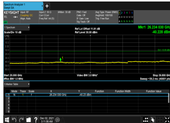
B41_N77(20M)_DFT-s-OFDM_BPSK_Edge_1RB_Left_High_CH
