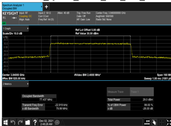
B41_N77(80M)_CP- OFDM_QPSK_Outer_Full_Mid_CH
