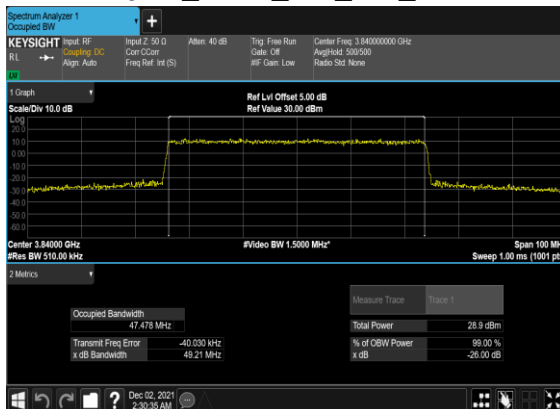
B41_N77(50M)_CP-OFDM_64 QAM_Outer_Full_Mid_CH
