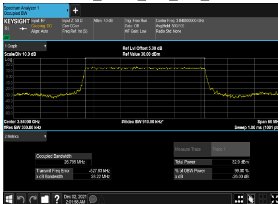
B41_N77(30M)_DFT-s-OFDM_PI_2- BPSK_Outer_Full_Mid_CH
