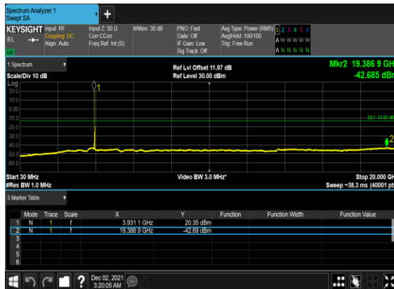
B41_N77(50M)_DFT-s- OFDM_BPSK_Edge_1RB_Left_High_CH
