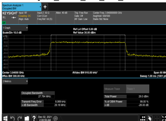
B41_N77(30M)_CP-OFDM_64 QAM_Outer_Full_Mid_CH
