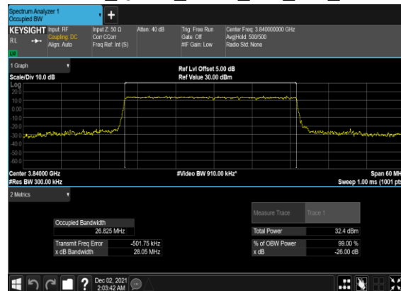
B41_N77(30M)_DFT-s- OFDM_QPSK_Outer_Full_Mid_CH
