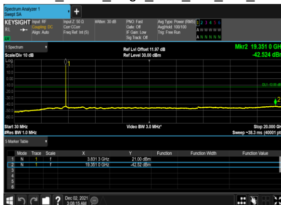
B41_N77(20M)_DFT-s-OFDM_BPSK_Edge_1RB_Left_Mid_CH
