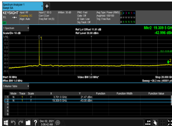
B41_N77(20M)_DFT-s-OFDM_QPSK_Edge_1RB_Left_Low_CH
