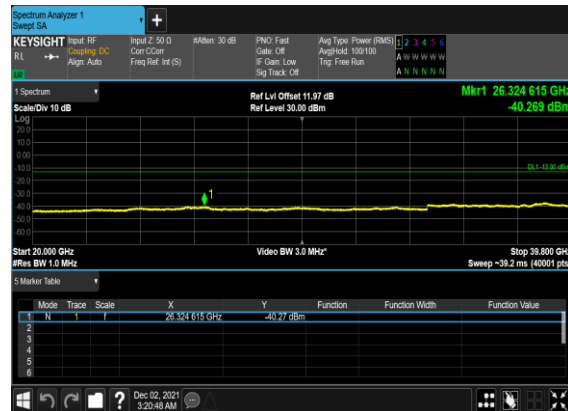
B41_N77(50M)_DFT-s- OFDM_BPSK_Edge_1RB_Left_High_CH
