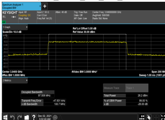
B41_N77(100M)_CP-OFDM_64 QAM_Outer_Full_Mid_CH
