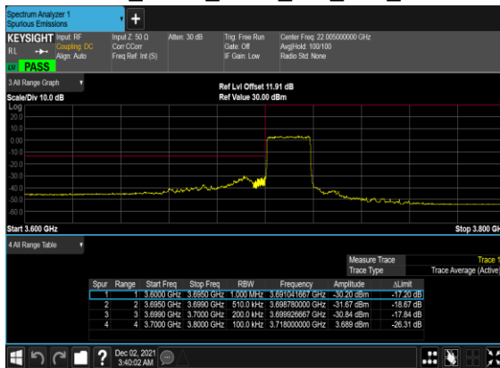
B41_N77(20M)_DFT-s-OFDM_BPSK_Outer_Full_Low_CH
