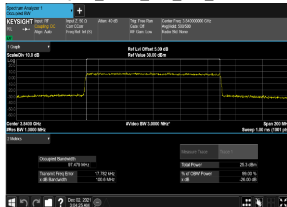
B41_N77(100M)_CP-OFDM_256 QAM_Outer_Full_Mid_CH
