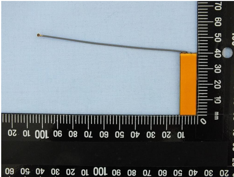
mFlexPIFA antenna
