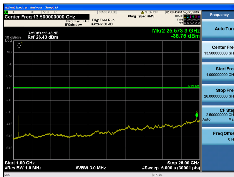
Band4-5MHz-QPSK-20375-1RB#0-1000~26000MHz
