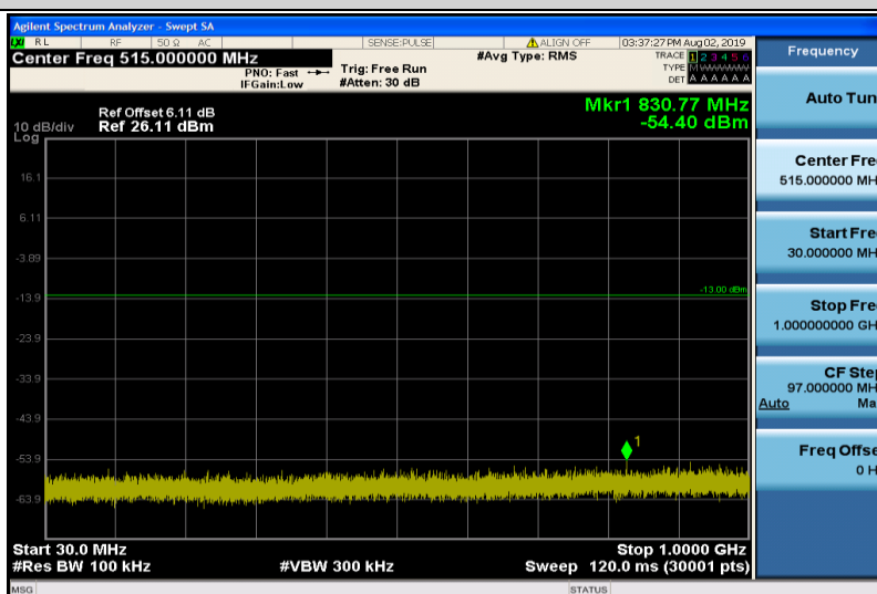
Band4-15MHz-QPSK-20175-1RB#0-30~1000MHz
