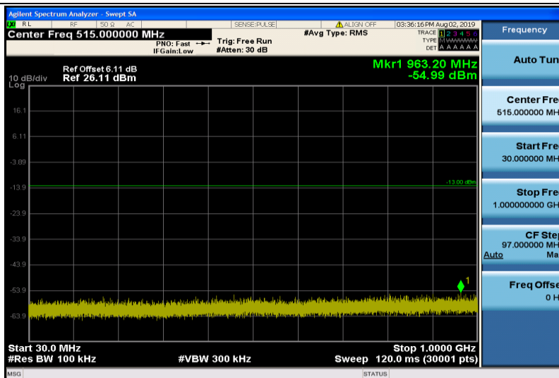
Band4-15MHz-QPSK-20025-1RB#0-30~1000MHz
