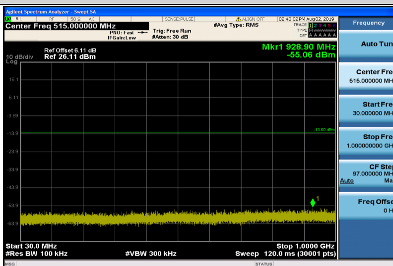
Band2-10MHz-16QAM-18900-1RB#0-30~1000MHz
