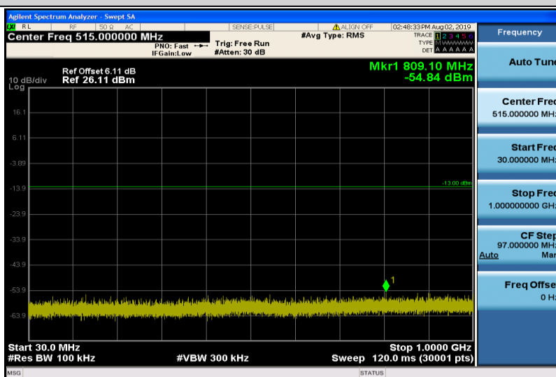
Band2-15MHz-QPSK-18900-1RB#0-30~1000MHz
