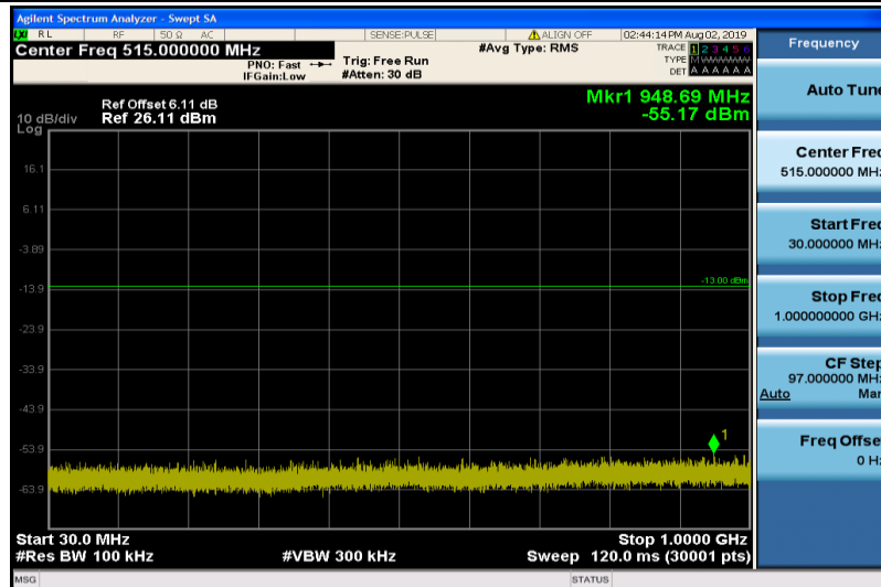
Band2-10MHz-16QAM-19150-1RB#0-30~1000MHz
