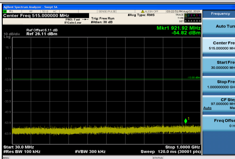
Band4-5MHz-QPSK-20175-1RB#0-30~1000MHz
