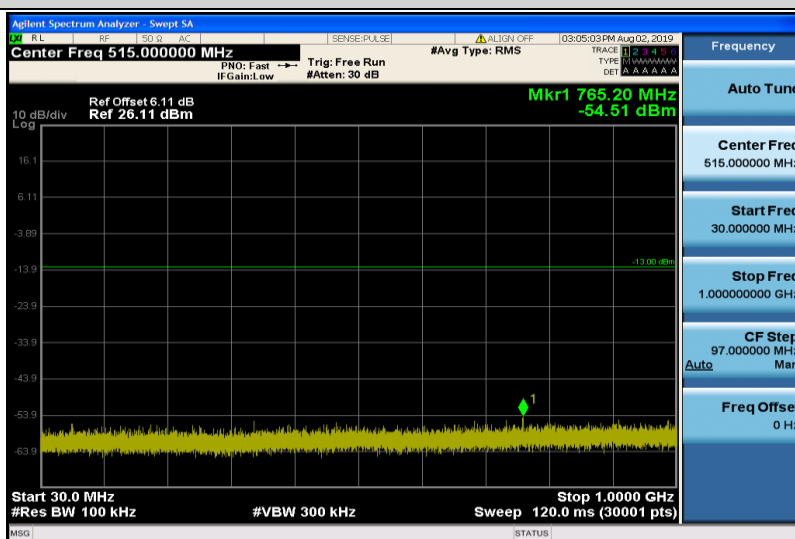
Band4-1.4MHz-16QAM-20175-1RB#0-30~1000MHz
