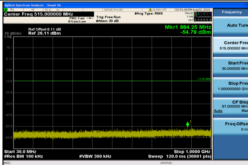
Band2-15MHz-QPSK-19125-1RB#0-30~1000MHz
