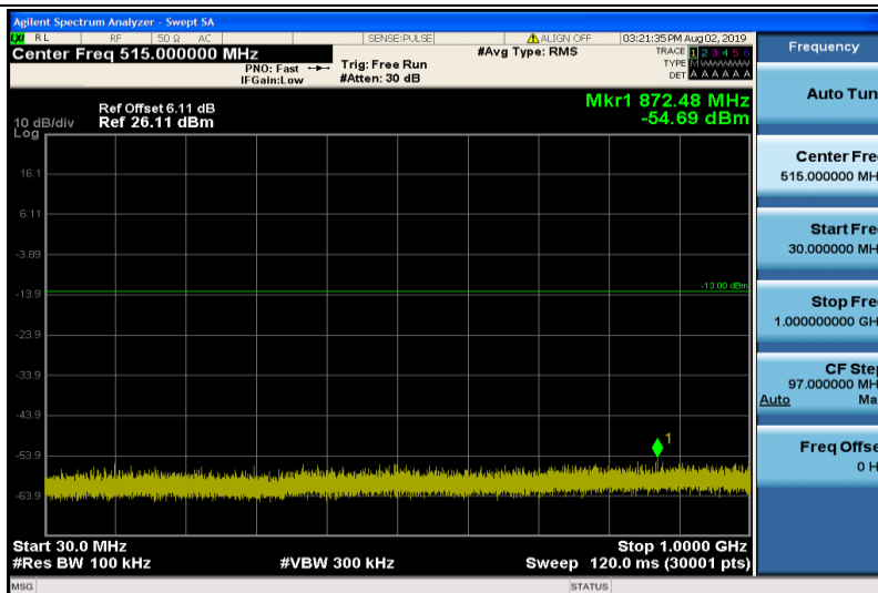
Band4-5MHz-QPSK-19975-1RB#0-30~1000MHz
