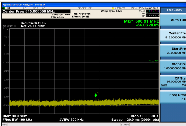
Band2-10MHz-16QAM-18650-1RB#0-30~1000MHz
