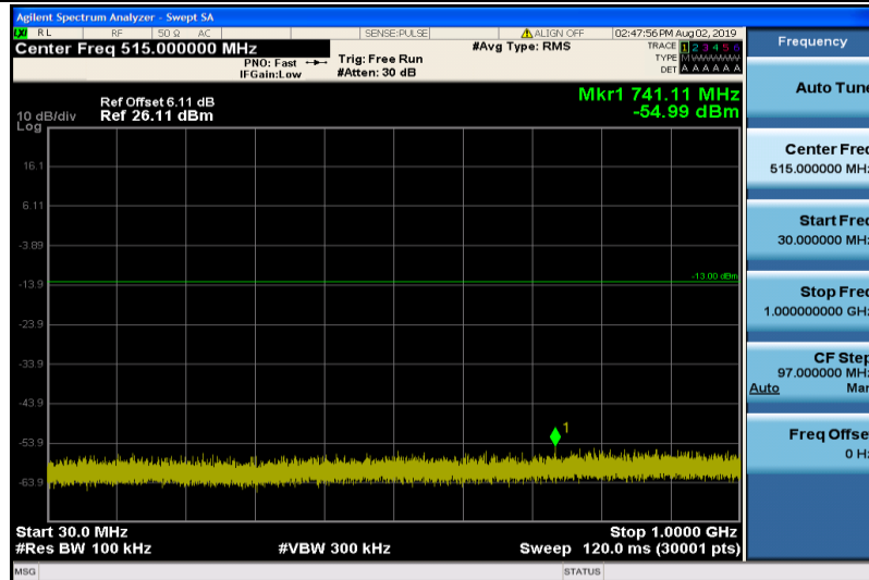
Band2-15MHz-16QAM-18675-1RB#0-30~1000MHz
