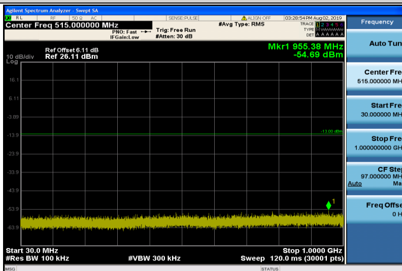
Band4-10MHz-QPSK-20175-1RB#0-30~1000MHz
