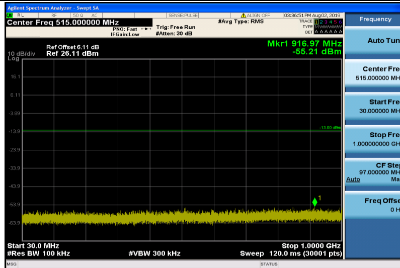
Band4-15MHz-16QAM-20025-1RB#0-30~1000MHz
