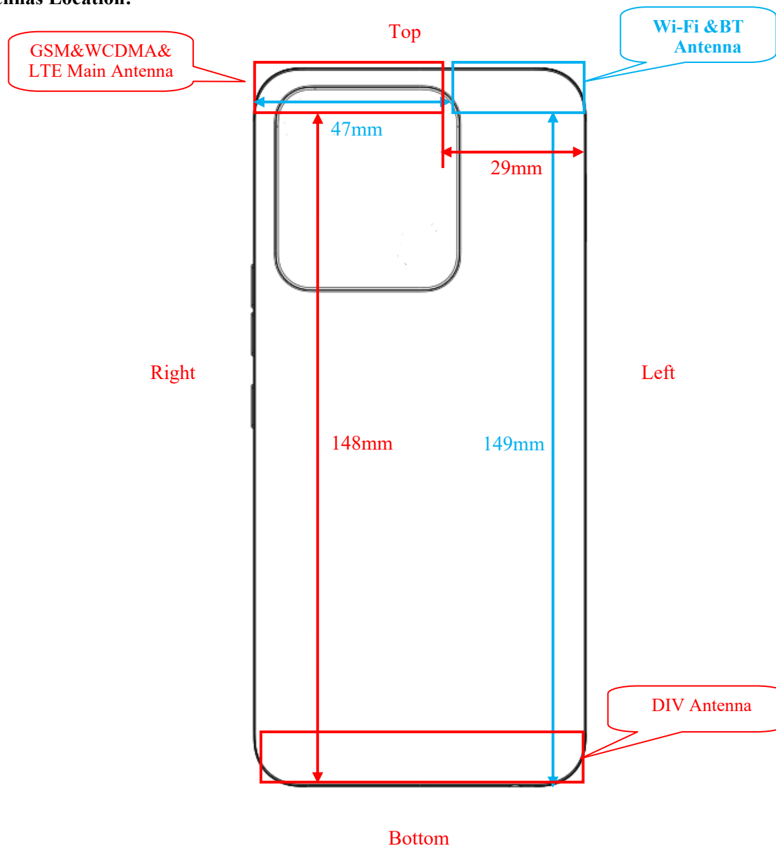
EUT Back View
