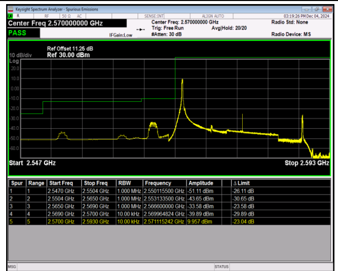
Band38-20MHz-QPSK-37850-100RB#0
