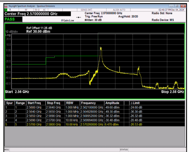
Band38-5MHz-16QAM-37775-25RB#0
