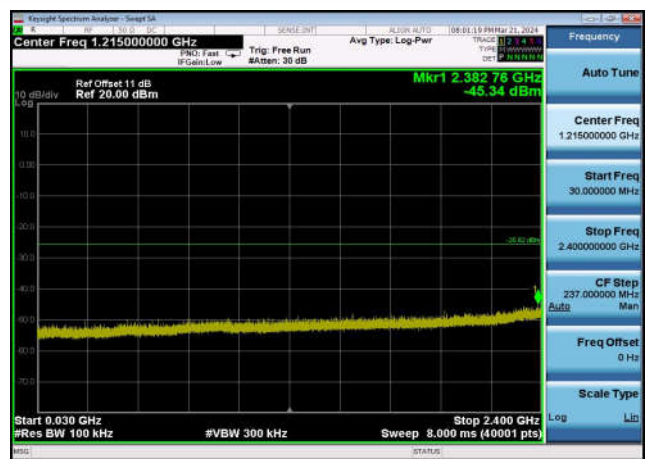
,Plot 3,30MHz~2400MHz-802.11g,2462MHz ,Ant1
