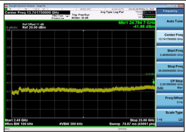
,Plot 4,2483.5MHz~25000MHz-802.11n(40 MHz),2437MHz,Ant1
