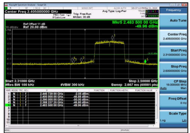
,Plot 2,Band Edge-802.11ax(40MHz) ,2452MHz,Ant1
