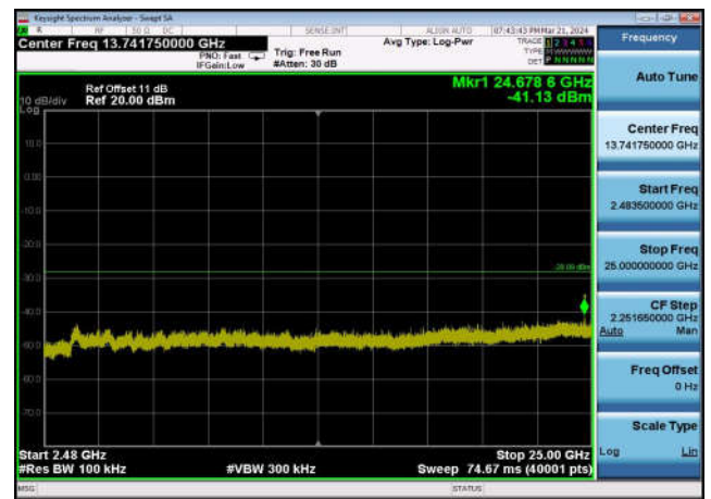
,Plot 4,2483.5MHz~25000MHz-802.11n(20 MHz),2462MHz,Ant1
