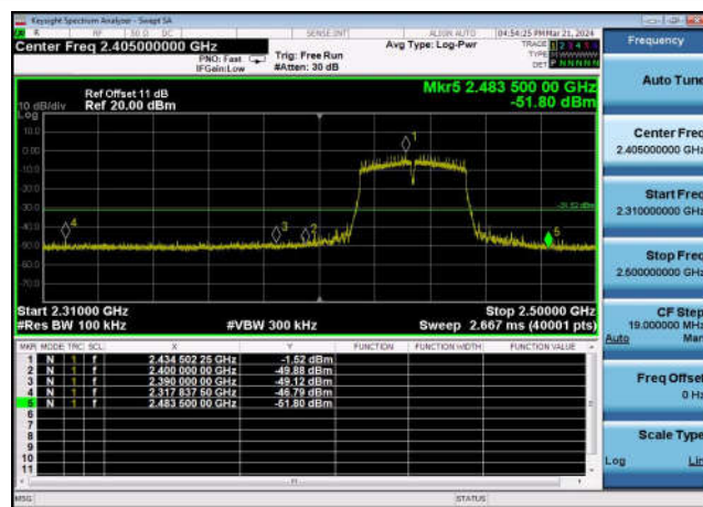
,Plot 2,Band Edge-802.11n(40MHz) ,2452MHz,Ant1
