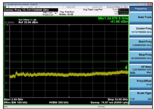
,Plot 4,2483.5MHz~25000MHz-802.11n(40 MHz),2452MHz,Ant1
