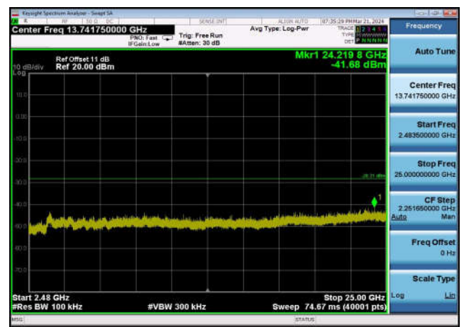
,Plot 4,2483.5MHz~25000MHz-802.11n(20 MHz),2437MHz,Ant1
