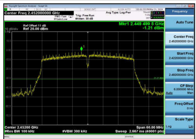
,Plot 2,Band Edge-802.11n(40MHz) ) ,2422MHz,Ant1
