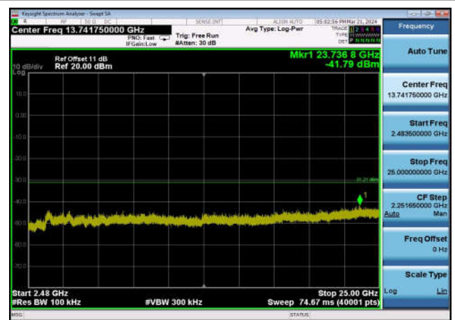
,Plot 1,Reference Level-802.11ax(20MHz),2412MHz,Ant1
