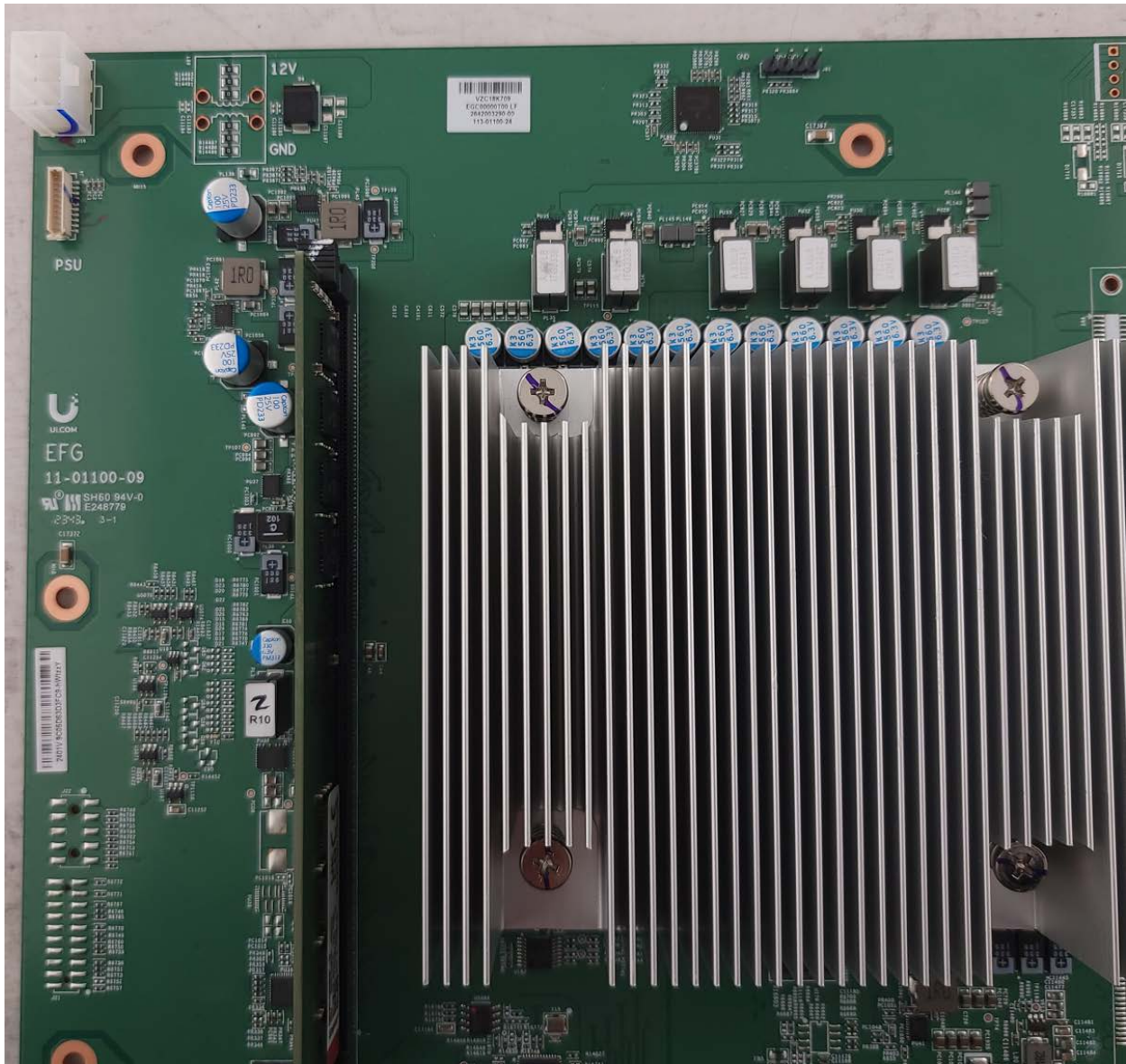
Photograph 1: Top Main PCB Close-up Back/Left
