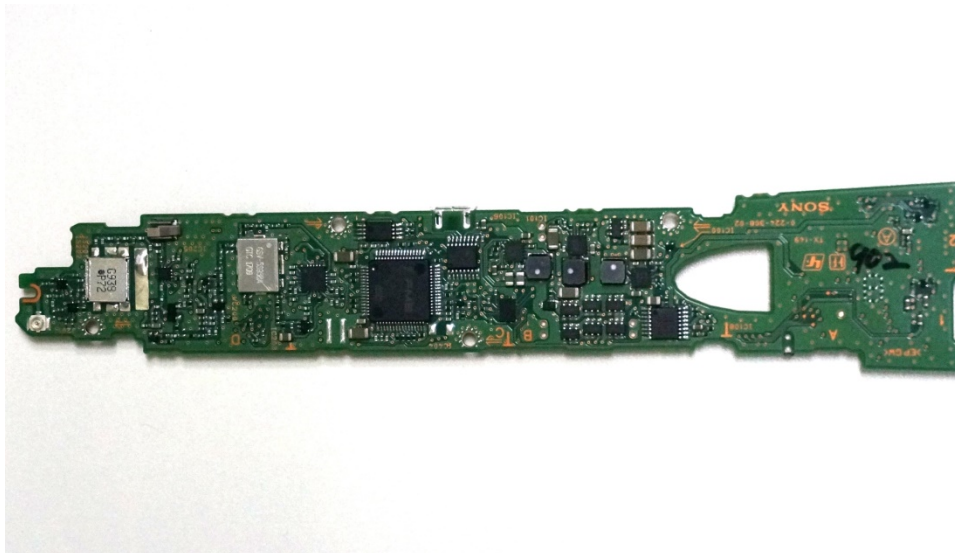
Fig.5: Side A of board TX-149
