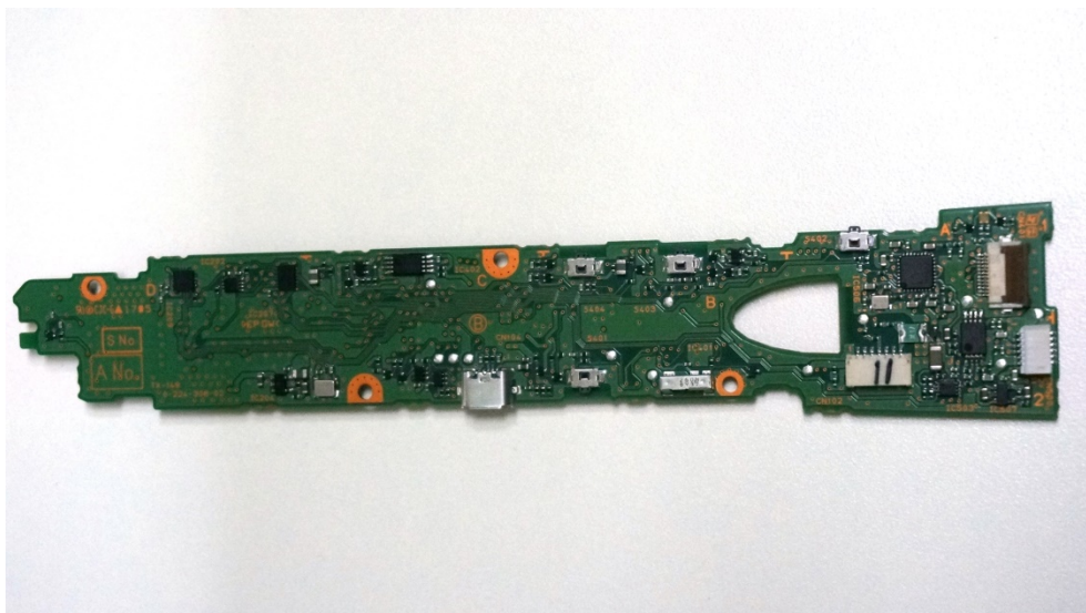
Fig.6: Side B of board TX-149
