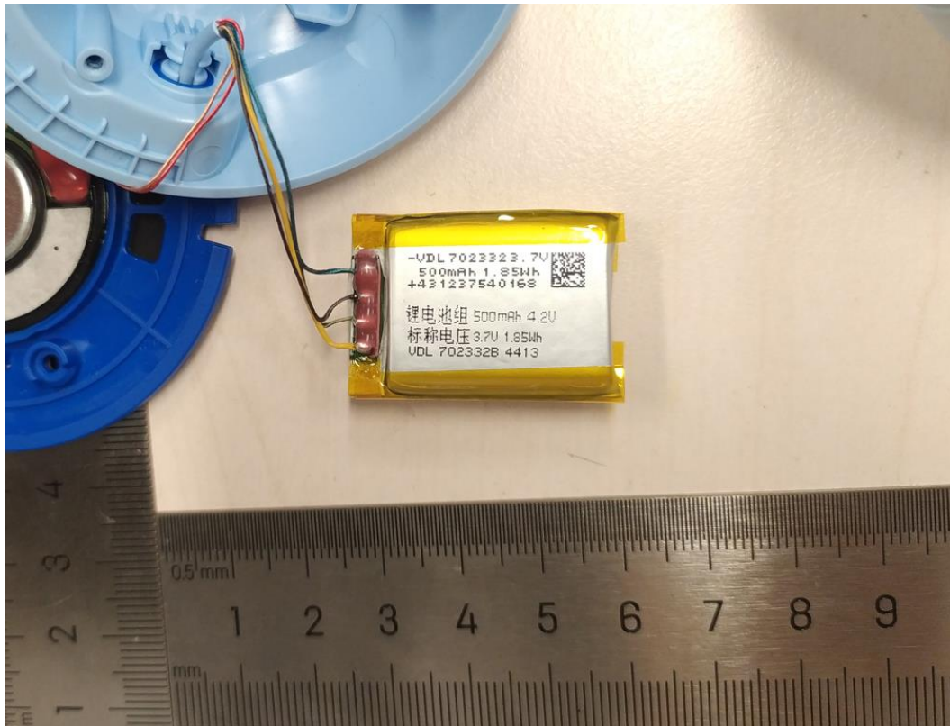
Fig.5. Battery pack view -1
