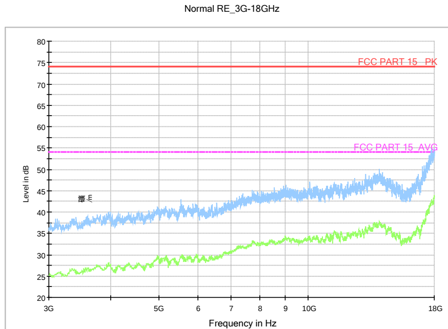
Fig.22. Radiated emission: GFSK, 2440MHz, 3 GHz - 18 GHz
