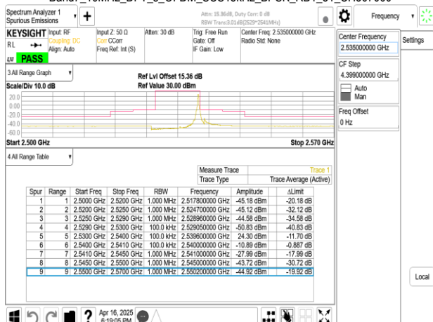
Band7_10MHz_DFT_s_OFDM_SCS15kHz_BPSK_RB1_51_CH507000
