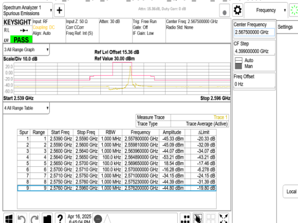
Band7_5MHz_CP_OFDM_SCS15kHz_QPSK_RB1_24_CH513500
