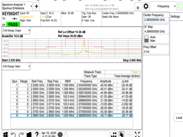
Band7_10MHz_CP_OFDM_SCS15kHz_QPSK_RB1_51.CH513000
