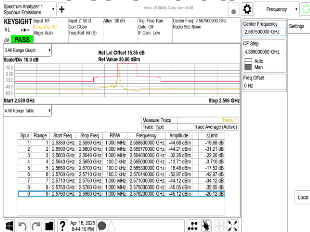
Band7_5MHz_CP_OFDM_SCS15kHz_QPSK_RB1_24_CH513500
