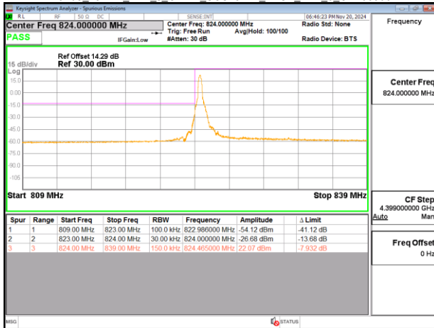
Band5_15MHz_CP_OFDM_SCS15kHz_BPSK_RB75_0_CH166300
