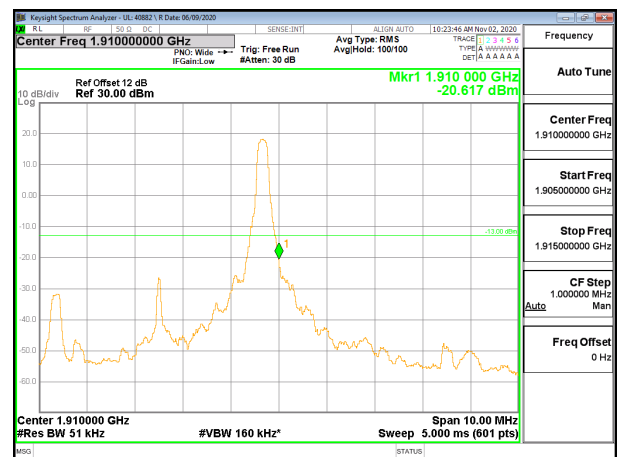
LTE B2 5MHz QPSK High Channel RB1-24
