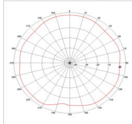
Far-field Power Distribution(H+V) on X-Z Plane Plot Peak Gain(H+V)= 2.67 dB, Plot AvgGain(H+V)= 0.53dB @2.45000 GHz
