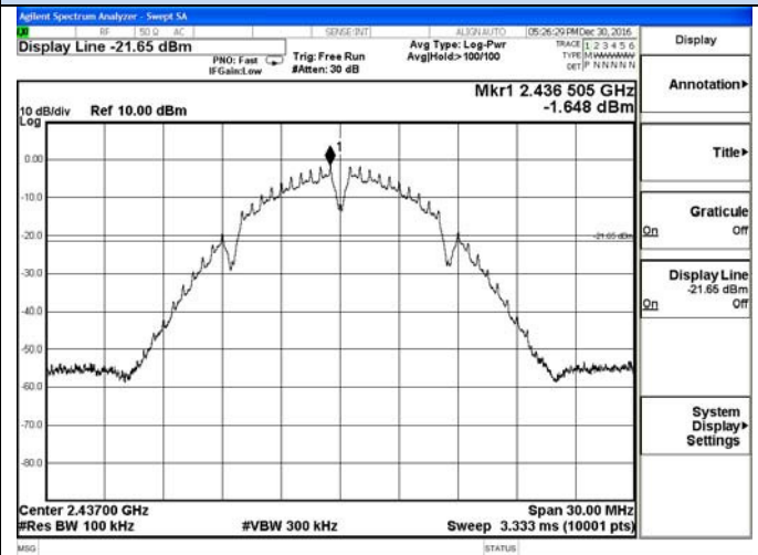
802.11b_Middle Channel
