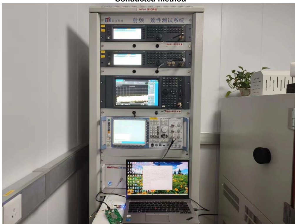
Conducted method
