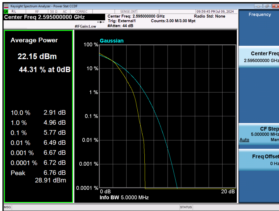
LTE Band 38 / 5 MHz / 16QAM / FULL RB Size
