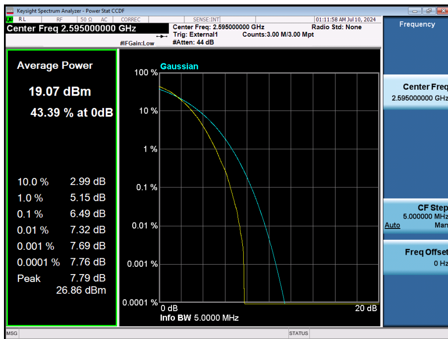
LTE Band 38 / 5 MHz / 256QAM / FULL RB Size
