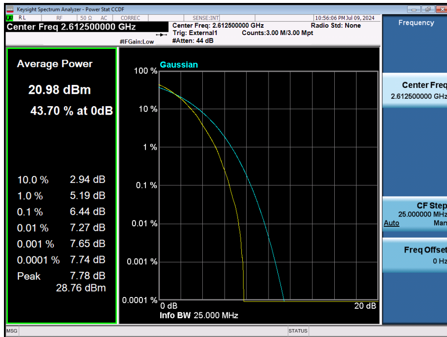
LTE Band 38 / 15 MHz / 64QAM / FULL RB Size
