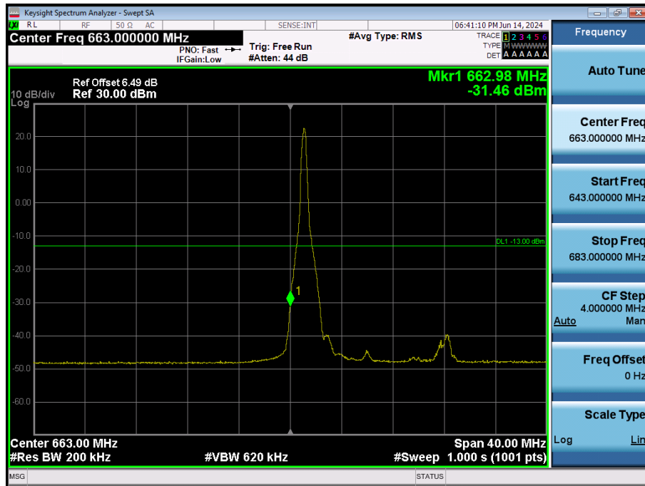
LTE Band 71 / 20MHz / QPSK - RB Size/Offset (1/0)
