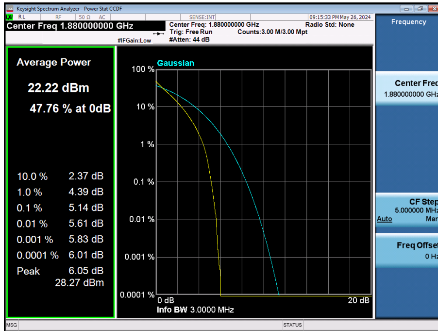
LTE Band 2 / 3 MHz / QPSK / FULL RB Size
