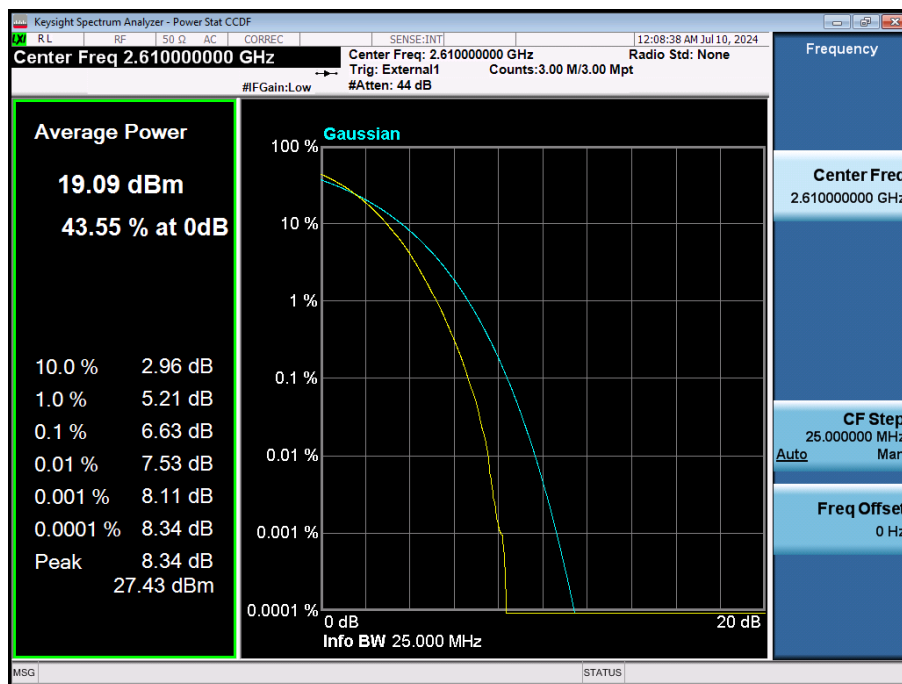
LTE Band 38 / 20 MHz / 256QAM / FULL RB Size
