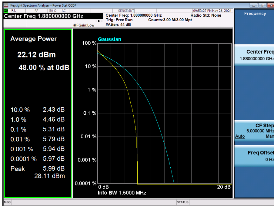
LTE Band 2 / 1.4 MHz / QPSK / FULL RB Size
