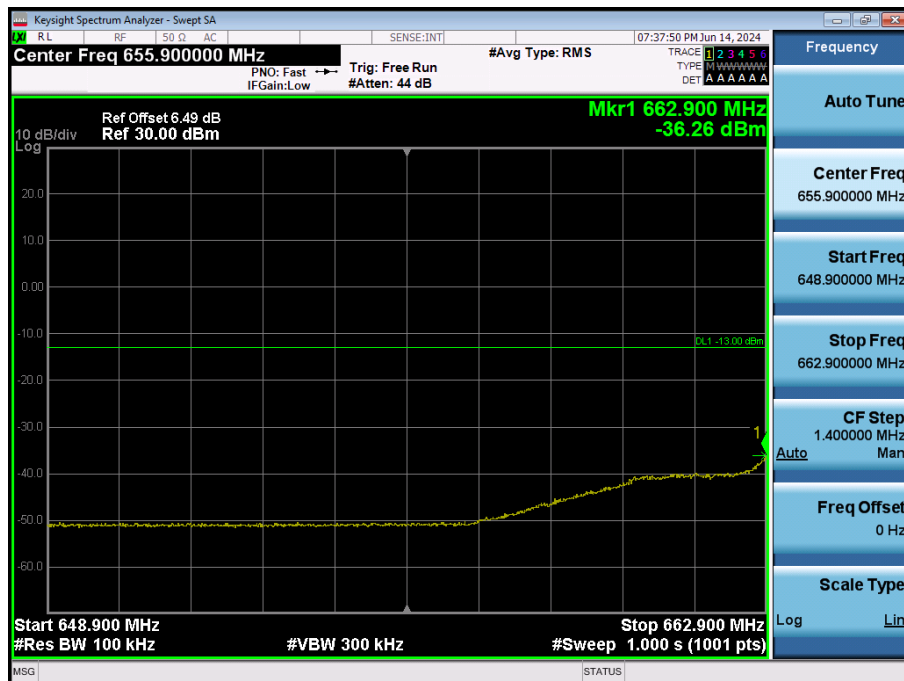
LTE Band 71 / 15MHz / QPSK - RB Size/Offset (36/0)
