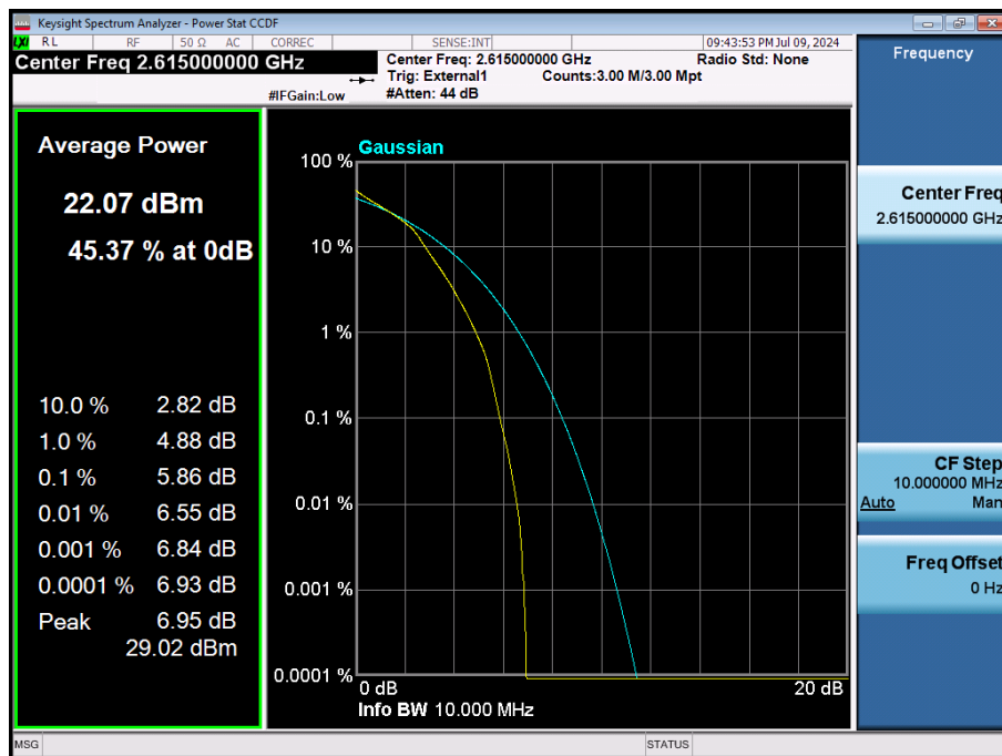
LTE Band 38 / 10 MHz / 16QAM / FULL RB Size
