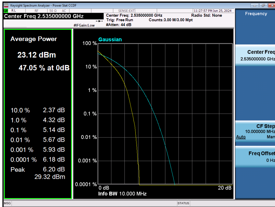
LTE Band 7 / 10 MHz / QPSK / FULL RB Size
