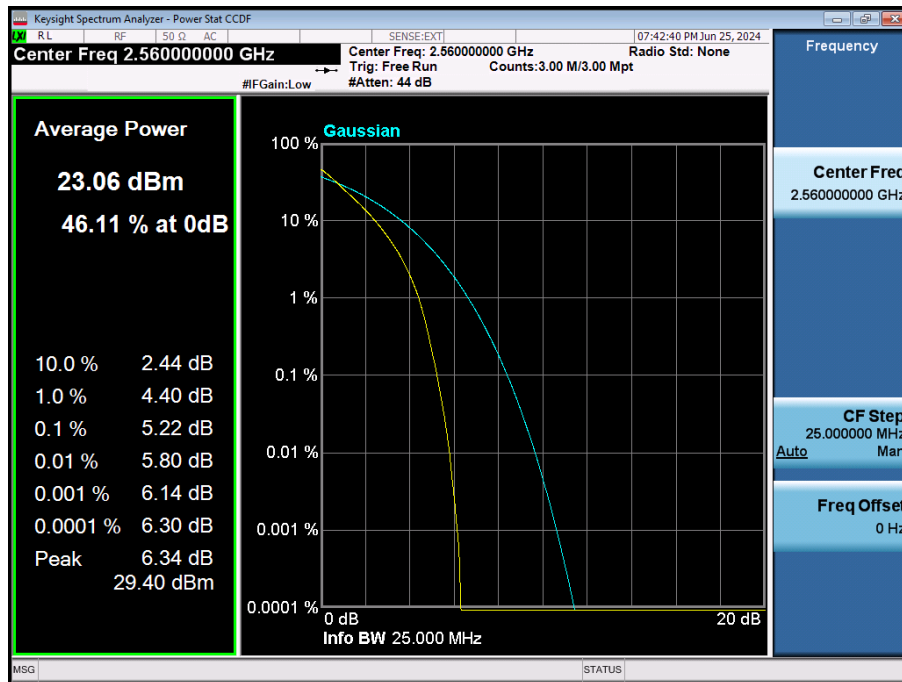
LTE Band 7 / 20 MHz / QPSK / FULL RB Size
