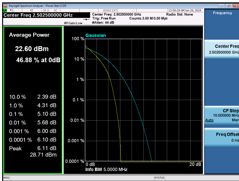
LTE Band 7 / 5 MHz / QPSK / FULL RB Size
