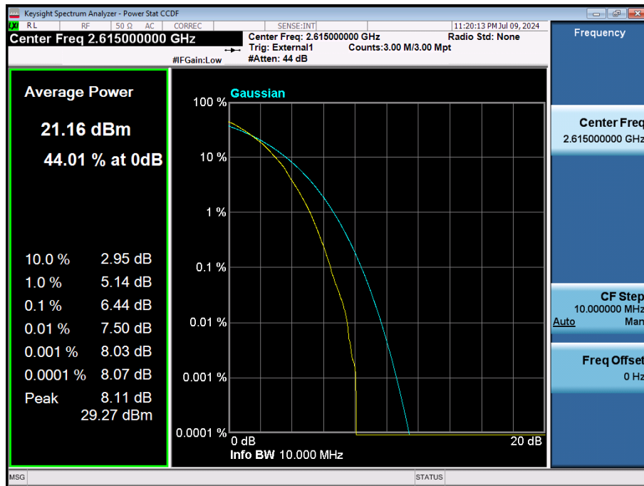
LTE Band 38 / 10 MHz / 64QAM / FULL RB Size
