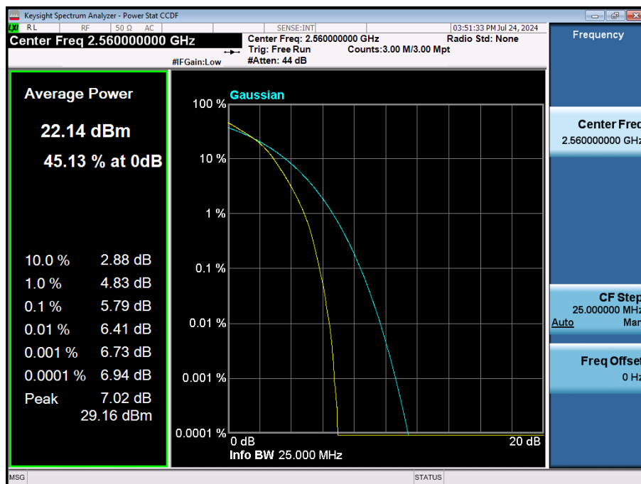
LTE Band 7 / 20 MHz / 16QAM / FULL RB Size
