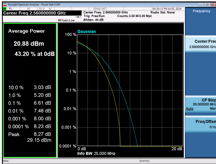
LTE Band 7 / 20 MHz / 64QAM / FULL RB Size
