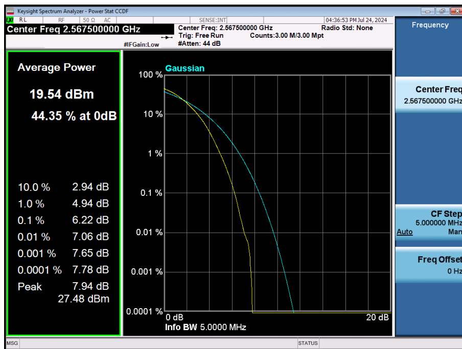
LTE Band 7 / 5 MHz / 256QAM / FULL RB Size
