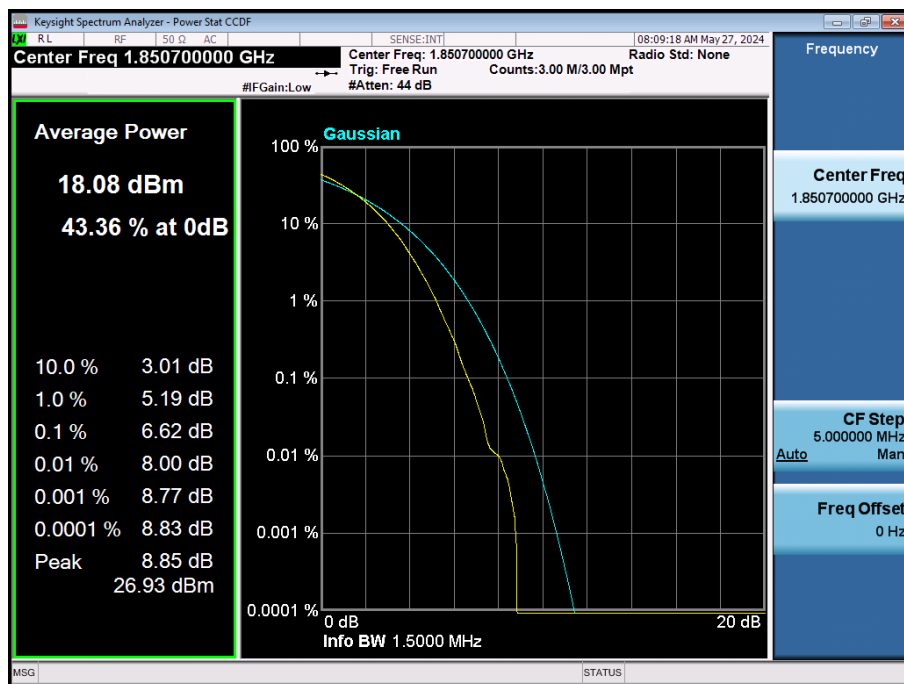
LTE Band 2 / 1.4 MHz / 256QAM / FULL RB Size
