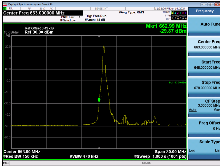
LTE Band 71 / 15MHz / 16QAM - RB Size/Offset (1/0)
