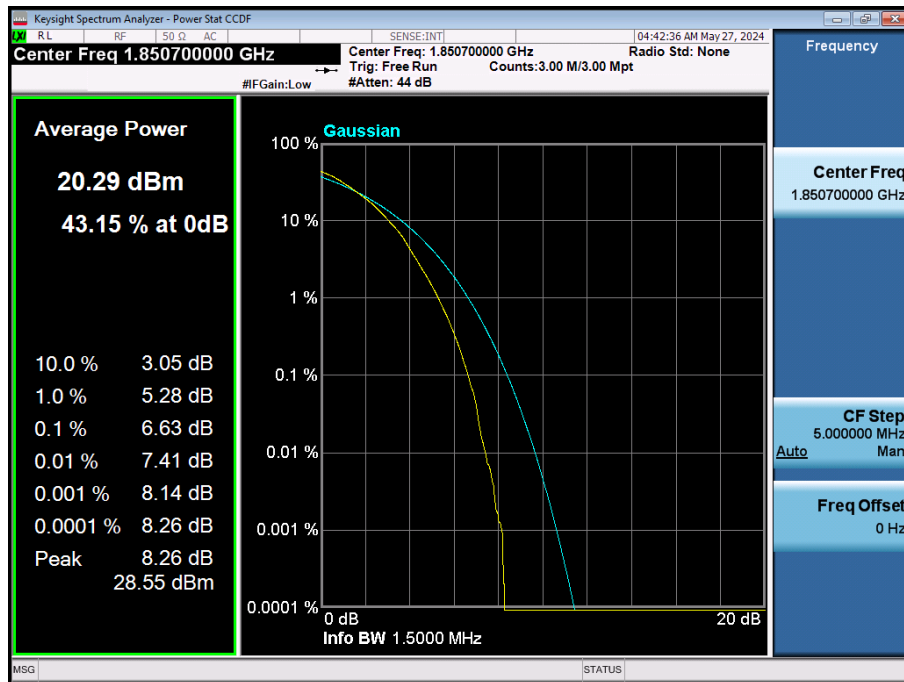
LTE Band 2 / 1.4 MHz / 64QAM / FULL RB Size
