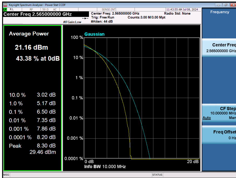
LTE Band 7 / 10 MHz / 64QAM / FULL RB Size
