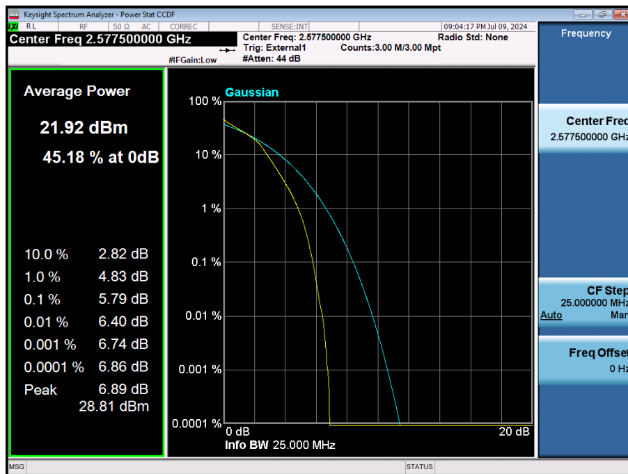
LTE Band 38 / 15 MHz / 16QAM / FULL RB Size
