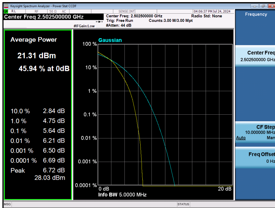
LTE Band 7 / 5 MHz / 16QAM / FULL RB Size
