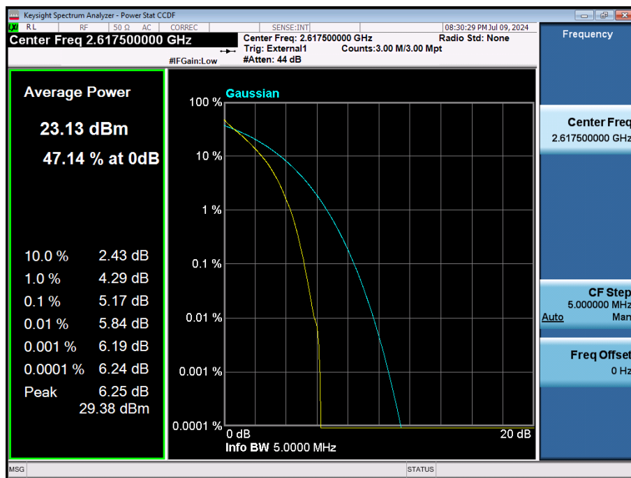
LTE Band 38 / 5 MHz / QPSK / FULL RB Size
