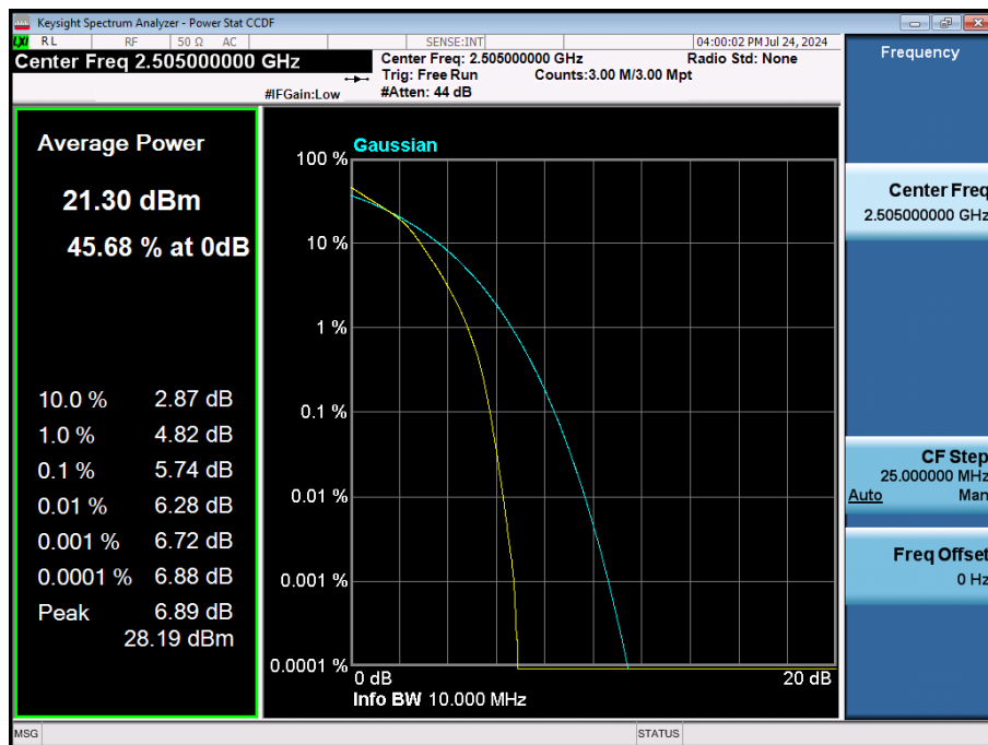
LTE Band 7 / 10 MHz / 16QAM / FULL RB Size
