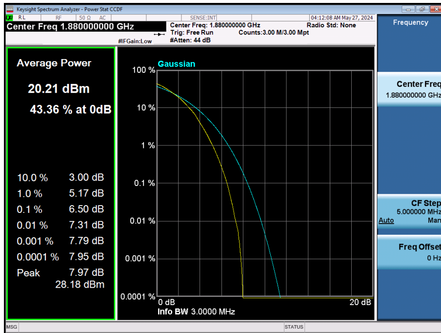
LTE Band 2 / 3 MHz / 64QAM / FULL RB Size
