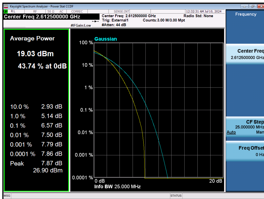
LTE Band 38 / 15 MHz / 256QAM / FULL RB Size
