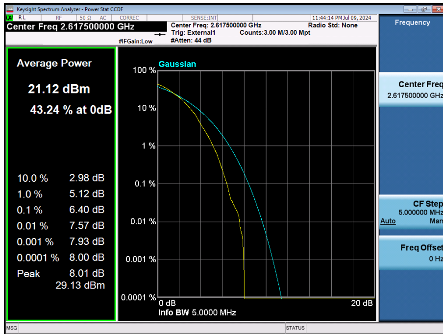
LTE Band 38 / 5 MHz / 64QAM / FULL RB Size
