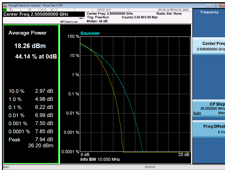
LTE Band 7 / 10 MHz / 256QAM / FULL RB Size
