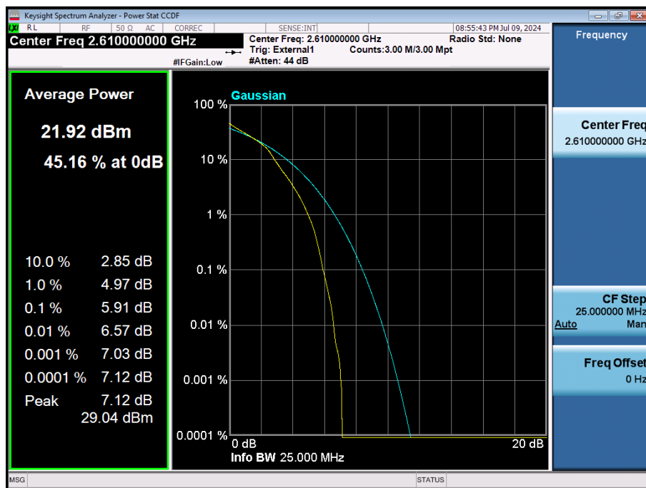
LTE Band 38 / 20 MHz / 16QAM / FULL RB Size
