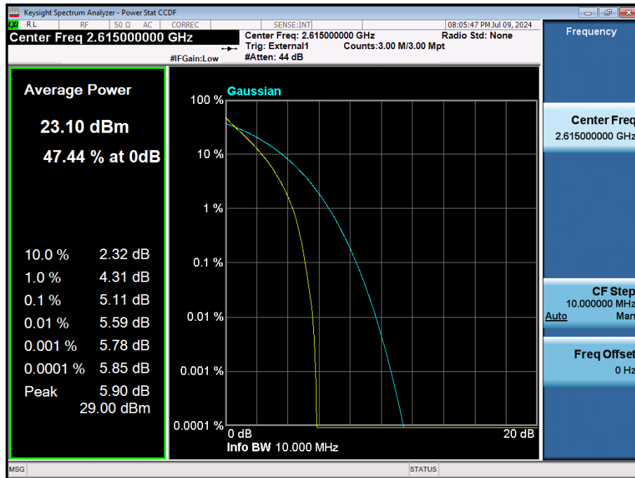
LTE Band 38 / 10 MHz / QPSK / FULL RB Size
