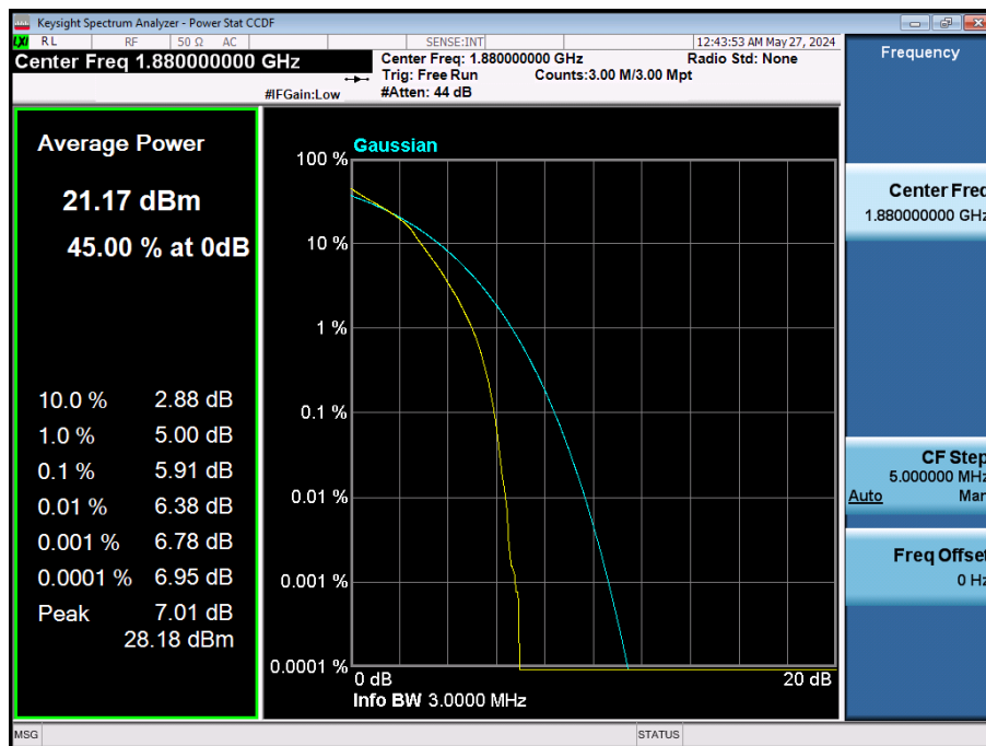
LTE Band 2 / 3 MHz / 16QAM / FULL RB Size
