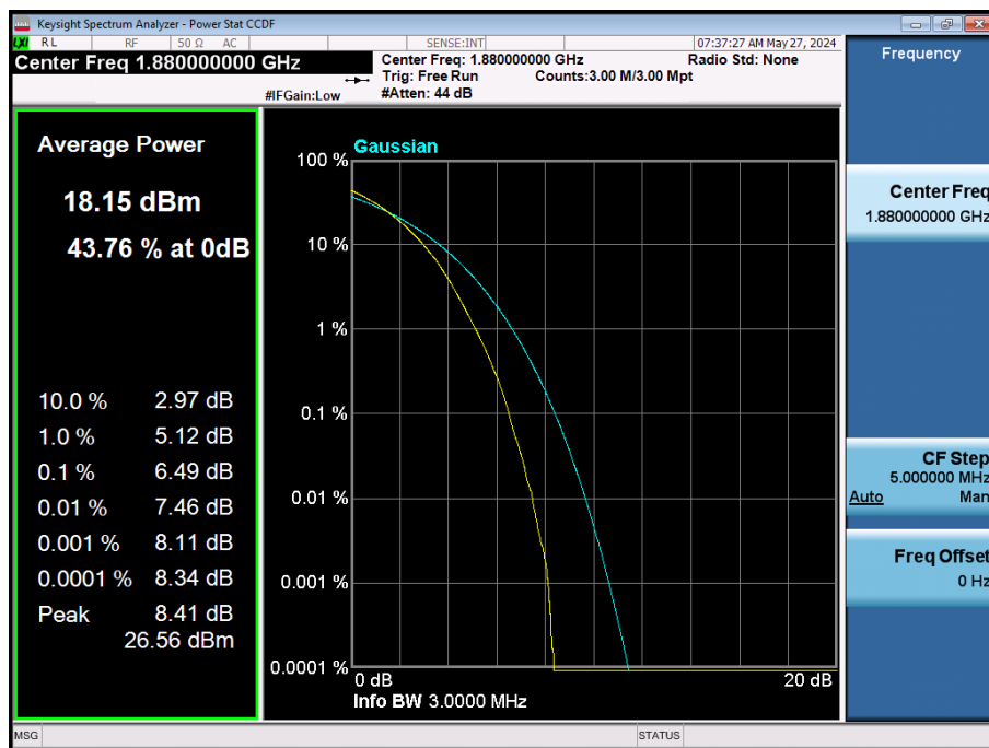
LTE Band 2 / 3 MHz / 256QAM / FULL RB Size
