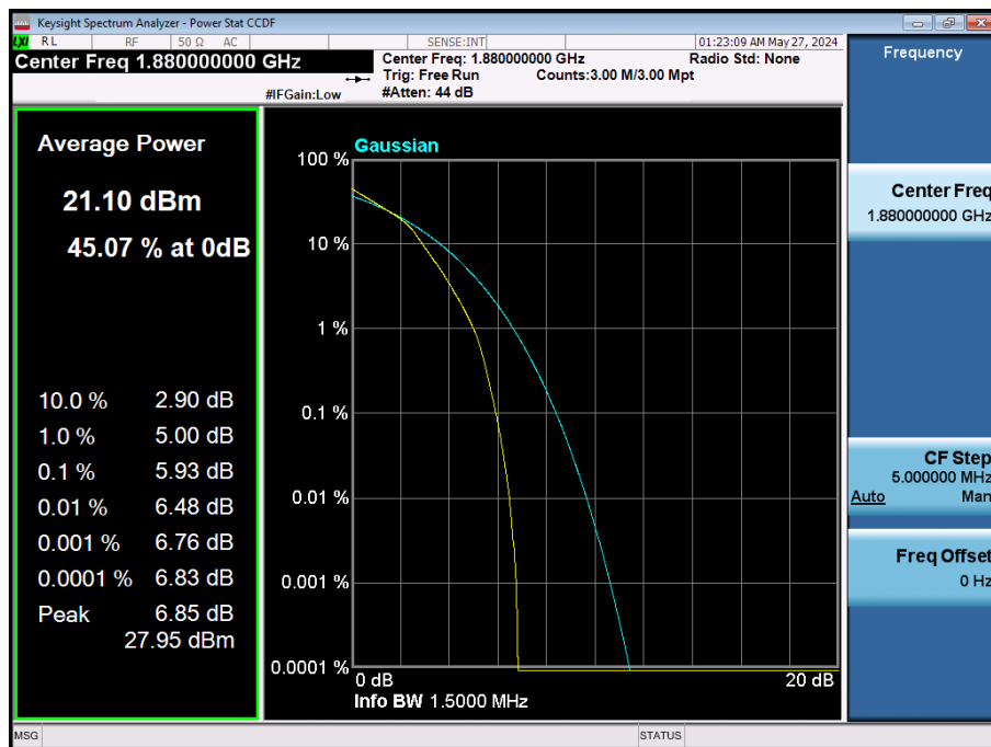
LTE Band 2 / 1.4 MHz / 16QAM / FULL RB Size
