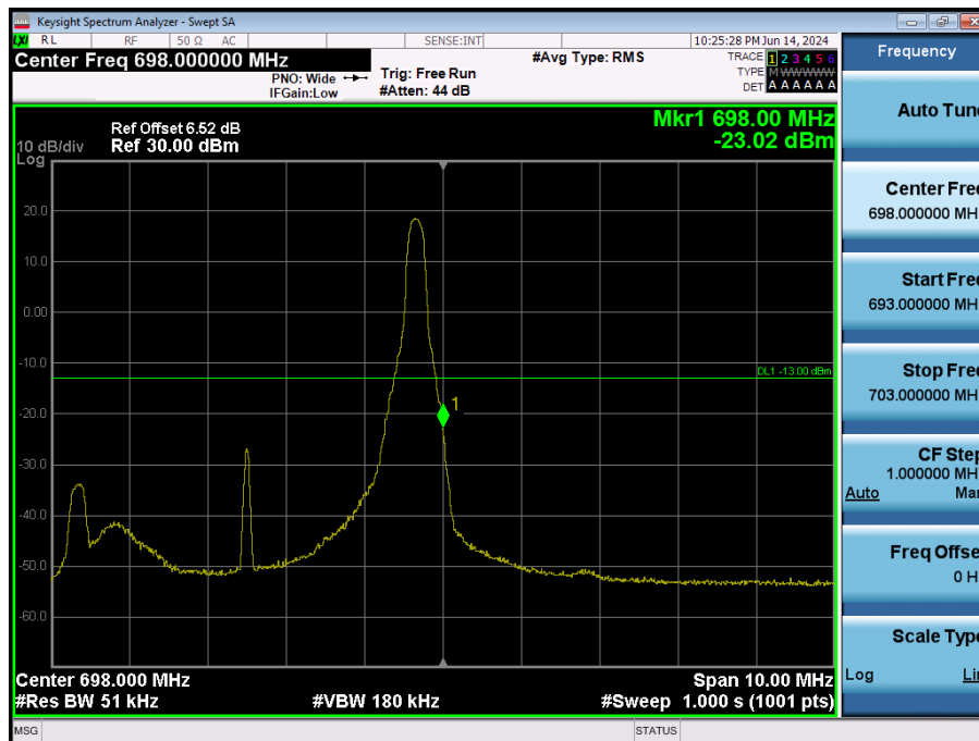
LTE Band 71 / 5MHz / QPSK - RB Size/Offset (1/24)
