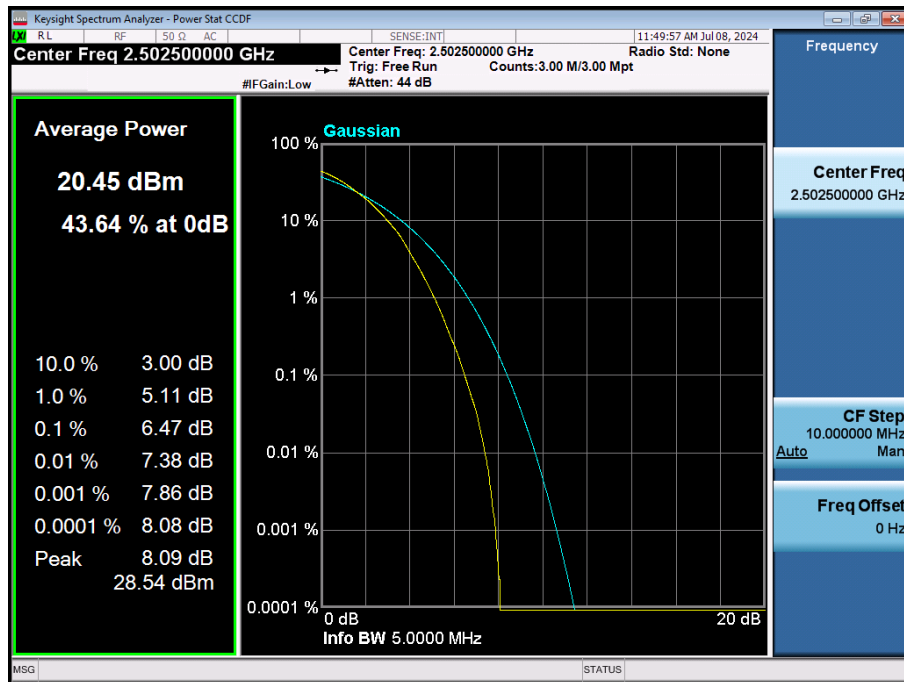
LTE Band 7 / 5 MHz / 64QAM / FULL RB Size
