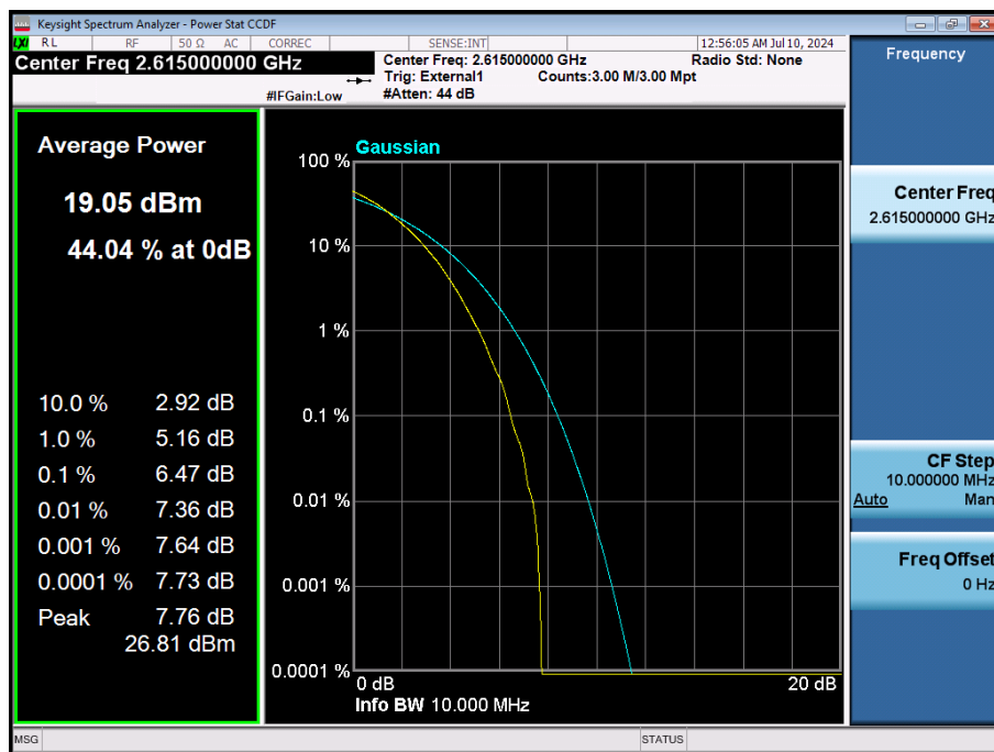
LTE Band 38 / 10 MHz / 256QAM / FULL RB Size
