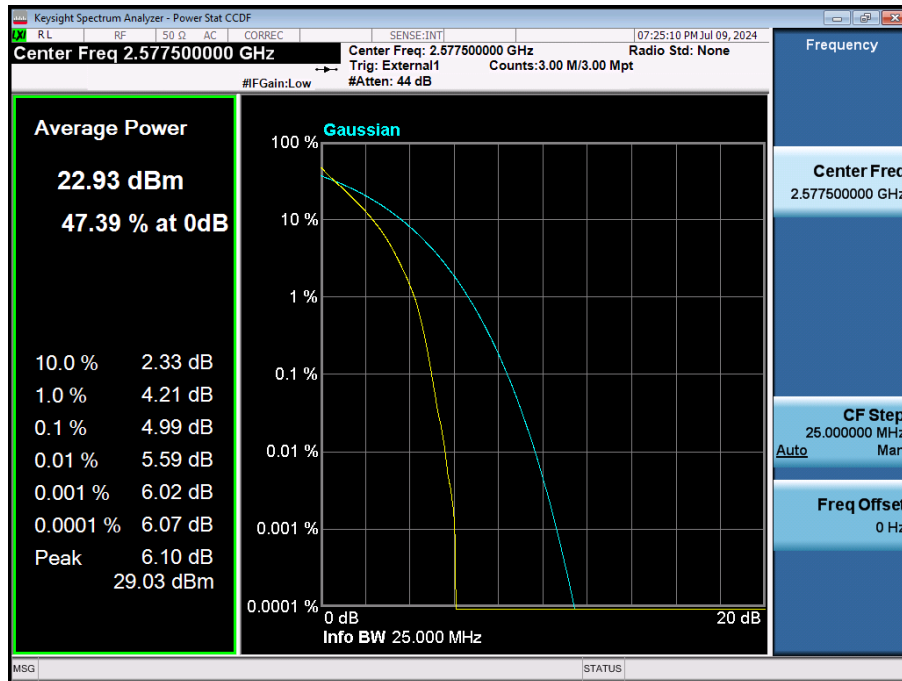
LTE Band 38 / 15 MHz / QPSK / FULL RB Size
