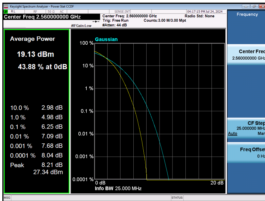
LTE Band 7 / 20 MHz / 256QAM / FULL RB Size
