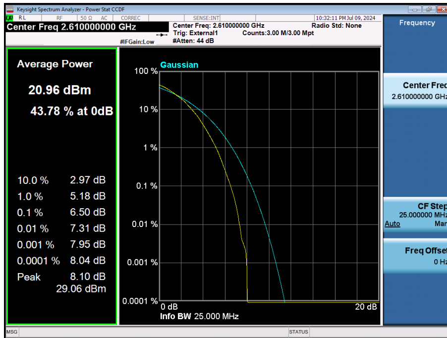
LTE Band 38 / 20 MHz / 64QAM / FULL RB Size
