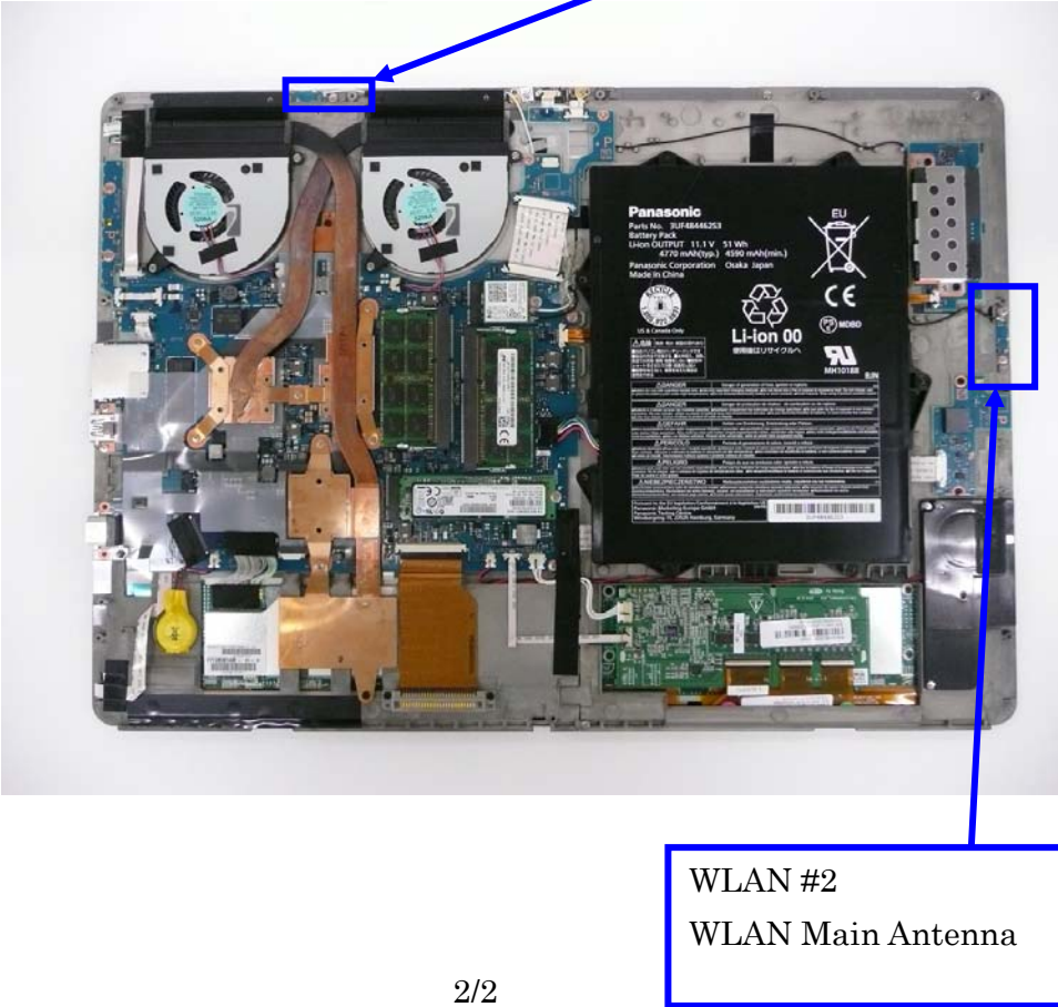
Back side view (back cover removed)
