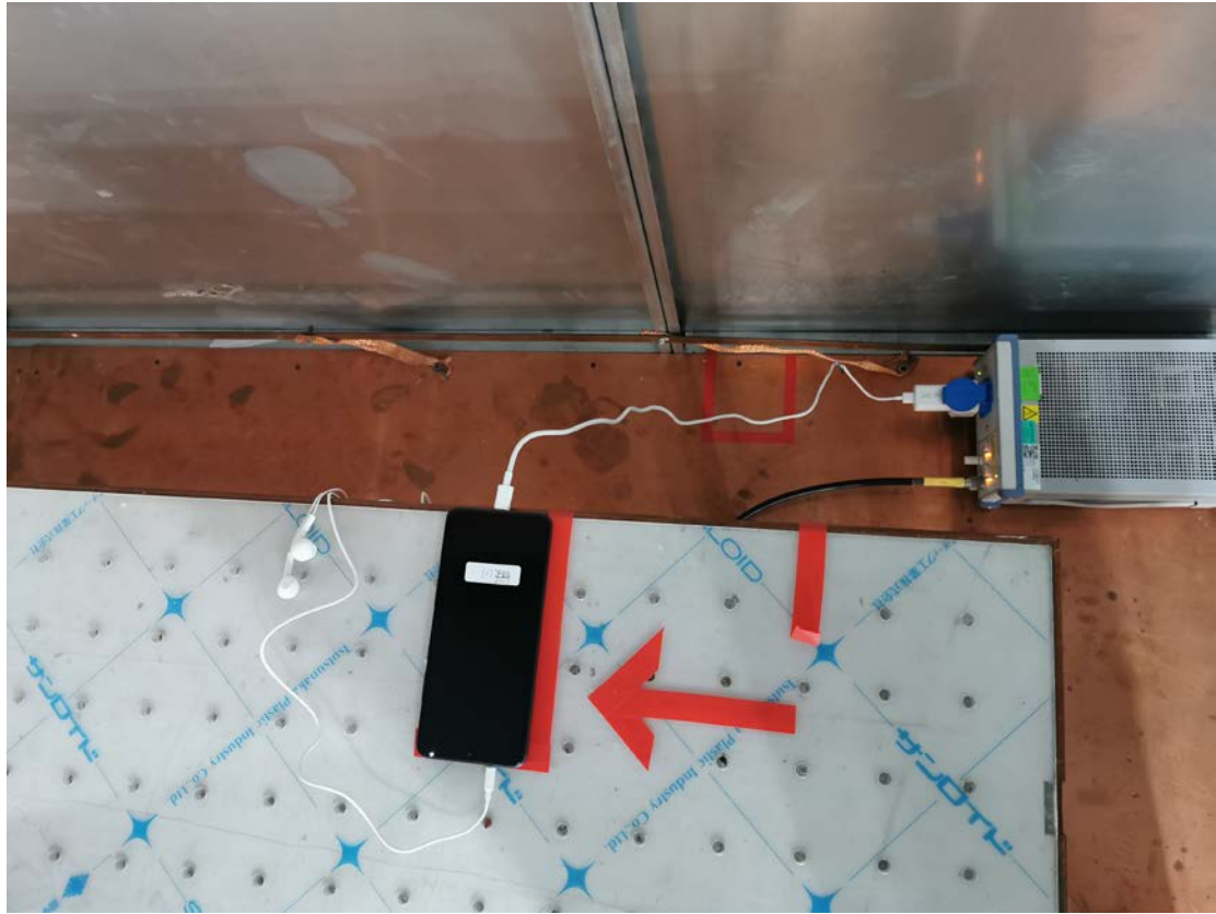
Conducted Emissions Test Setup (with charger)
