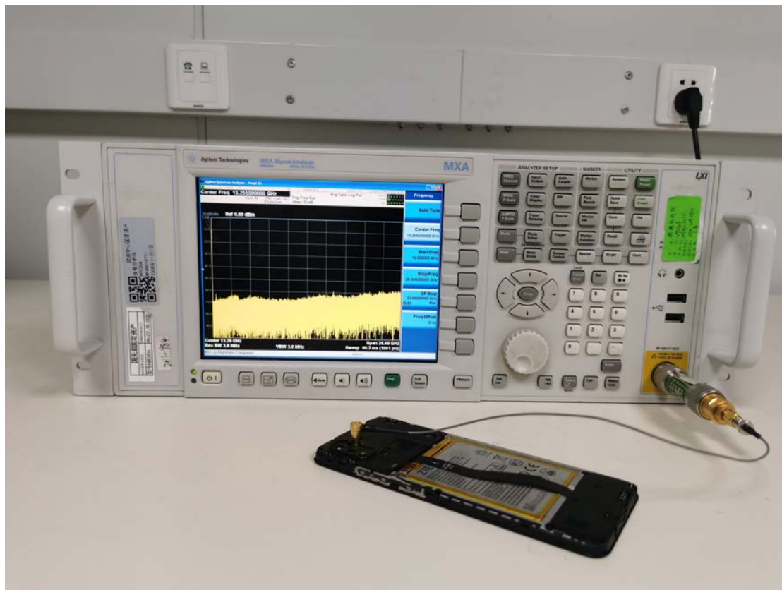
RF Conducted Test setup (BT/BLE/WIFI)
