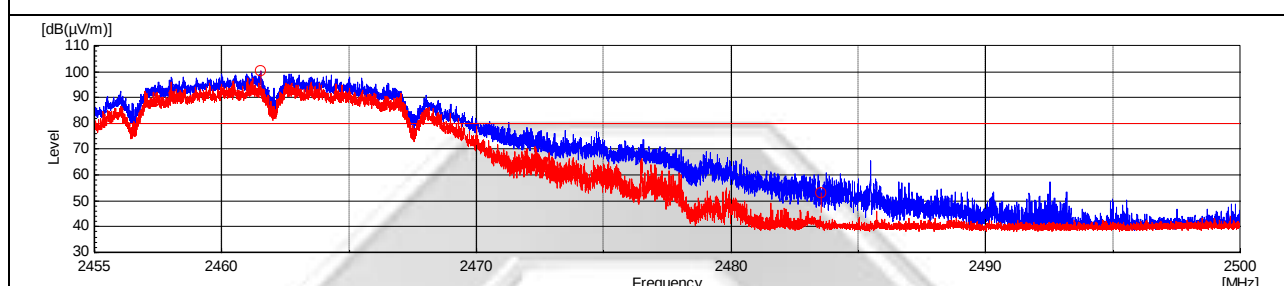
Plot 2 – Upper Band Edge at 2.4835GHz
