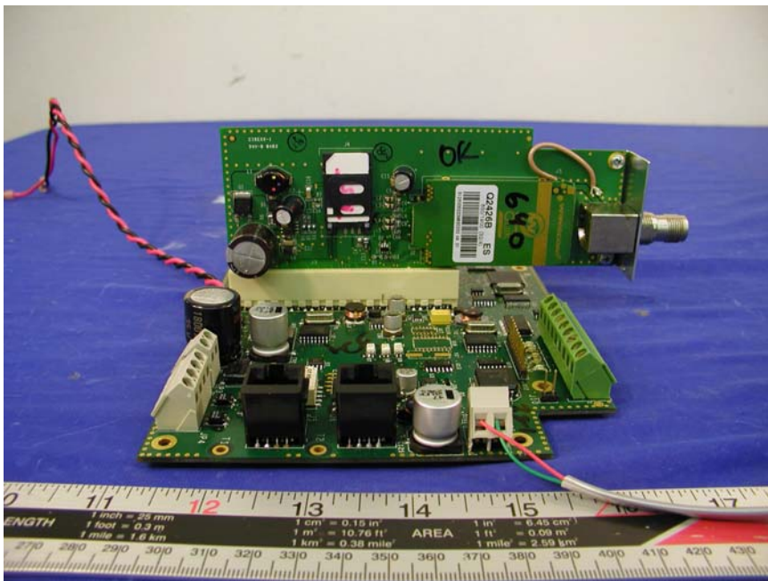
EUT - Main Board Side View
