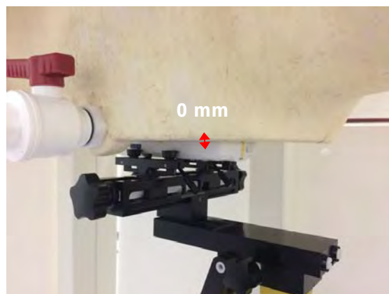
Fig.10 EUT Front side to flat phantom
