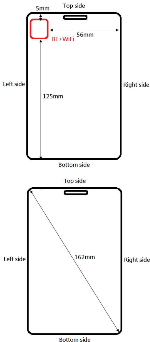
Fig.15 Antenna location and dimensional size
