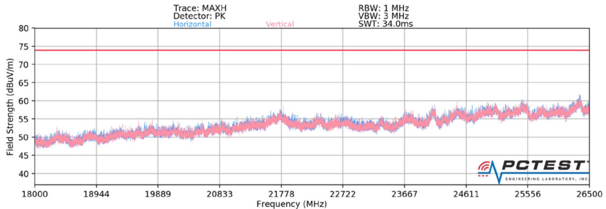
Plot 7-72. Radiated Spurious Plot above 18GHz CDD
