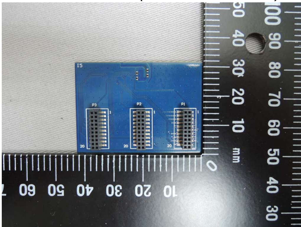
Back View of Antenna-3 (Part No.: DFAM-NW726-DT0R)
