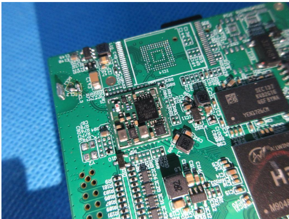
Photo 8 (Model:ah3.zw8us.4G/EG91)
