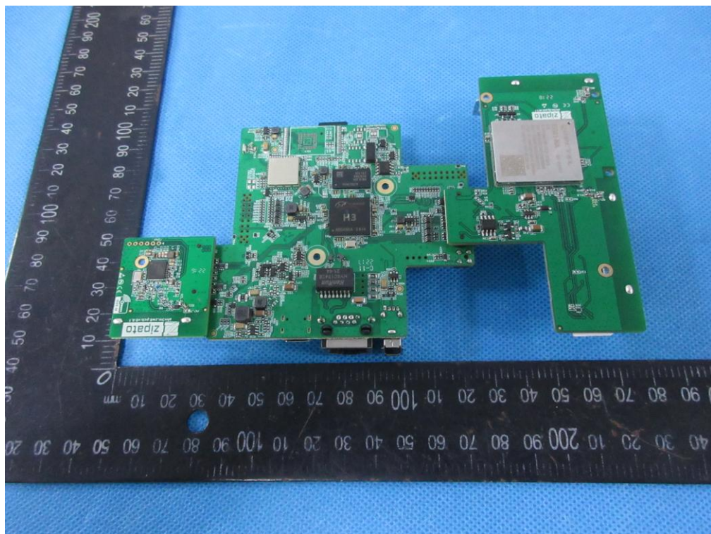
Photo 4 (Model:ah3.zw8us.4G/EG91)
