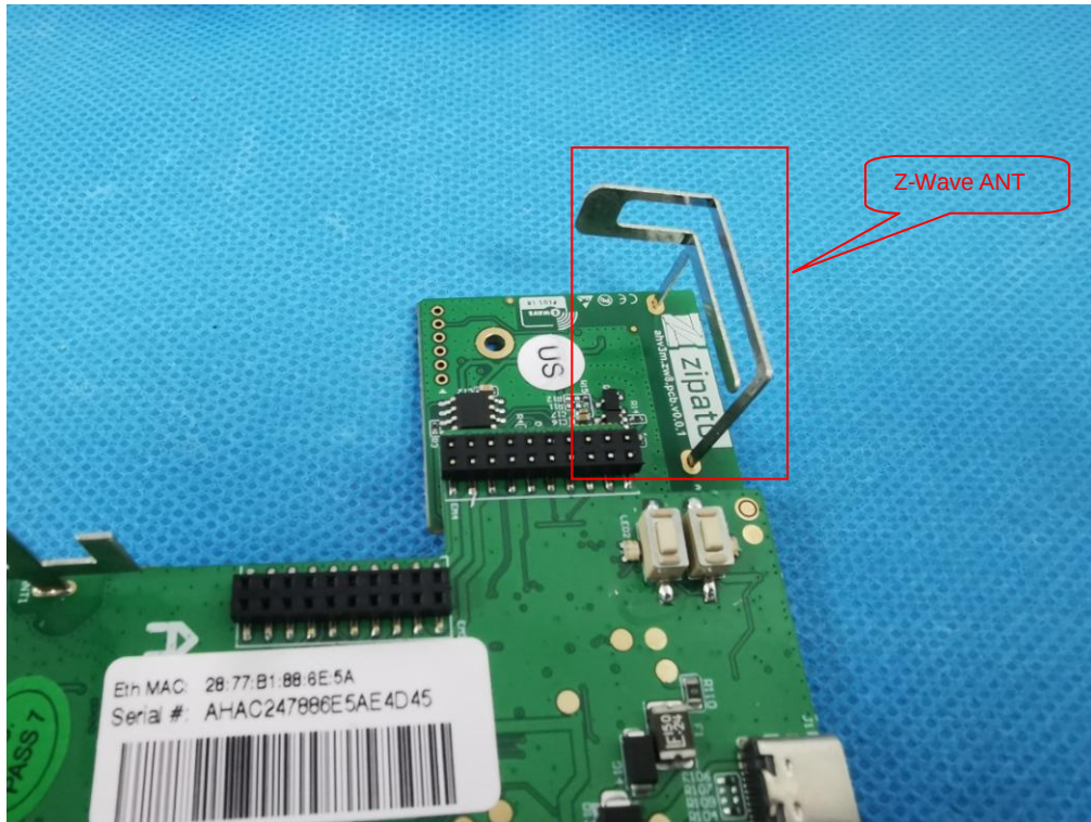
Photo 11 (Model:ah3.zw8us.4G/EG91)
