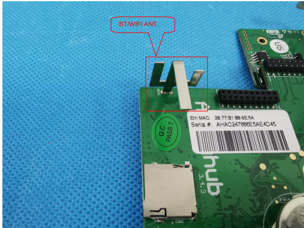
Photo 13 (Model:ah3.zw8us.4G/EG91)
