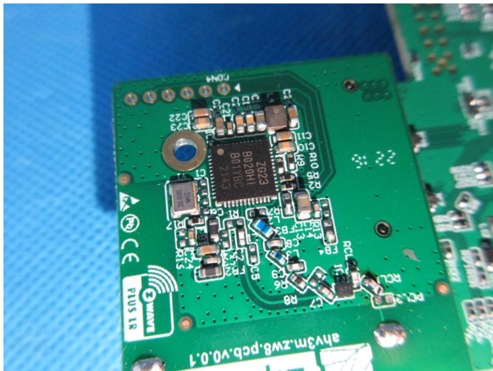
Photo 6 (Model:ah3.zw8us.4G/EG91)
