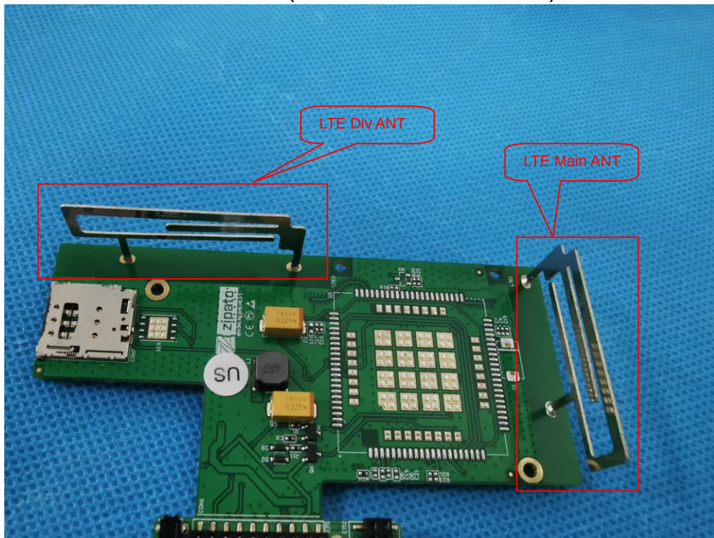
Photo 12 (Model:ah3.zw8us.4G/EG91)
